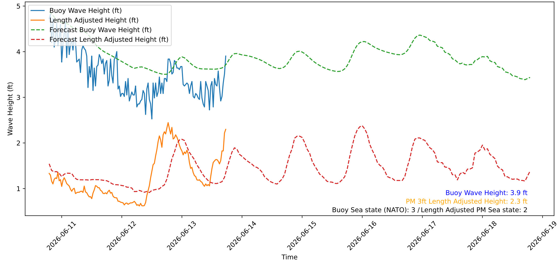
Wave Heights over Time for Red Beach at 2026-06-13 18:30:47
