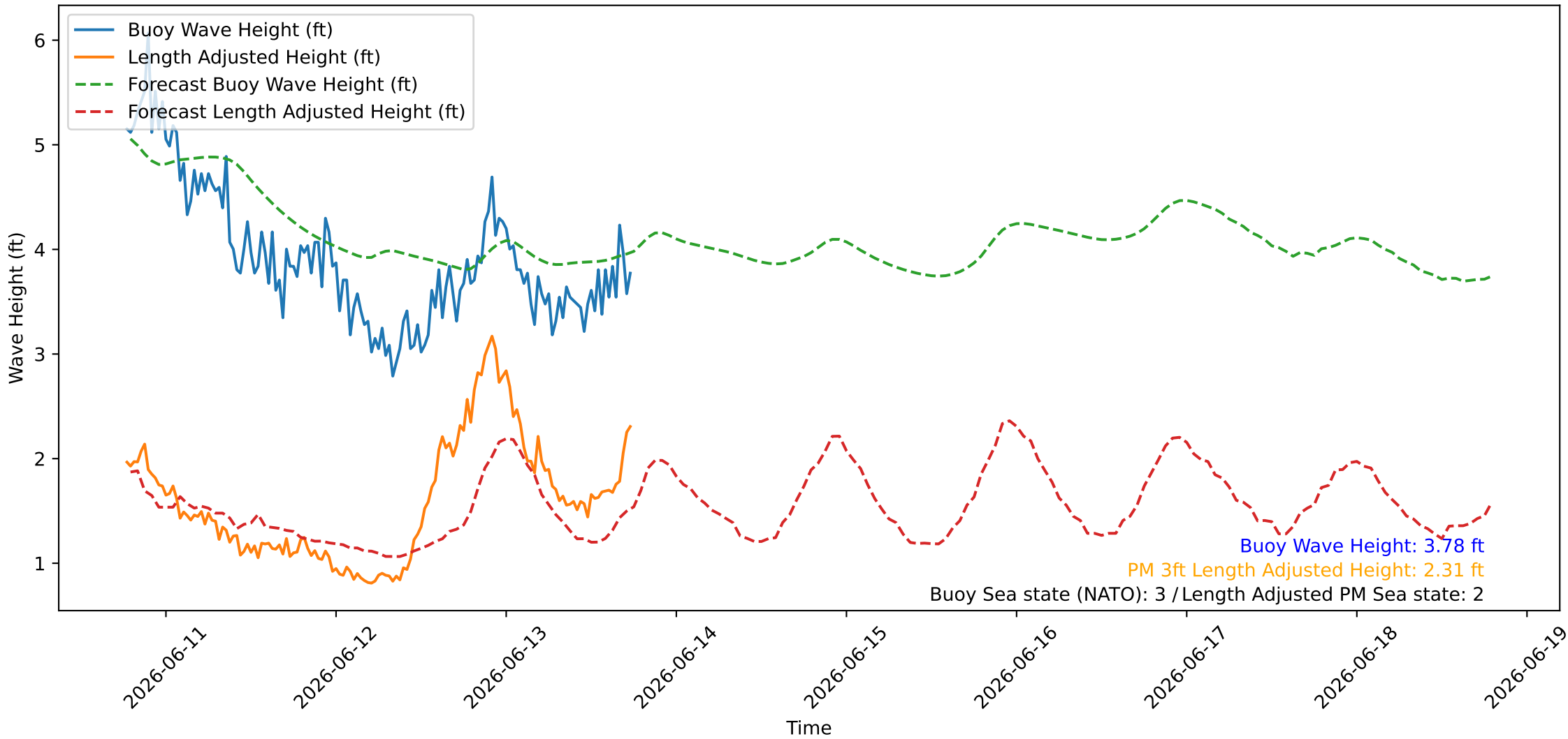
Wave Heights over Time for Oceanside Harbor at 2026-06-13 18:30:27
