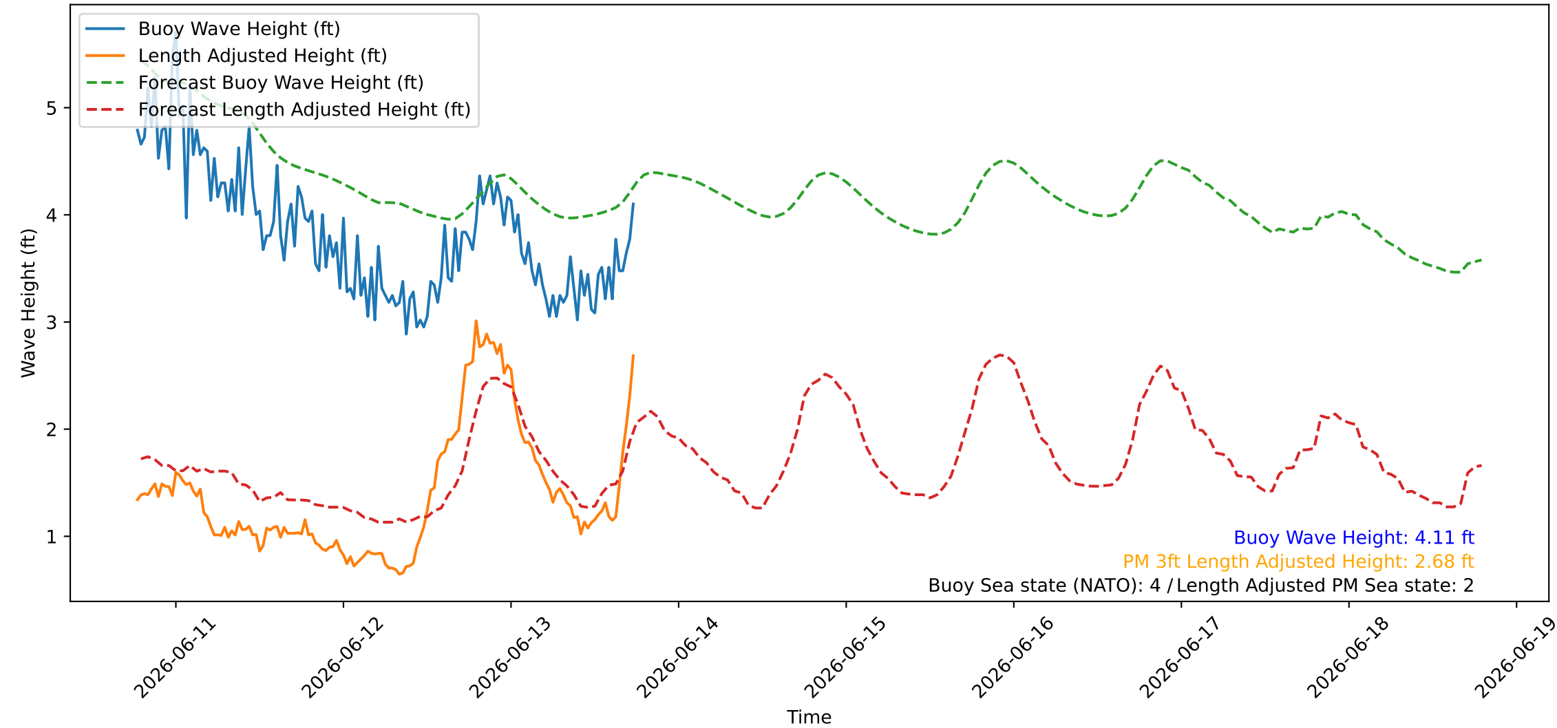
Wave Heights over Time for Green Beach at 2026-06-13 18:31:09
