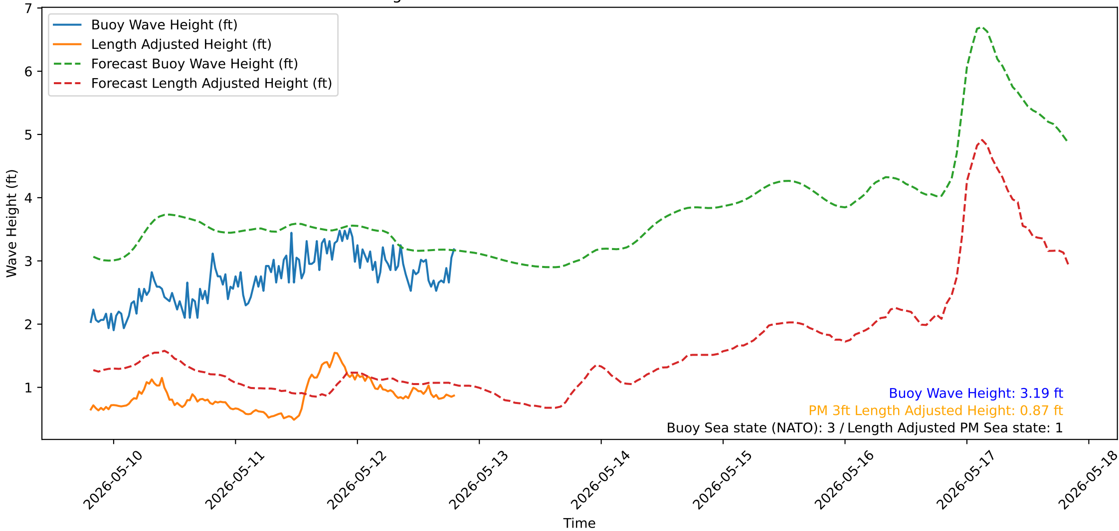
Wave Heights over Time for Green Beach at 2026-05-12 19:41:13
