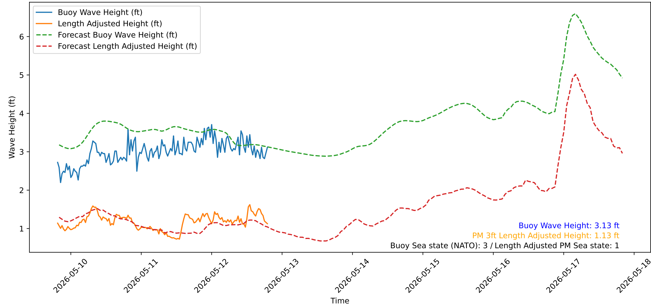
Wave Heights over Time for Oceanside Harbor at 2026-05-12 19:40:31
