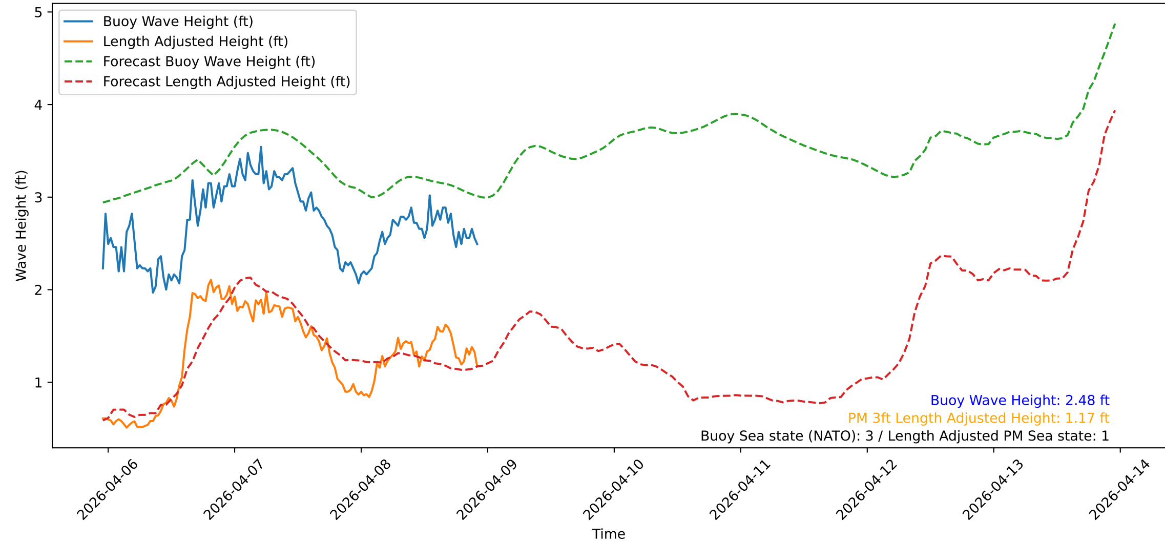
Wave Heights over Time for Red Beach at 2026-04-08 22:50:48
