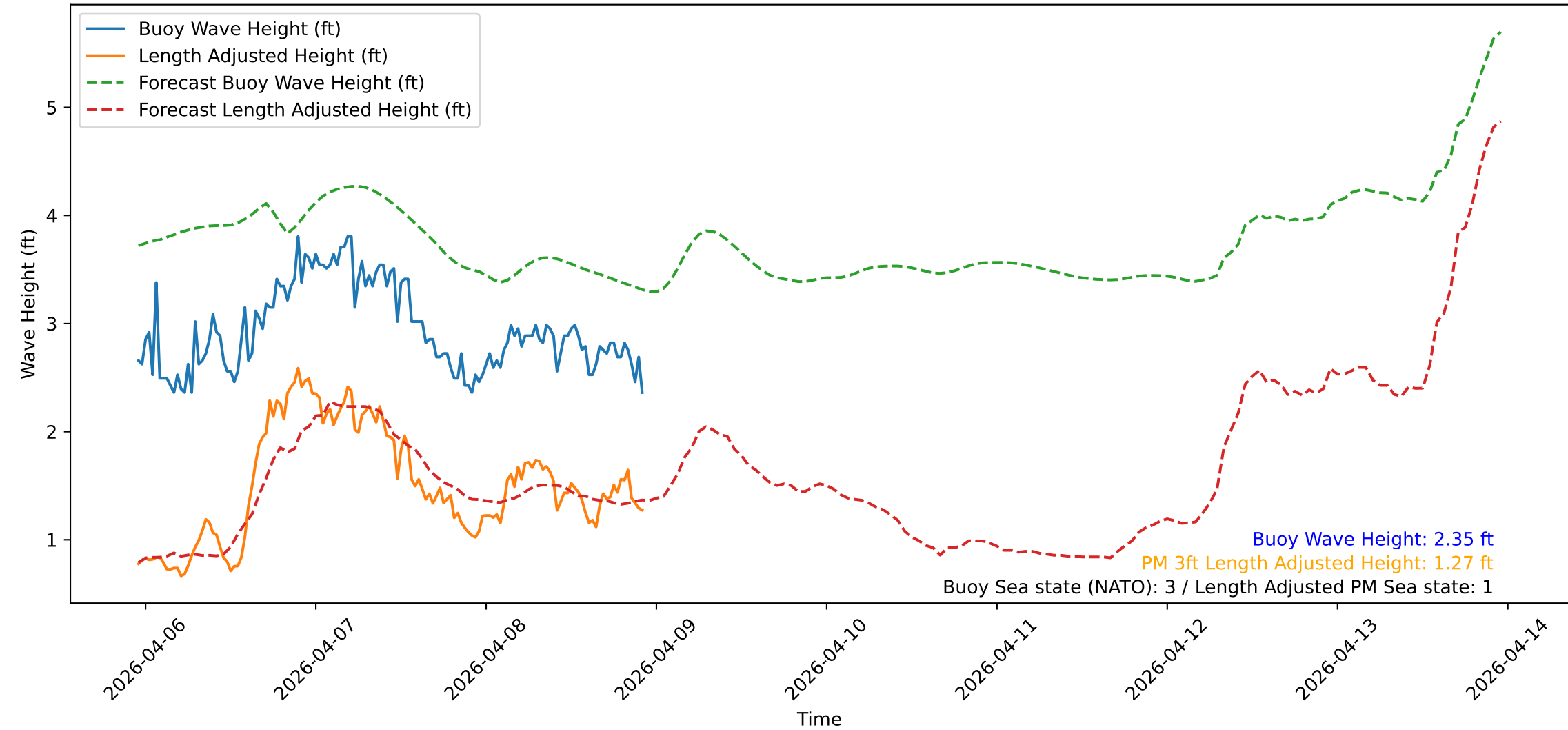
Wave Heights over Time for Green Beach at 2026-04-08 22:51:10
