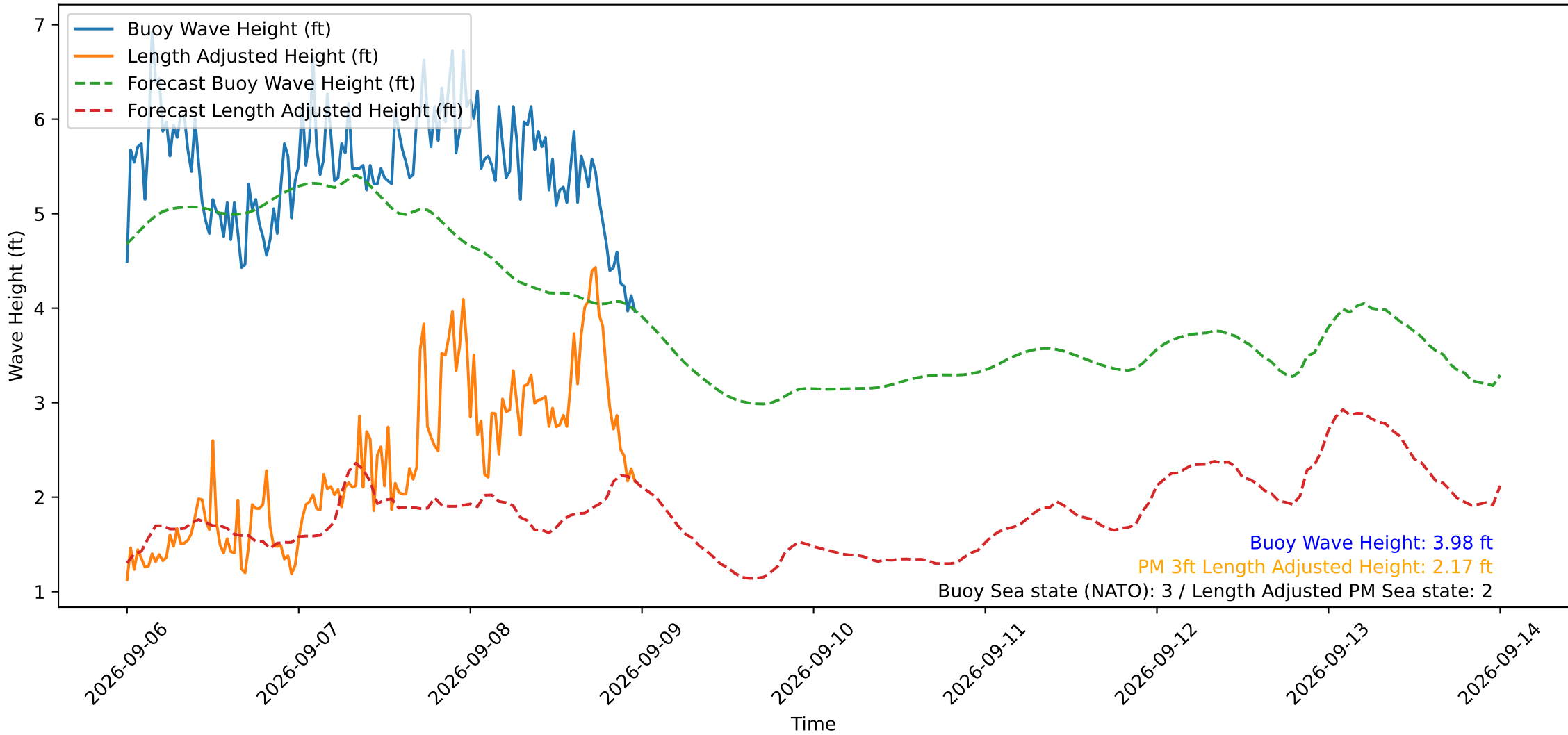
Wave Heights over Time for Red Beach at 2026-09-08 23:40:48
