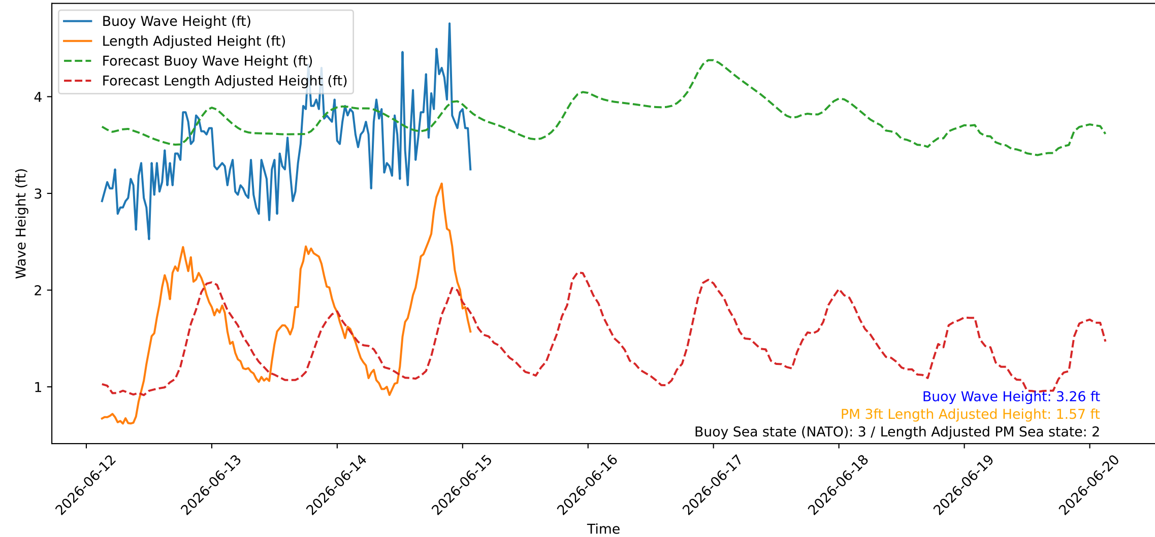
Wave Heights over Time for Red Beach at 2026-06-15 02:30:46
