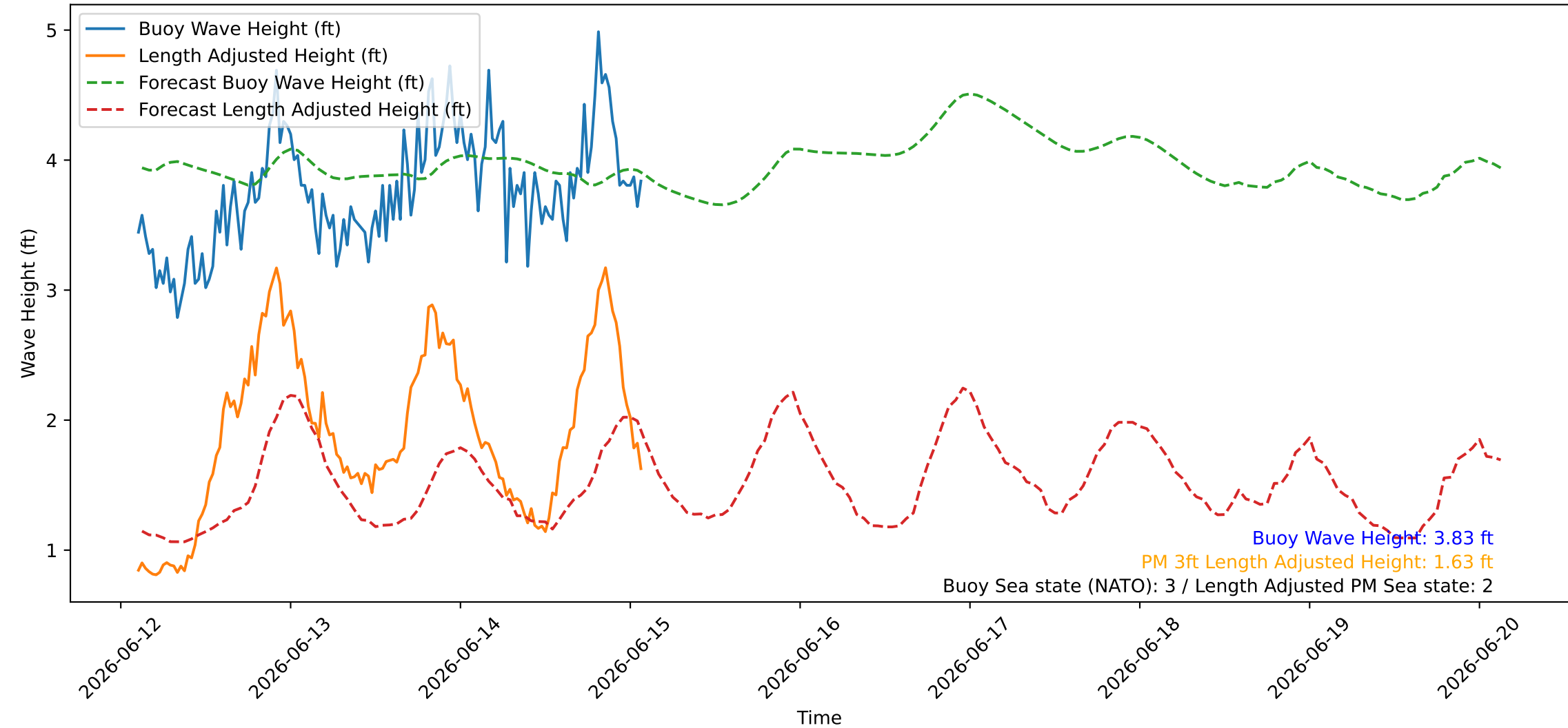
Wave Heights over Time for Oceanside Harbor at 2026-06-15 02:30:26
