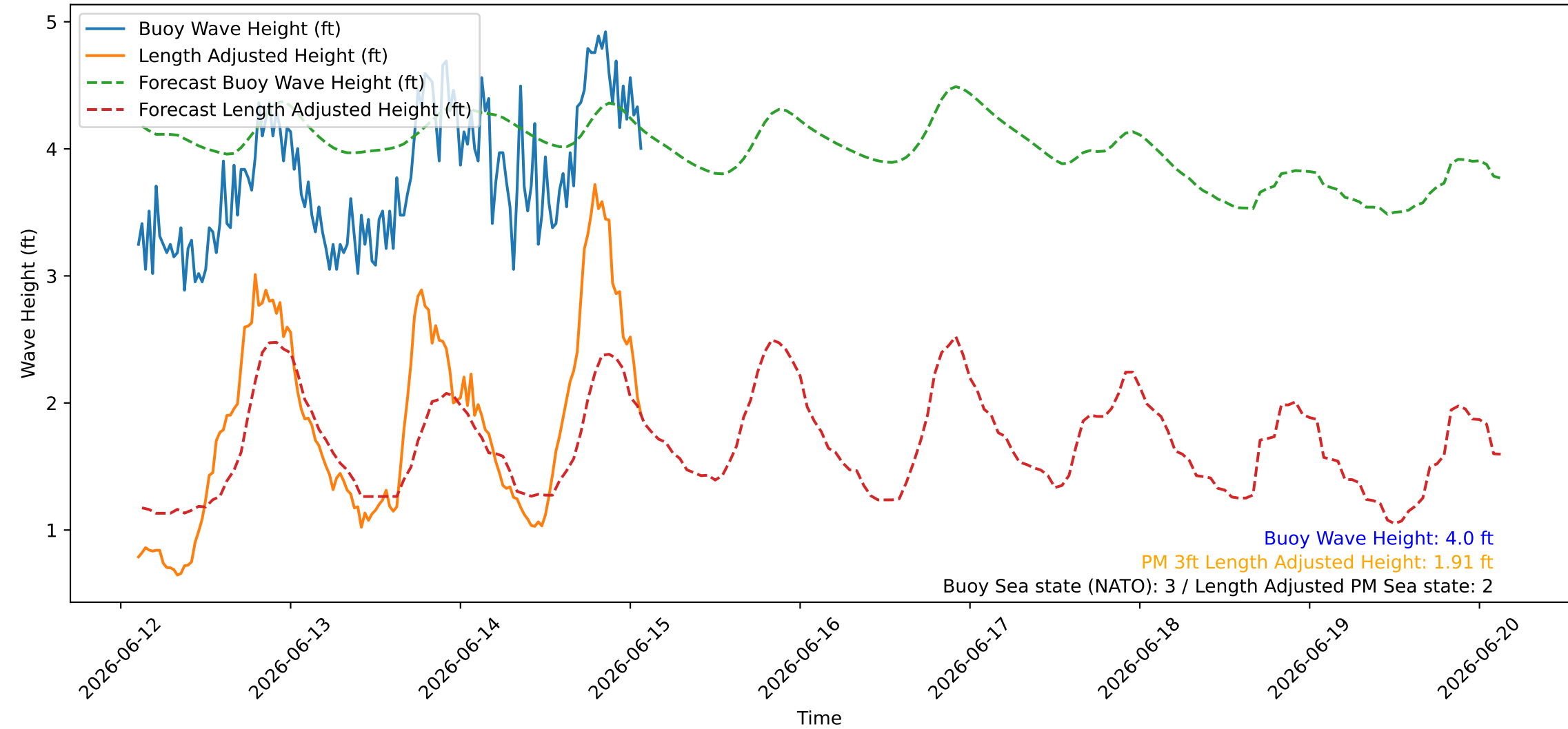
Wave Heights over Time for Green Beach at 2026-06-15 02:31:07
