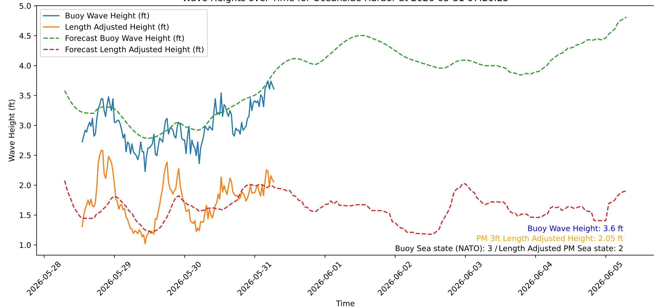
Wave Heights over Time for Oceanside Harbor at 2026-05-31 07:20:25
