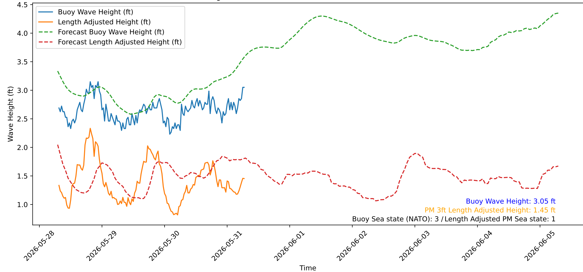
Wave Heights over Time for Red Beach at 2026-05-31 07:20:45
