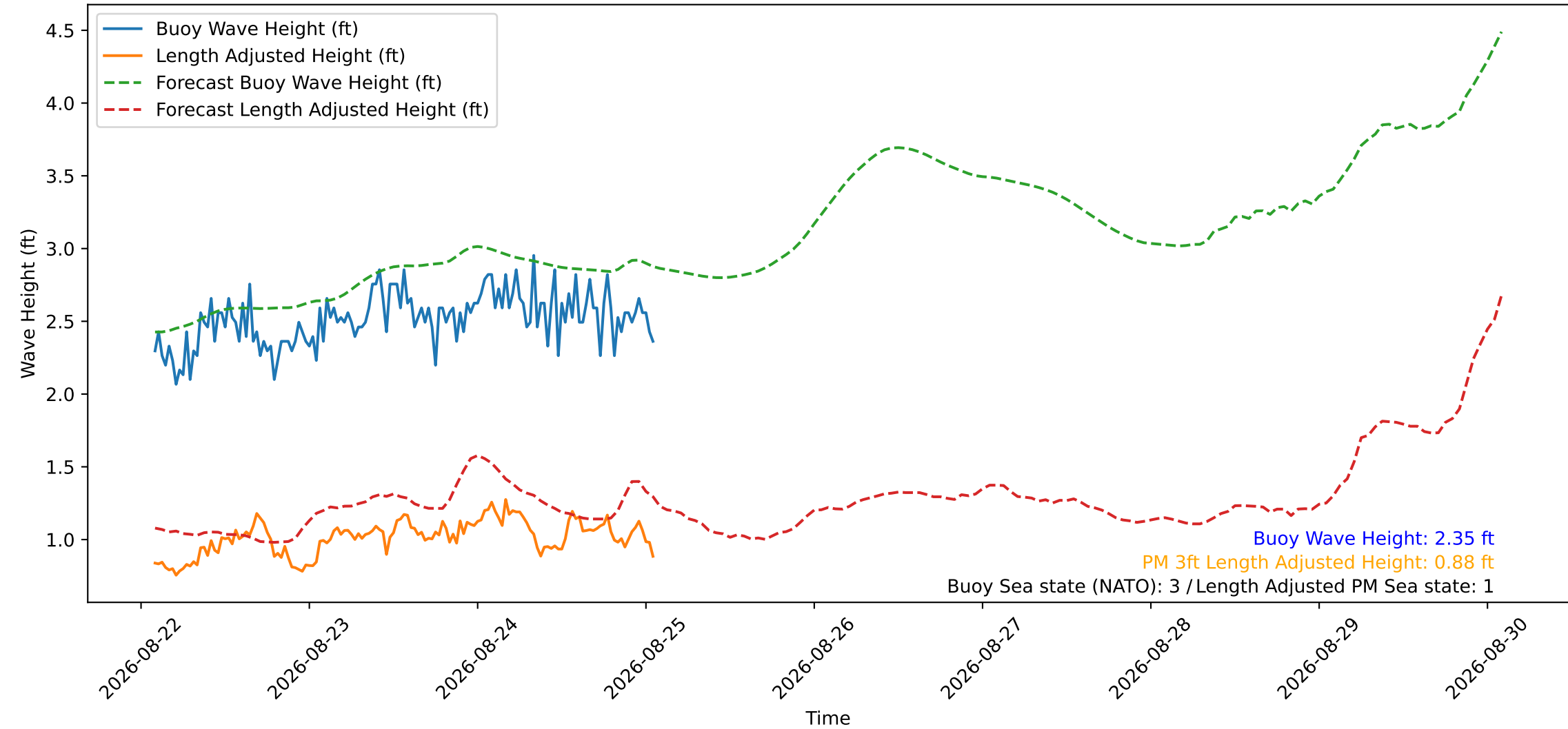
Wave Heights over Time for Red Beach at 2026-08-25 01:40:50
