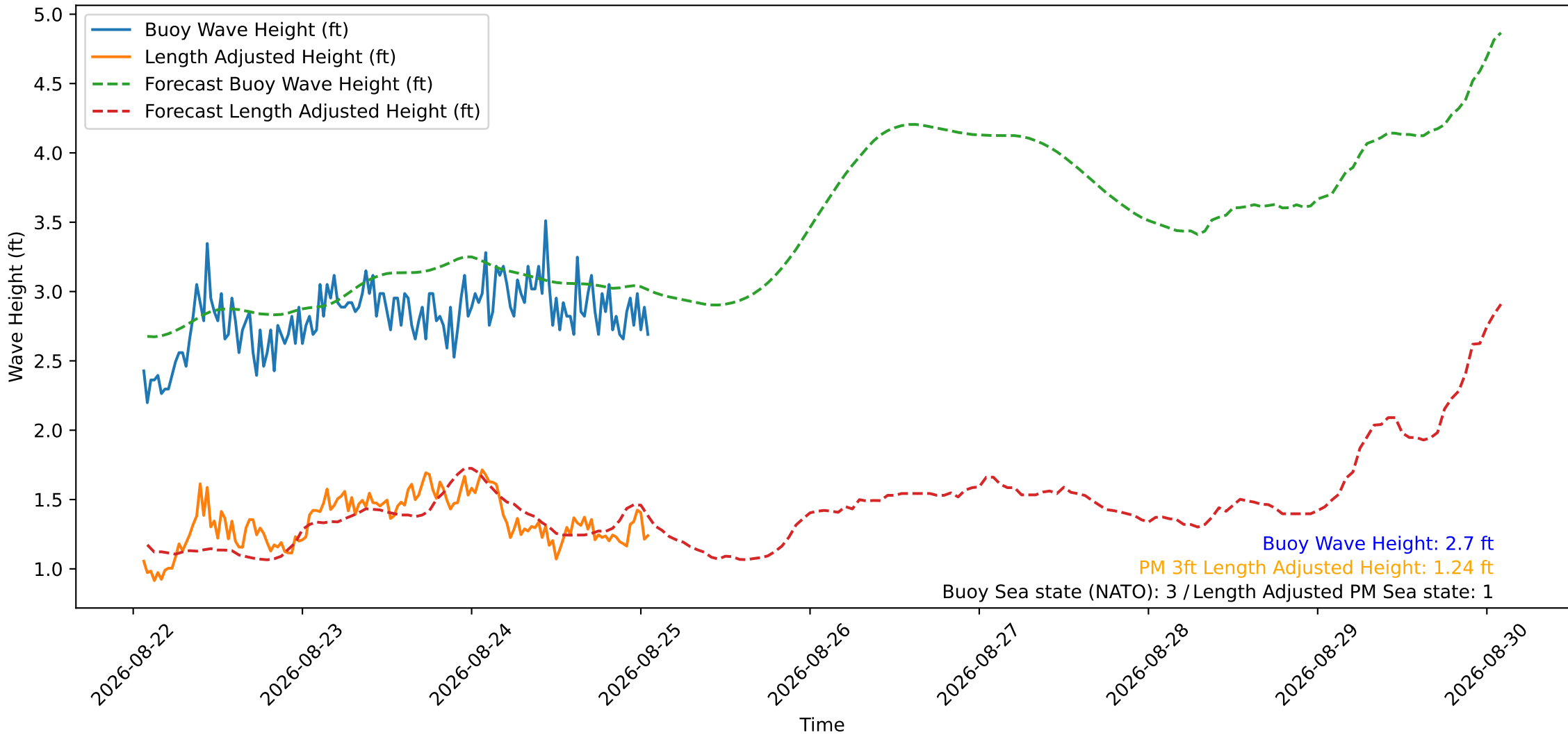
Wave Heights over Time for Oceanside Harbor at 2026-08-25 01:40:30
