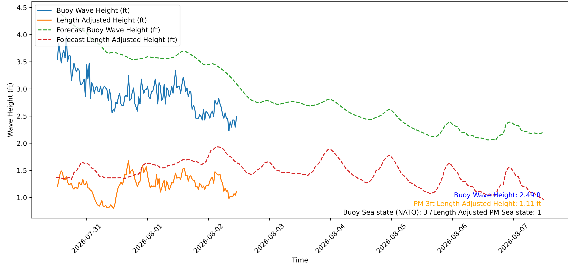
Wave Heights over Time for Red Beach at 2026-08-02 12:00:45
