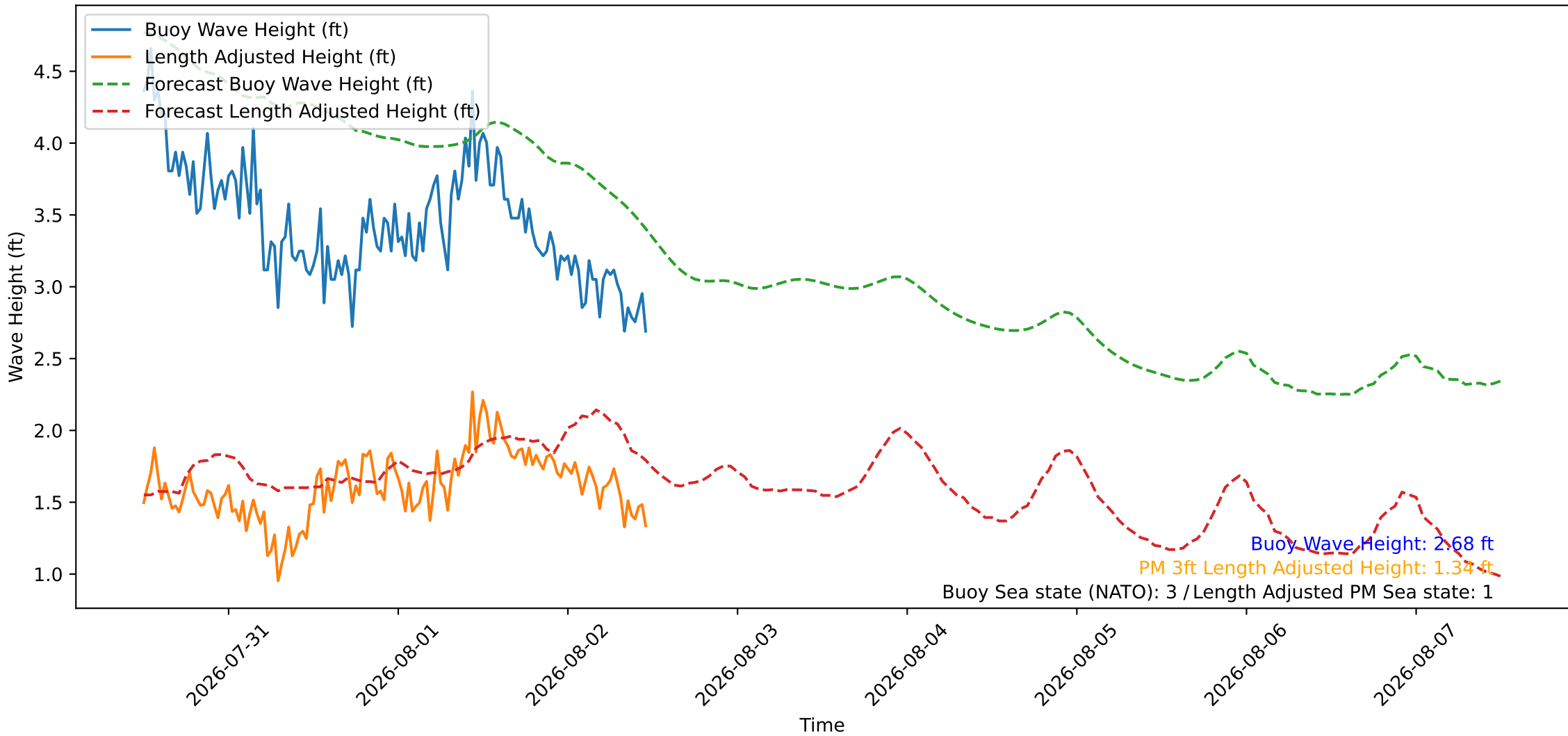
Wave Heights over Time for Oceanside Harbor at 2026-08-02 12:00:26
