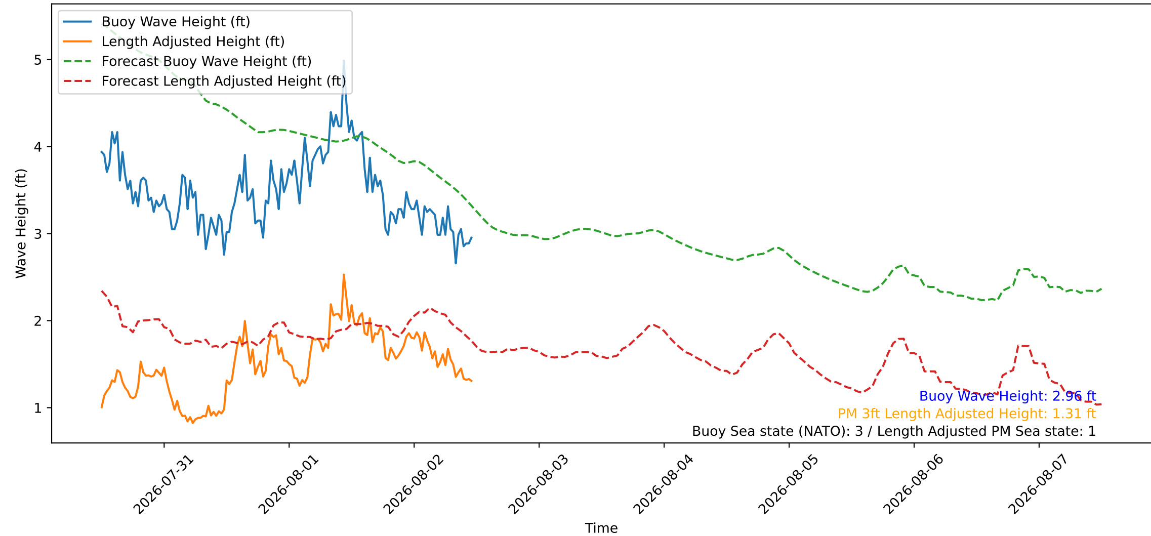
Wave Heights over Time for Green Beach at 2026-08-02 12:01:08
