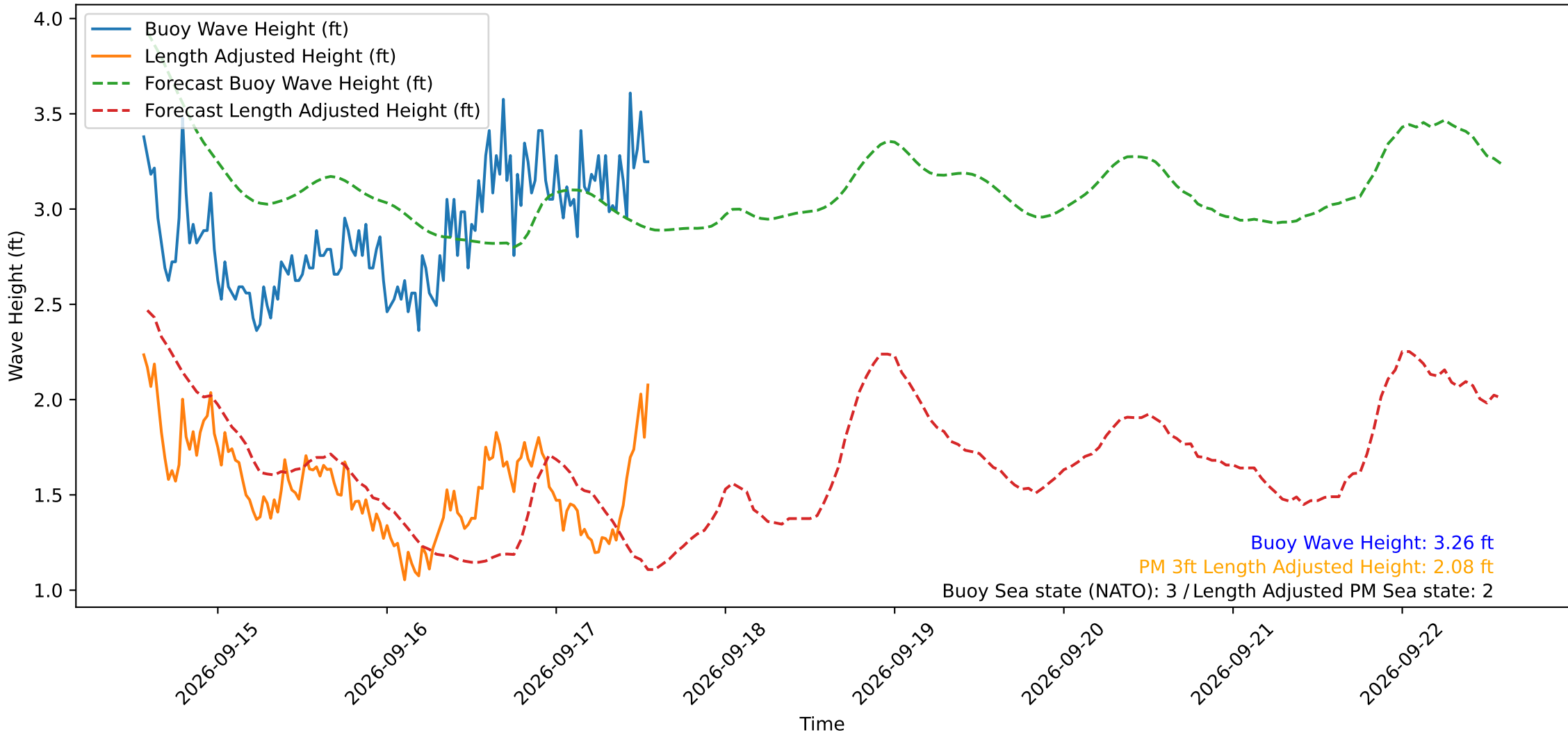
Wave Heights over Time for Oceanside Harbor at 2026-09-17 13:30:30
