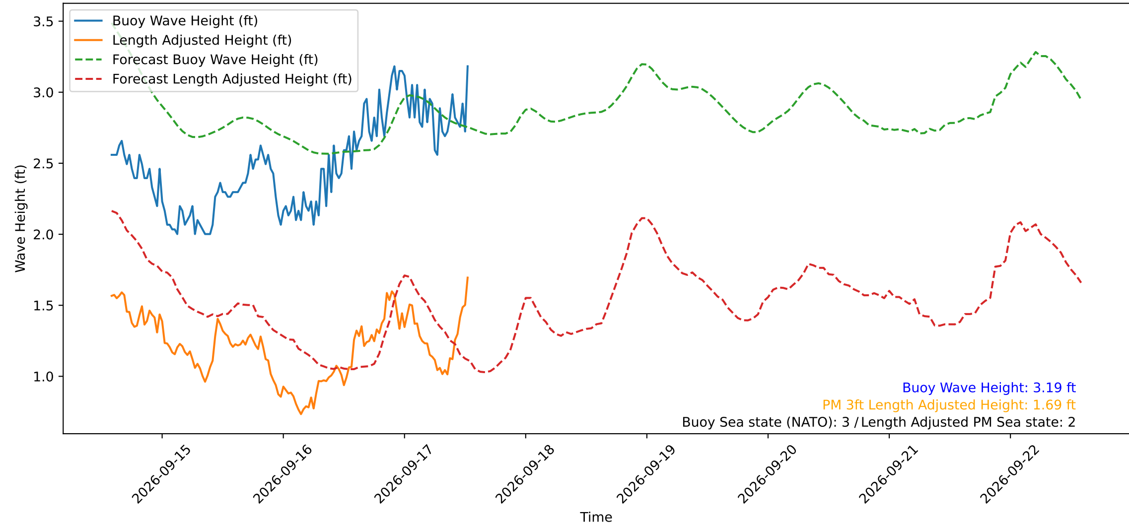
Wave Heights over Time for Red Beach at 2026-09-17 13:30:49
