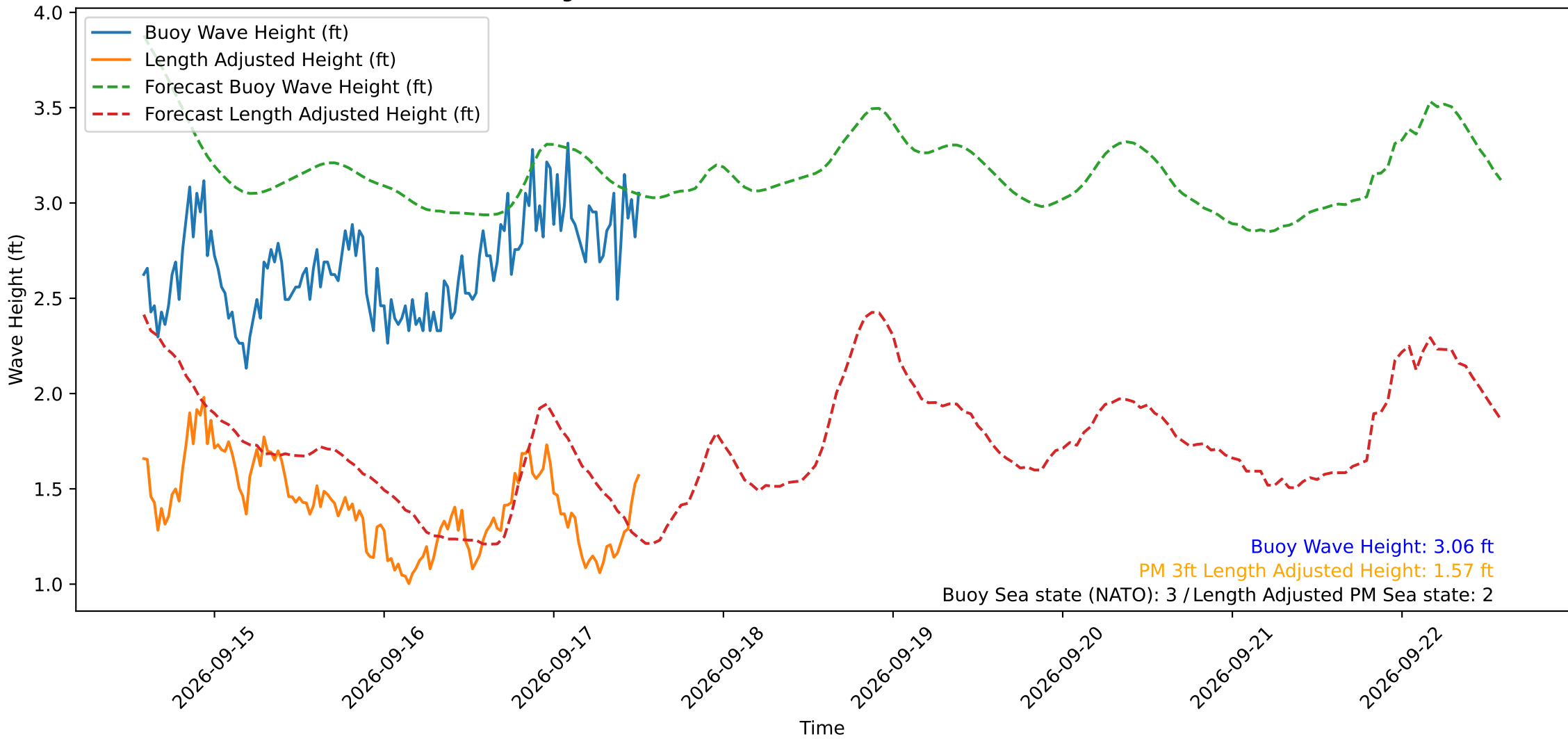
Wave Heights over Time for Green Beach at 2026-09-17 13:31:12
