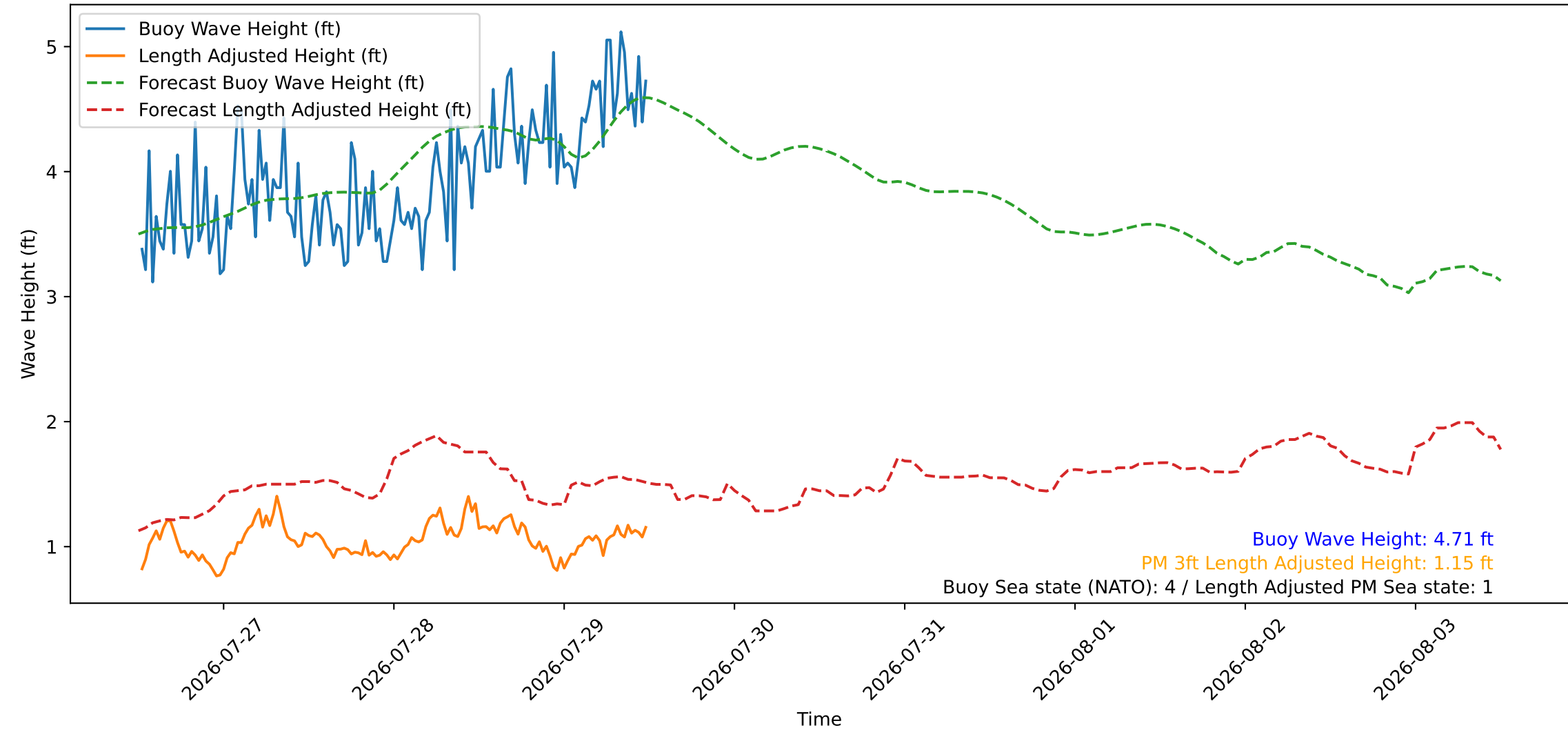
Wave Heights over Time for Red Beach at 2026-07-29 12:20:47
