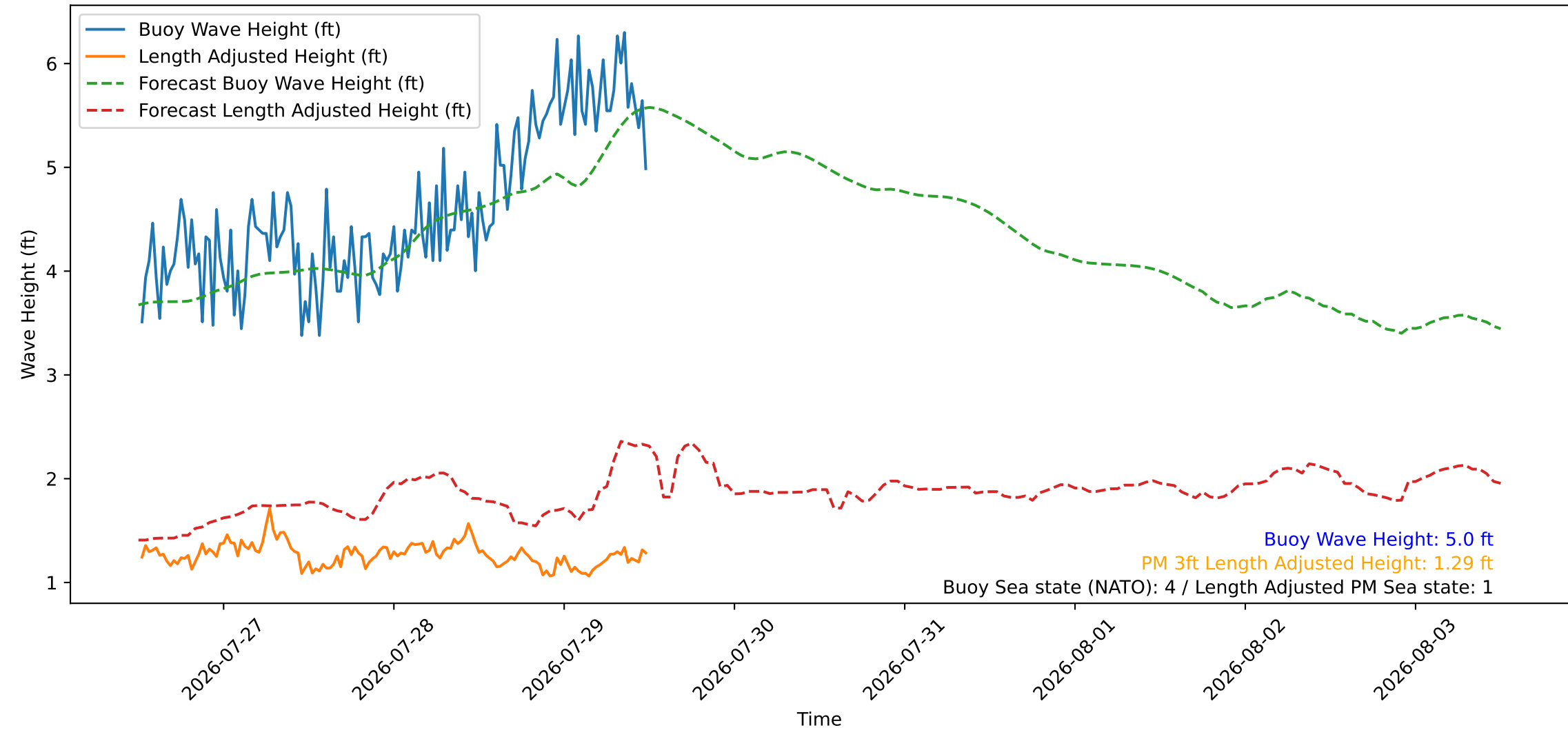
Wave Heights over Time for Green Beach at 2026-07-29 12:21:09
