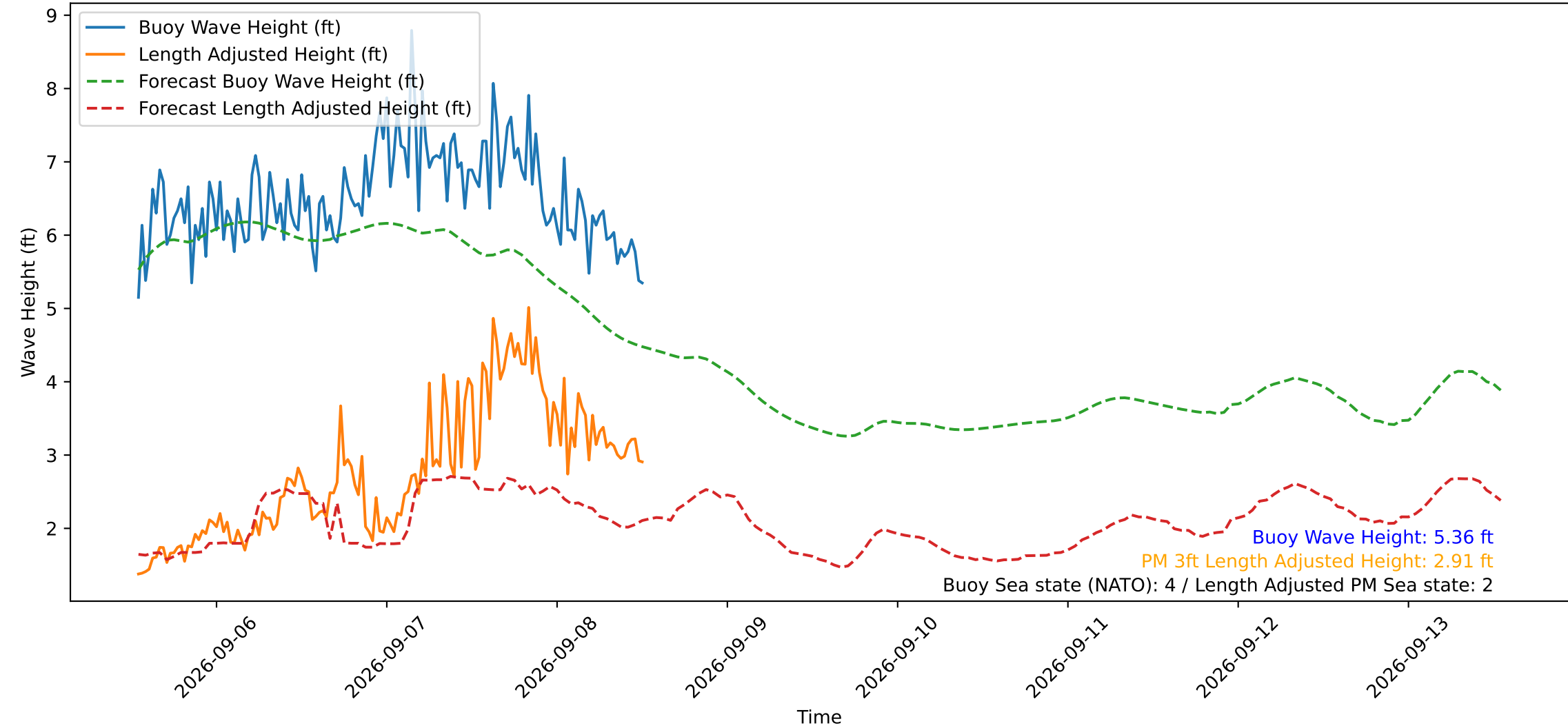
Wave Heights over Time for Green Beach at 2026-09-08 12:51:14
