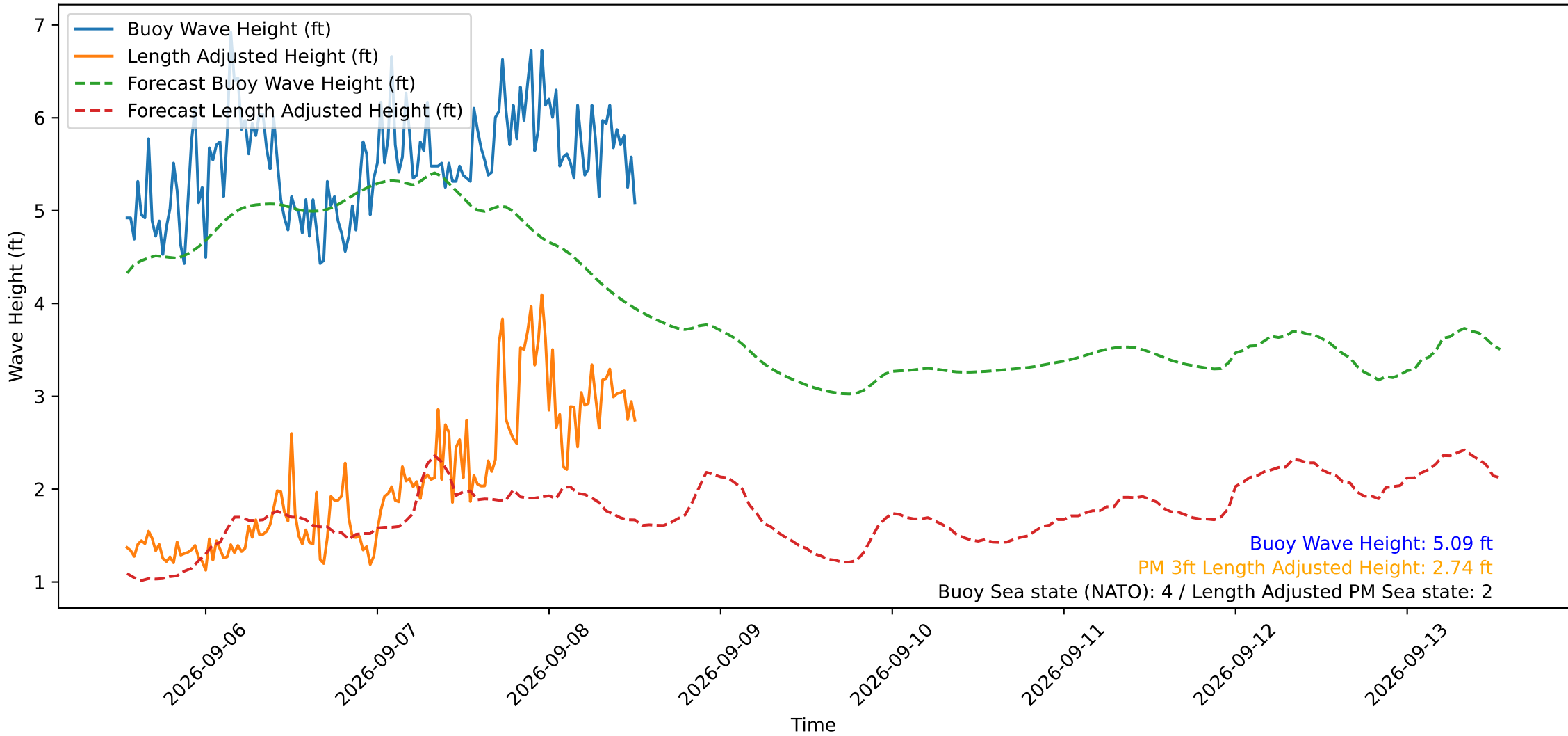
Wave Heights over Time for Red Beach at 2026-09-08 12:50:50
