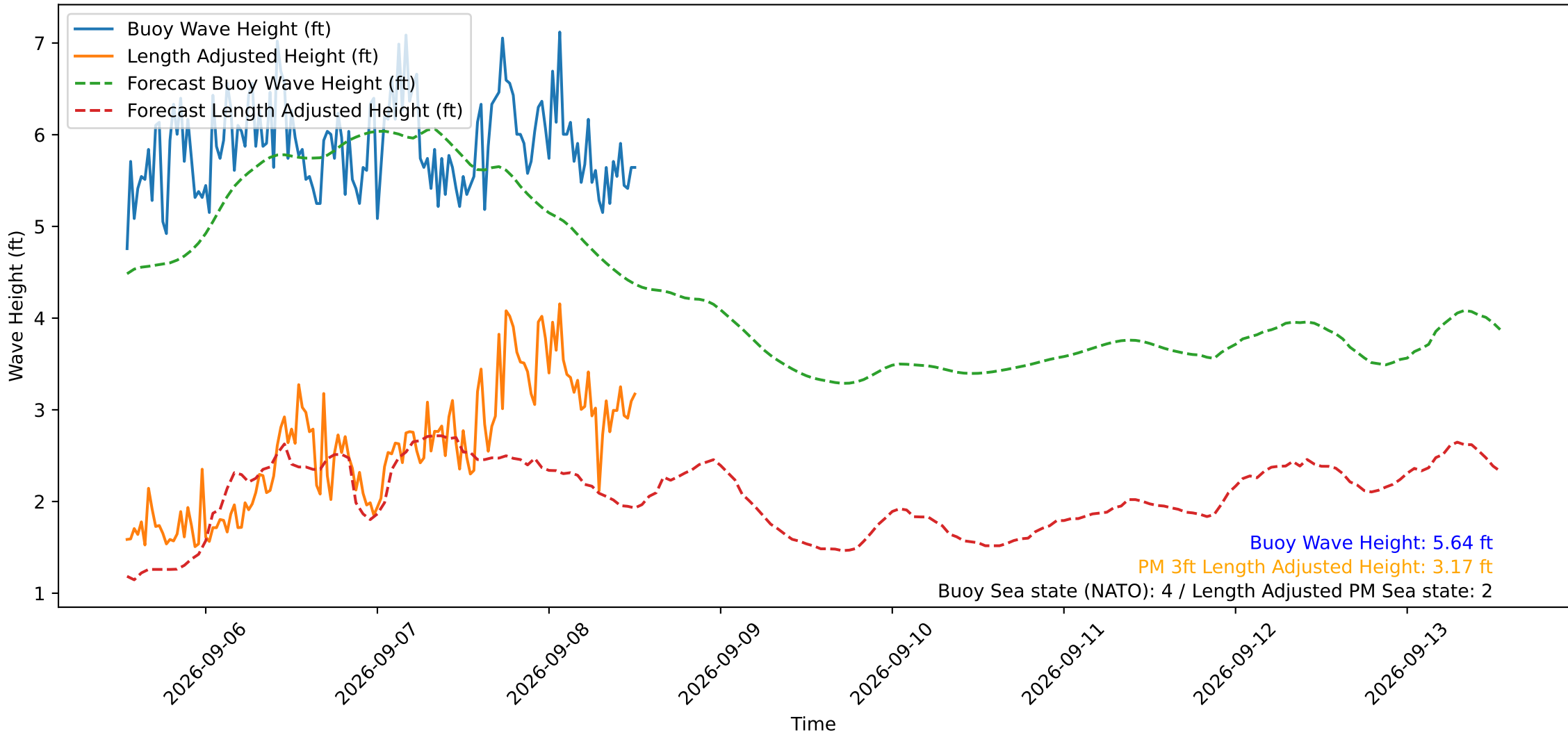
Wave Heights over Time for Oceanside Harbor at 2026-09-08 12:50:30
