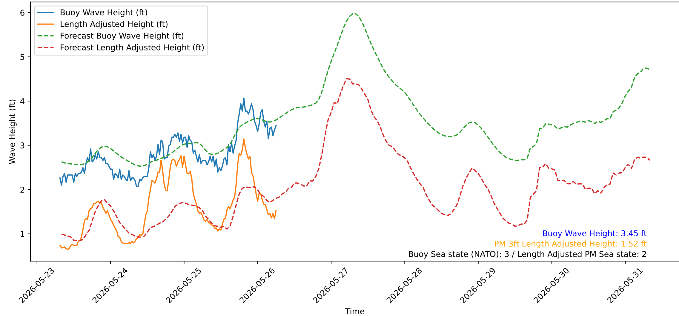
Wave Heights over Time for Green Beach at 2026-05-26 07:31:10
