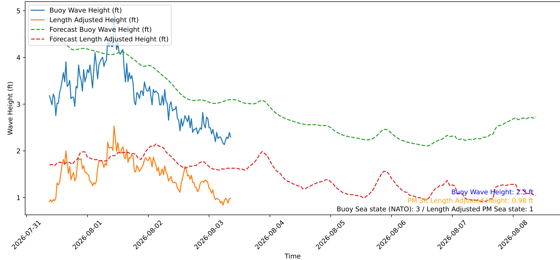
Wave Heights over Time for Green Beach at 2026-08-03 09:11:08
