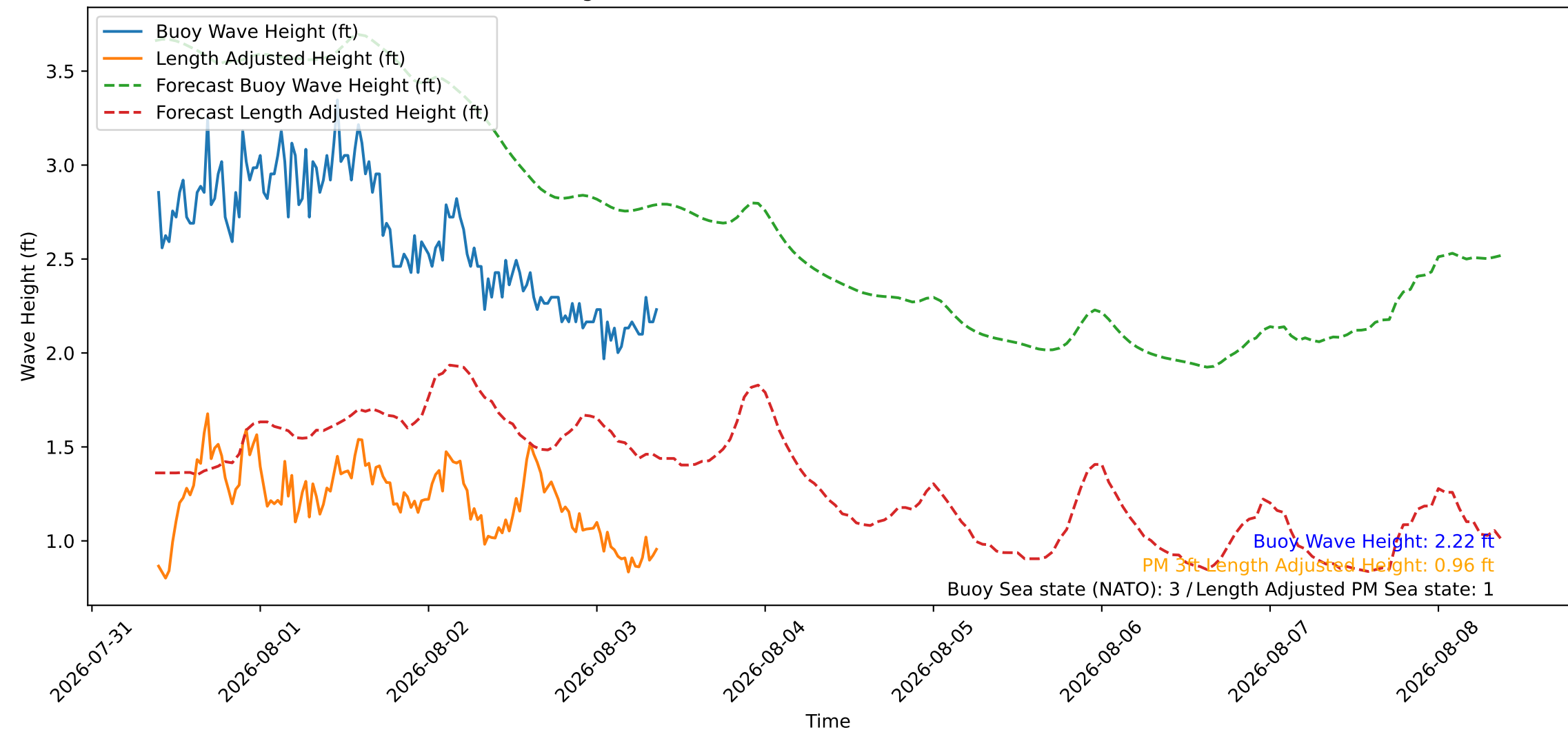
Wave Heights over Time for Red Beach at 2026-08-03 09:10:46
