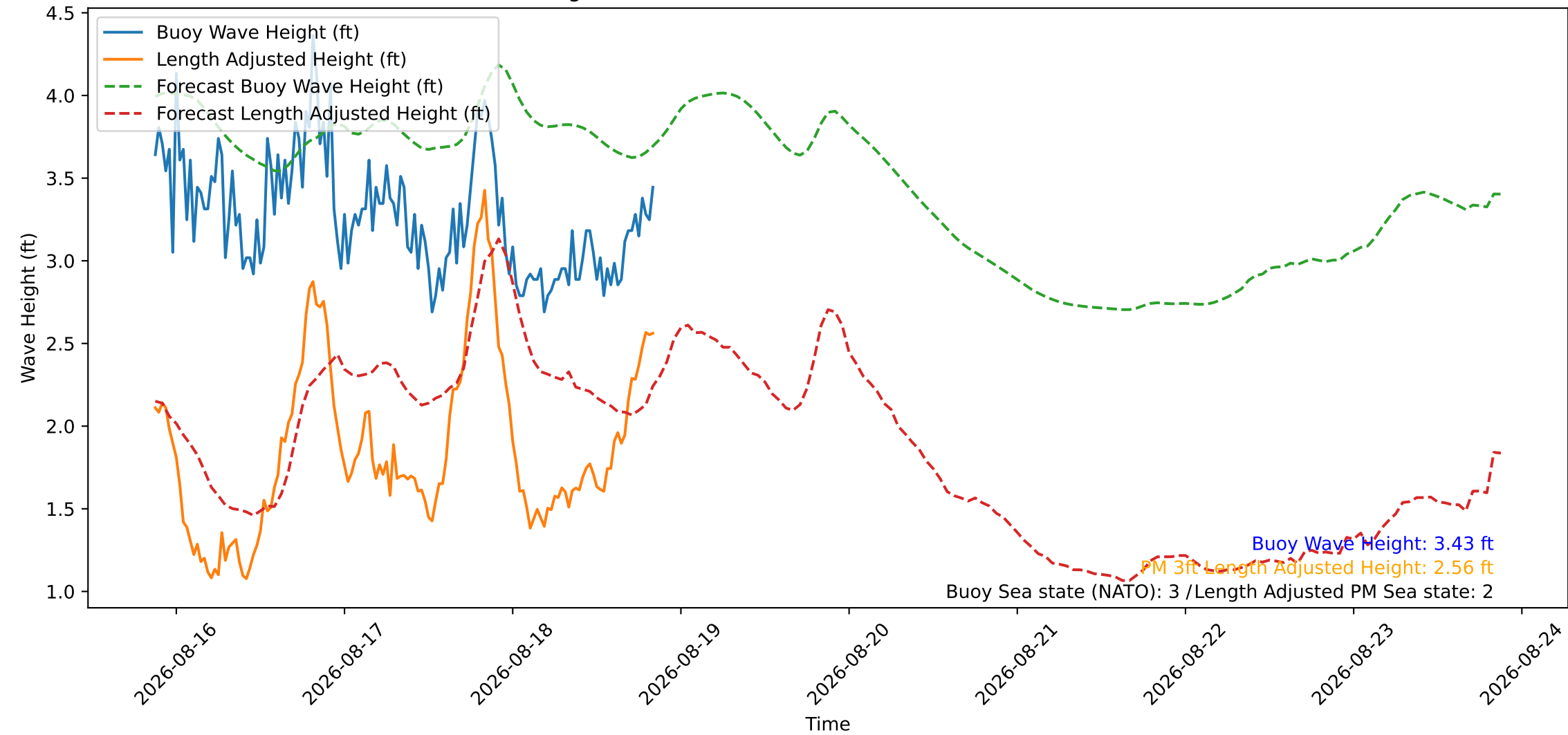
Wave Heights over Time for Green Beach at 2026-08-18 20:41:08
