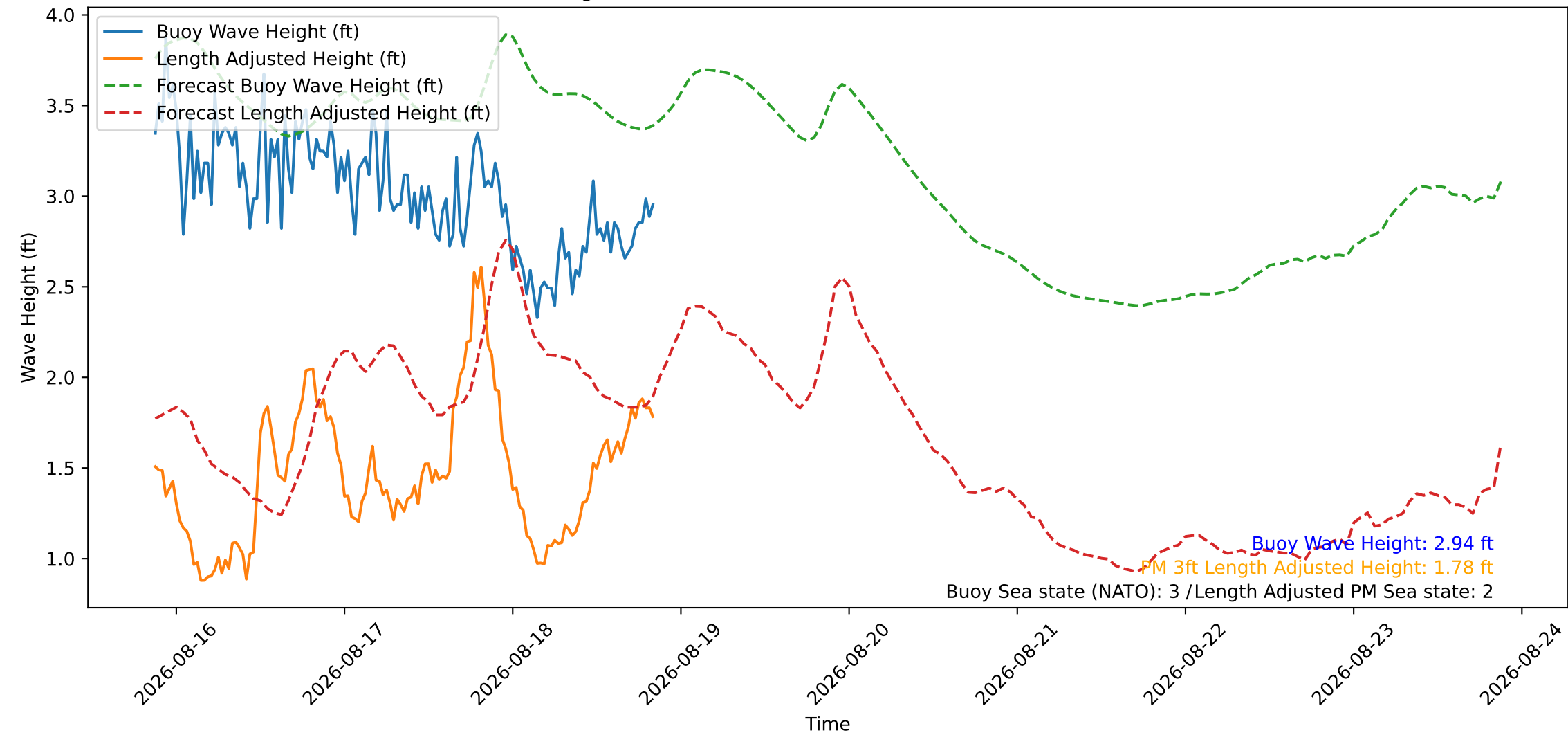
Wave Heights over Time for Red Beach at 2026-08-18 20:40:46
