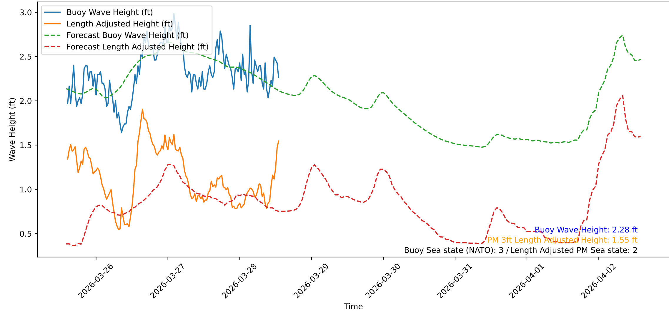
Wave Heights over Time for Red Beach at 2026-03-28 14:00:47
