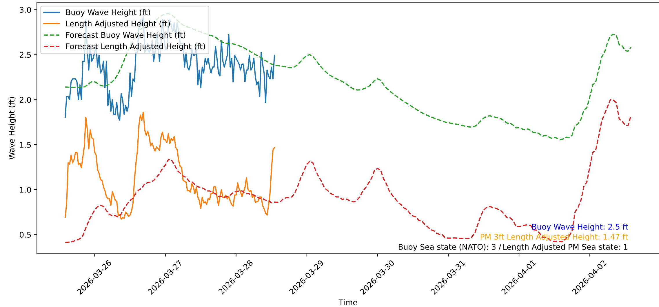
Wave Heights over Time for Oceanside Harbor at 2026-03-28 14:00:31
