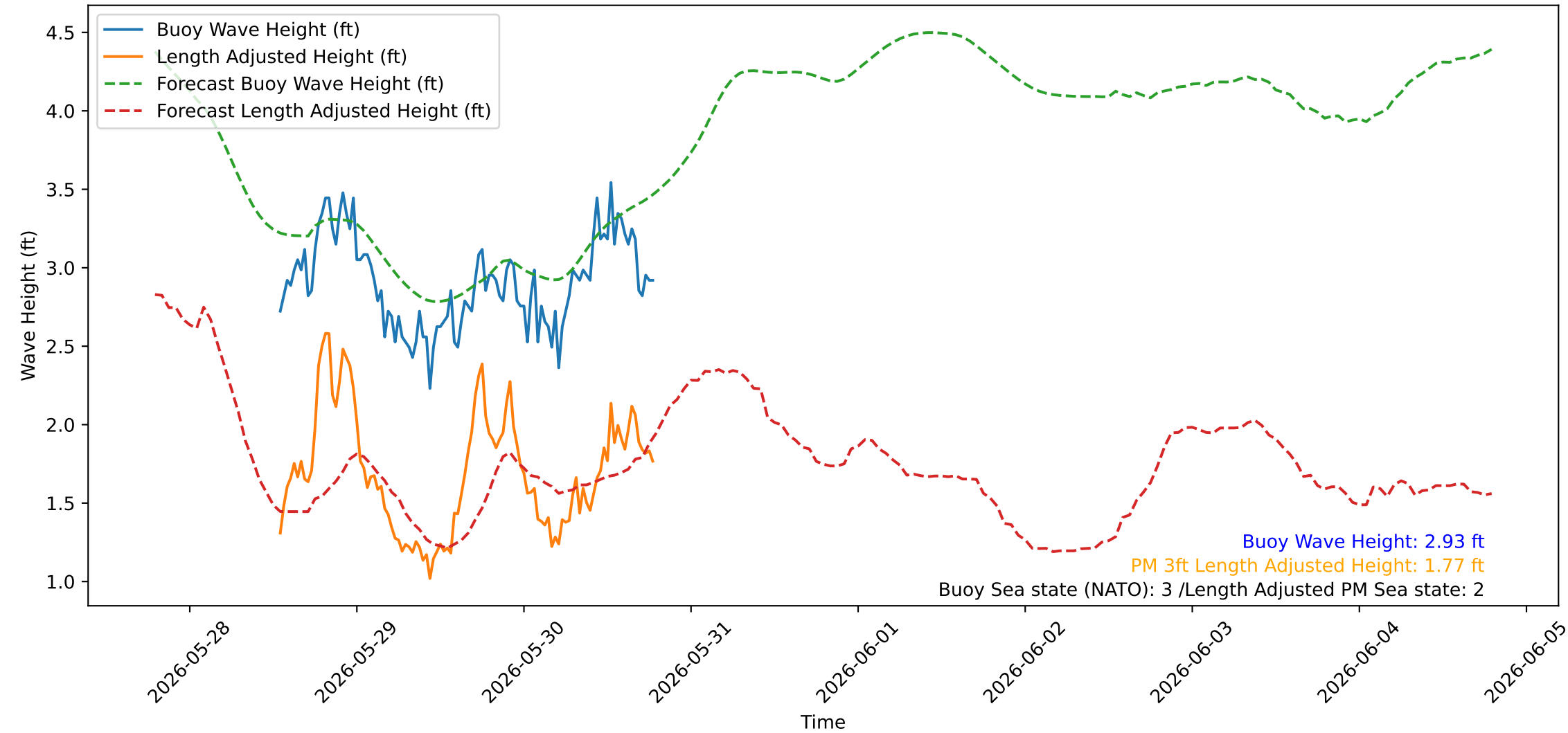
Wave Heights over Time for Oceanside Harbor at 2026-05-30 19:00:24
