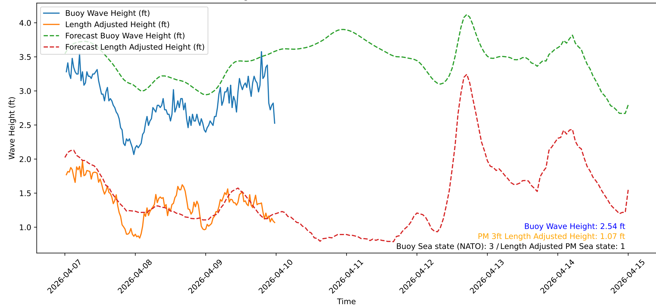
Wave Heights over Time for Red Beach at 2026-04-10 00:10:51
