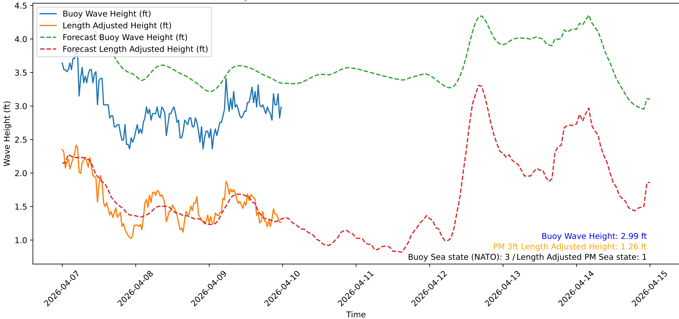
Wave Heights over Time for Green Beach at 2026-04-10 00:11:14
