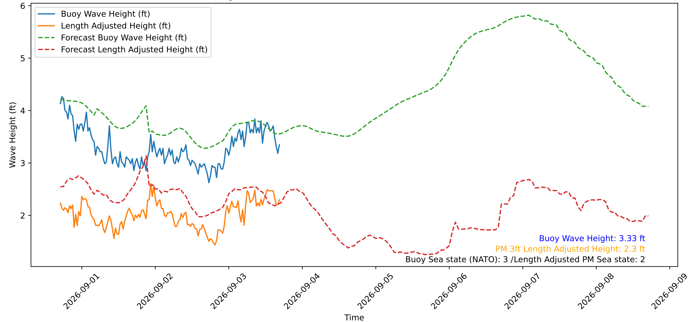
Wave Heights over Time for Oceanside Harbor at 2026-09-03 17:00:30
