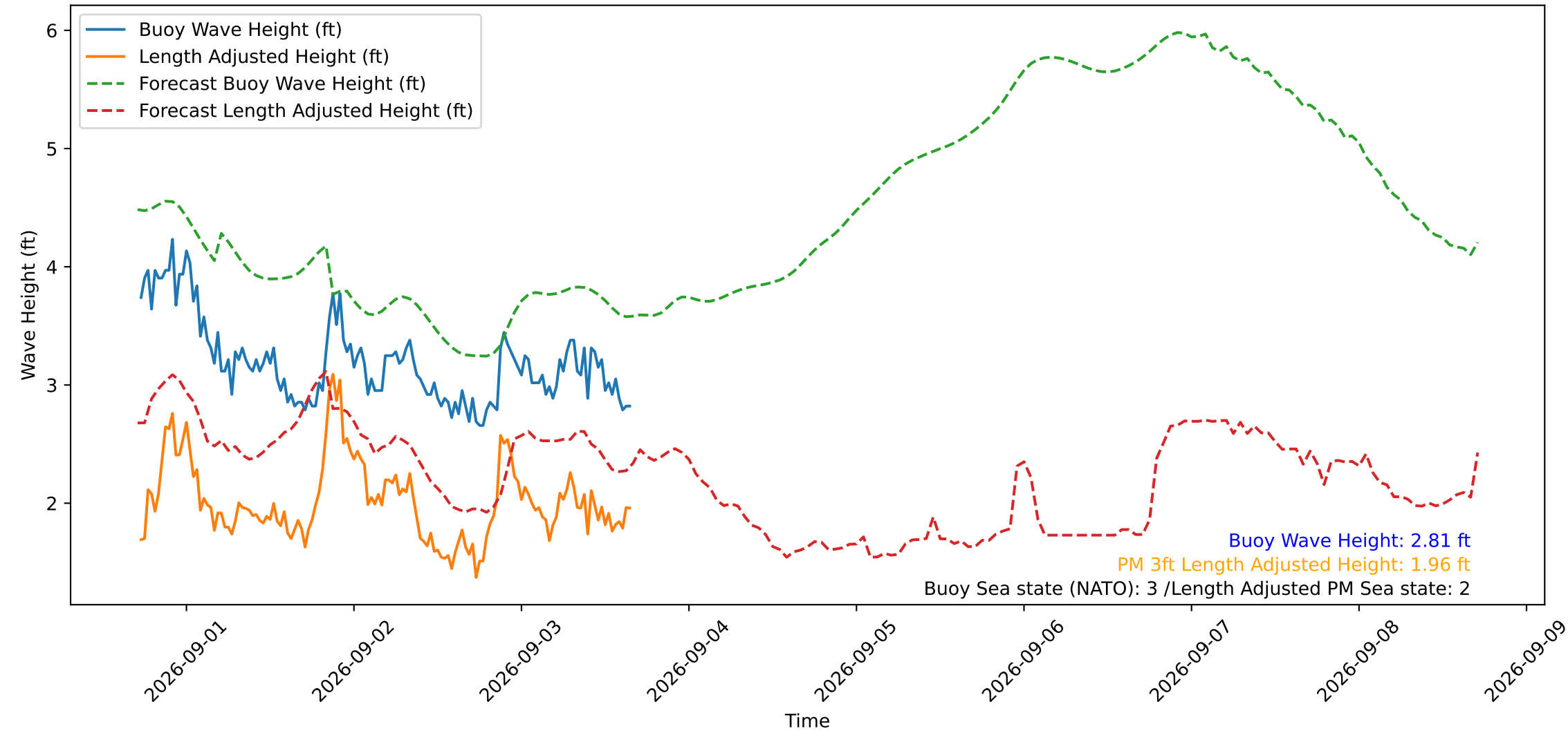
Wave Heights over Time for Green Beach at 2026-09-03 17:01:12
