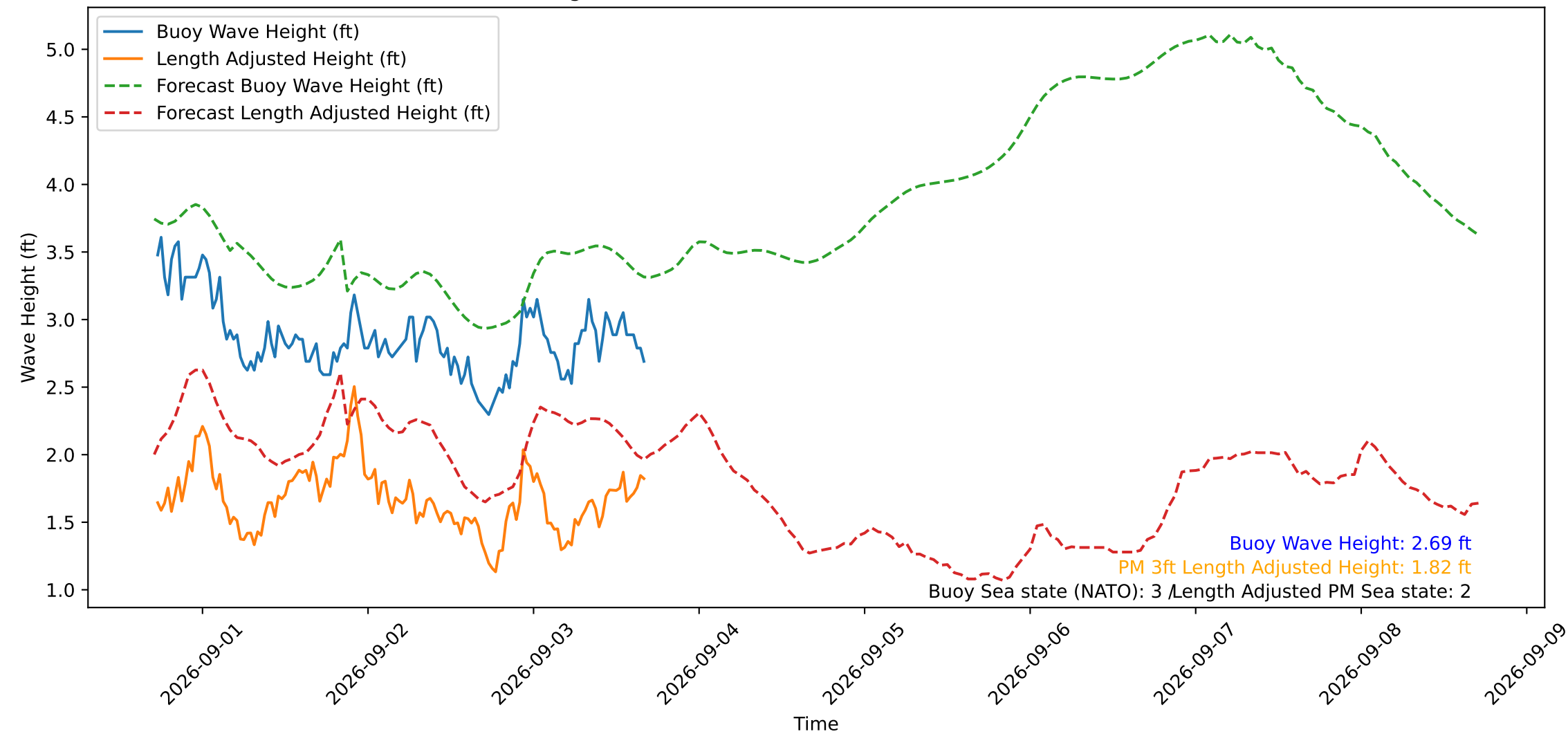
Wave Heights over Time for Red Beach at 2026-09-03 17:00:50
