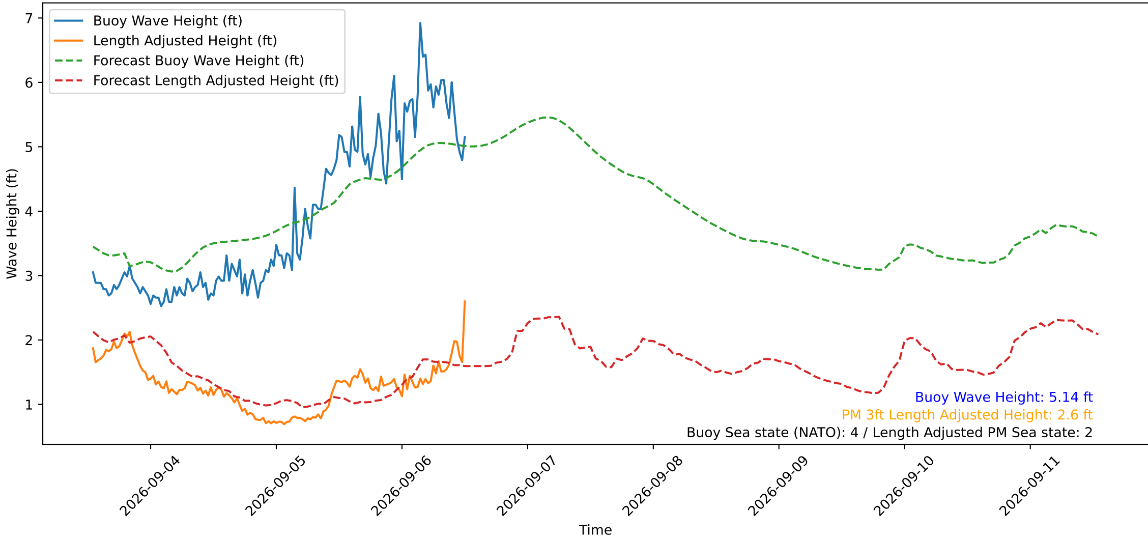
Wave Heights over Time for Red Beach at 2026-09-06 12:40:49
