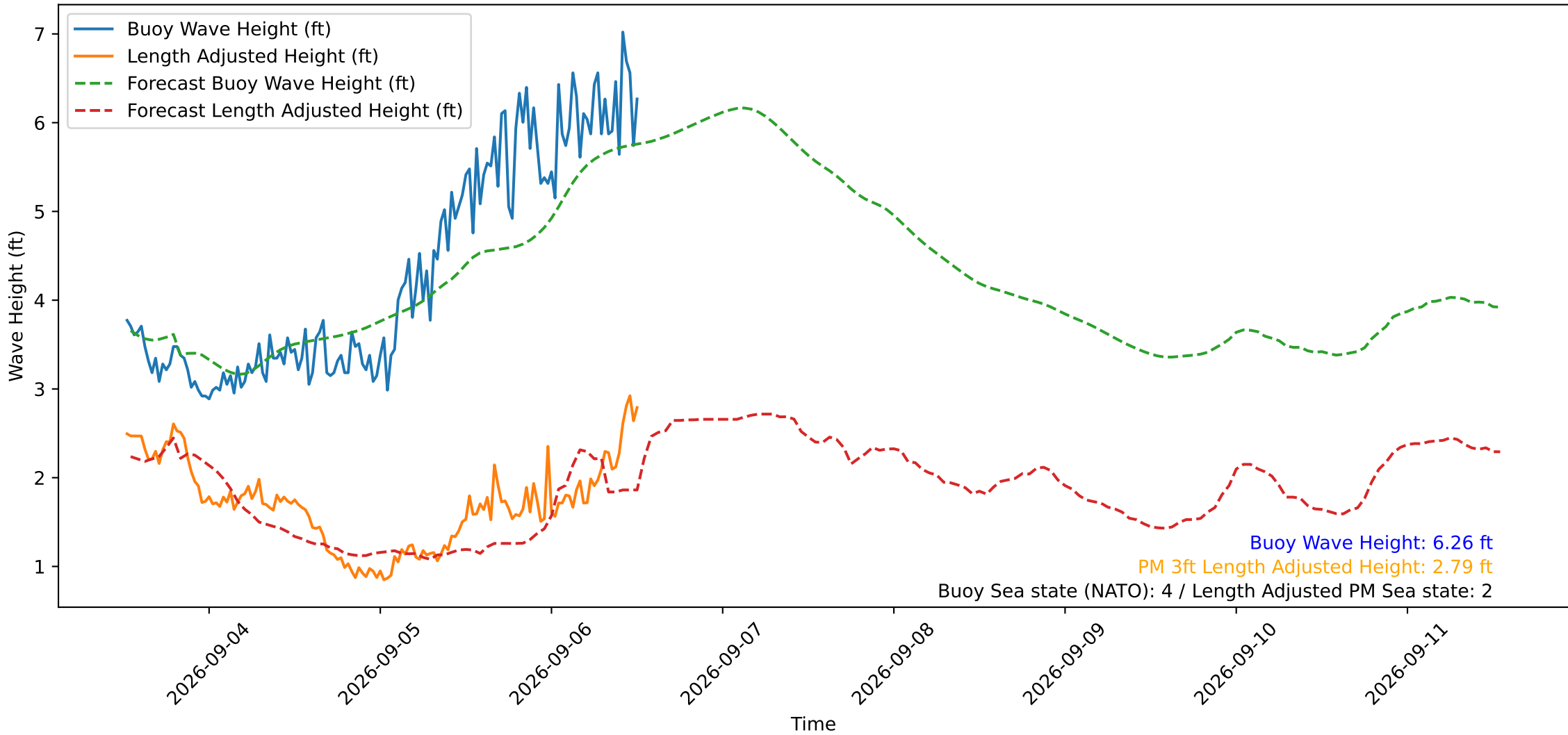
Wave Heights over Time for Oceanside Harbor at 2026-09-06 12:40:29
