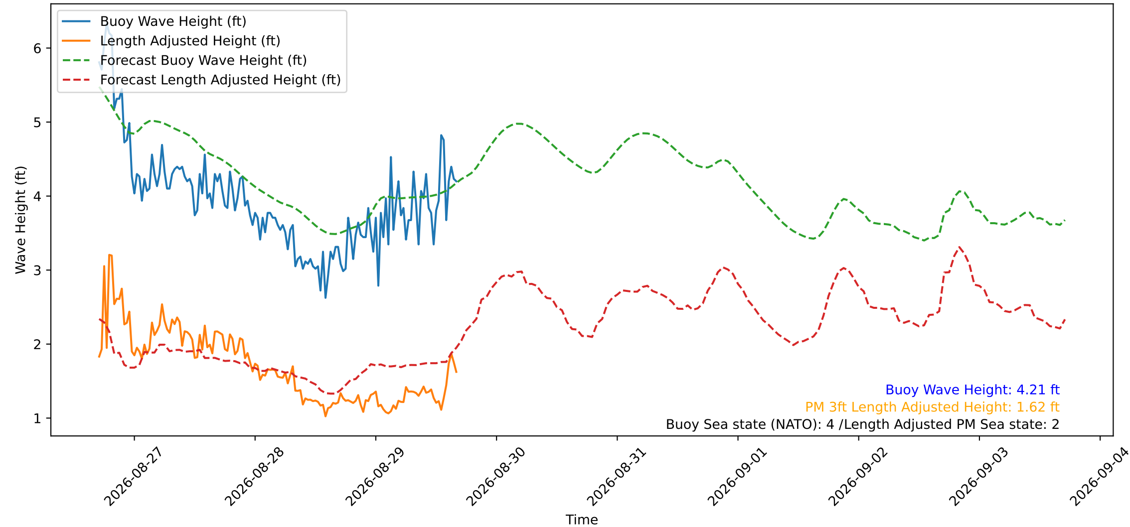
Wave Heights over Time for Green Beach at 2026-08-29 16:51:16
