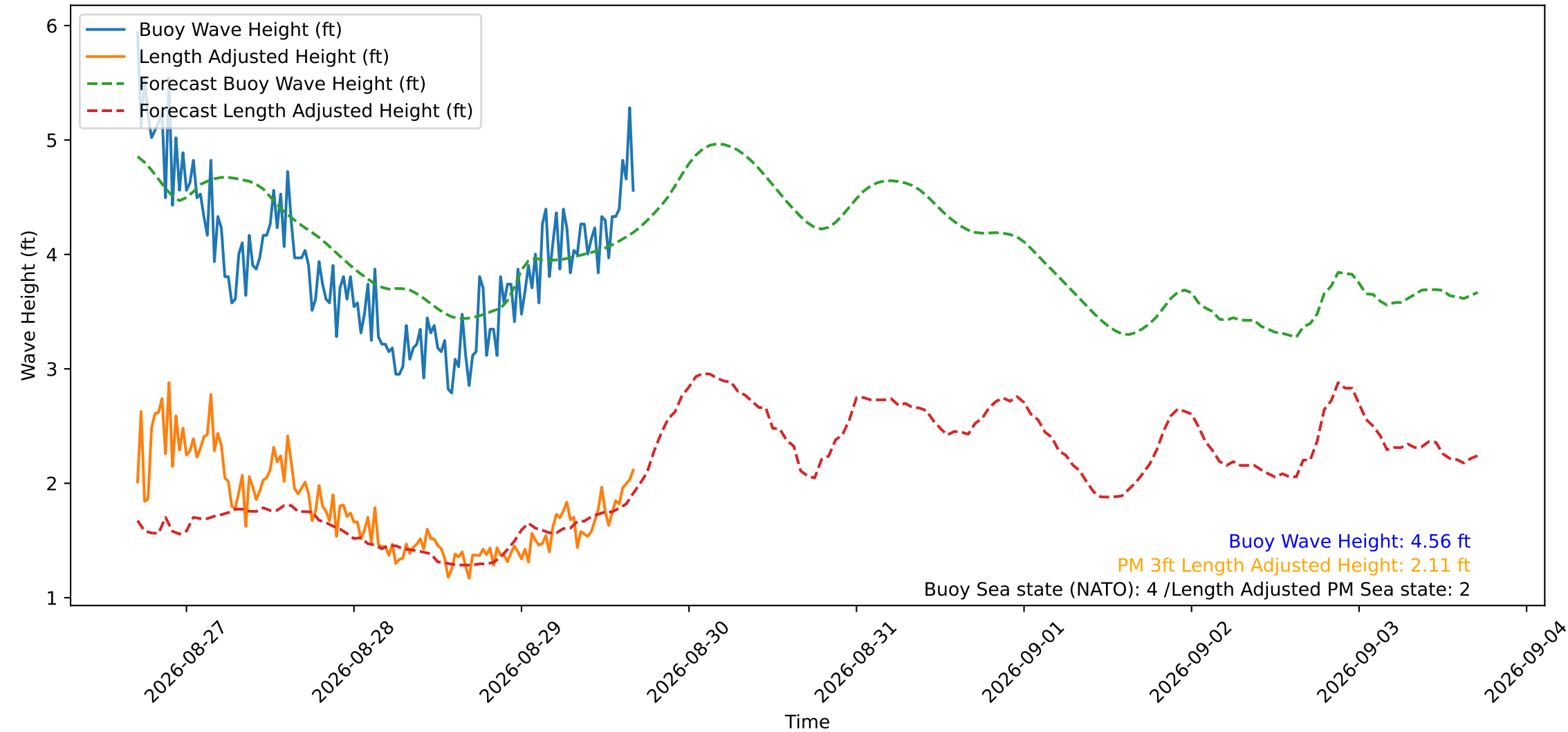
Wave Heights over Time for Oceanside Harbor at 2026-08-29 16:50:32
