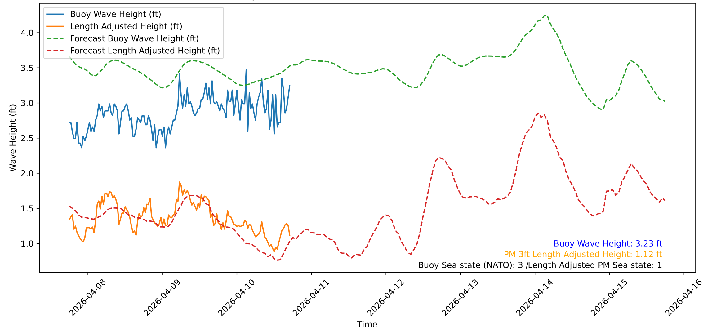
Wave Heights over Time for Green Beach at 2026-04-10 18:01:13
