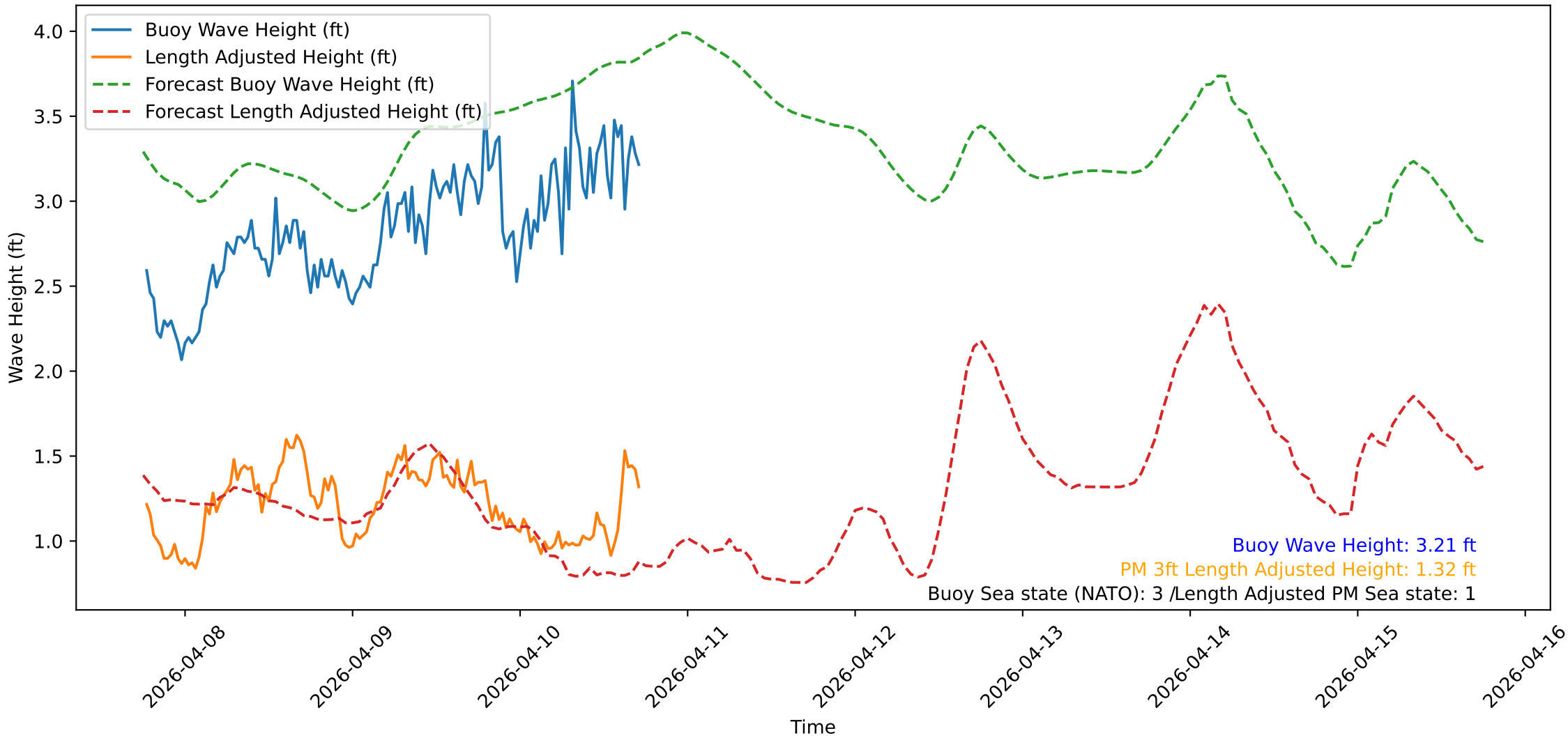
Wave Heights over Time for Red Beach at 2026-04-10 18:00:50
