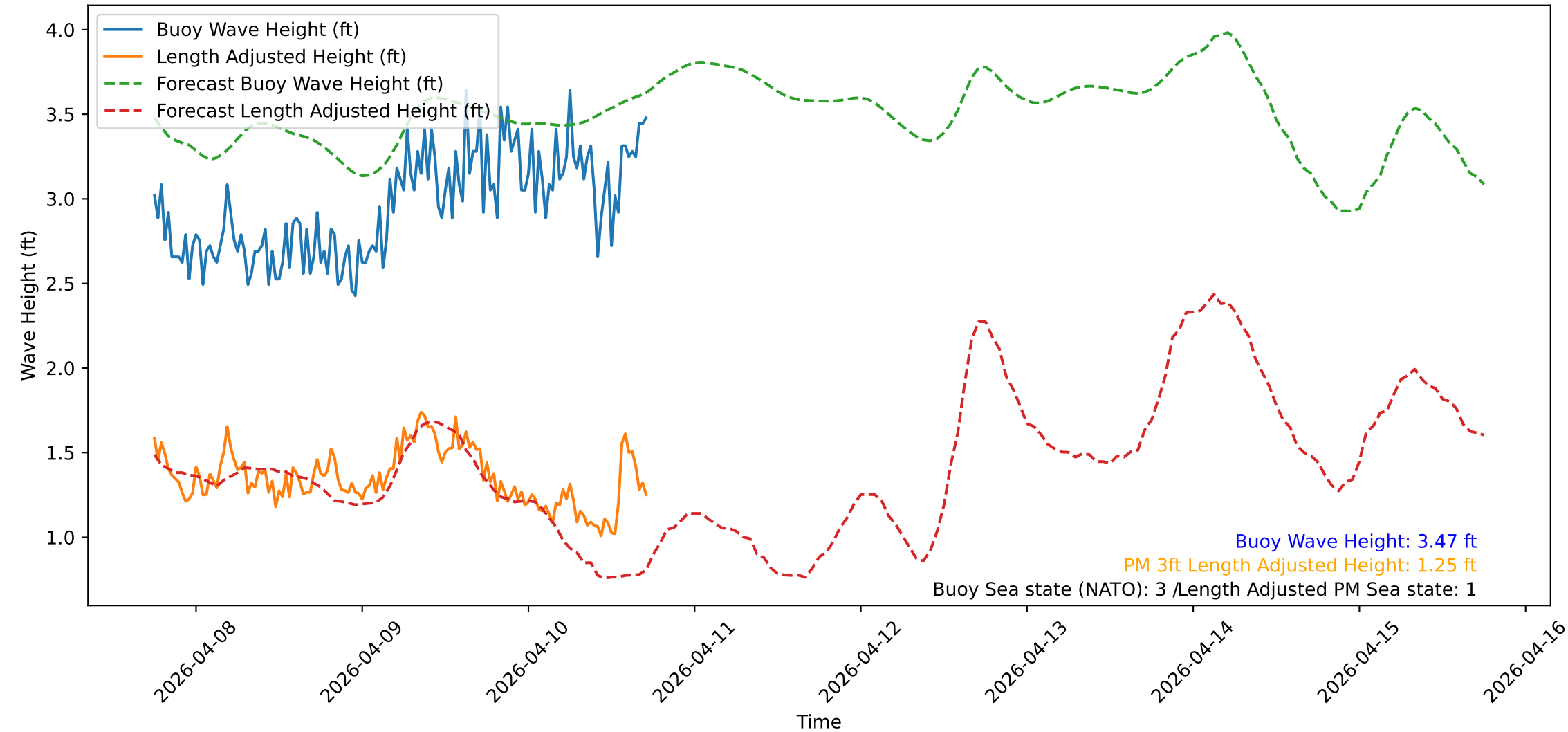
Wave Heights over Time for Oceanside Harbor at 2026-04-10 18:00:31
