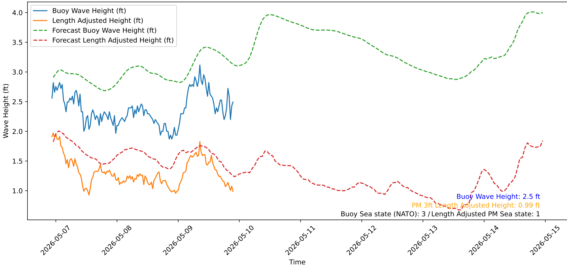
Wave Heights over Time for Oceanside Harbor at 2026-05-09 22:40:31
