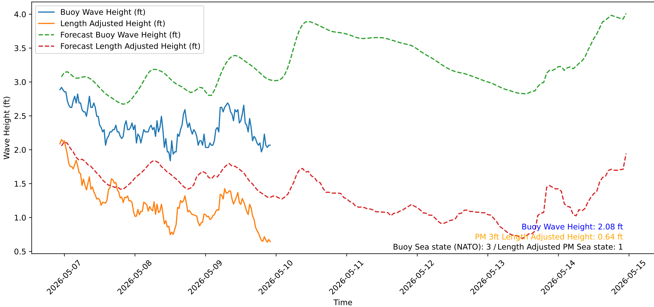
Wave Heights over Time for Green Beach at 2026-05-09 22:41:14
