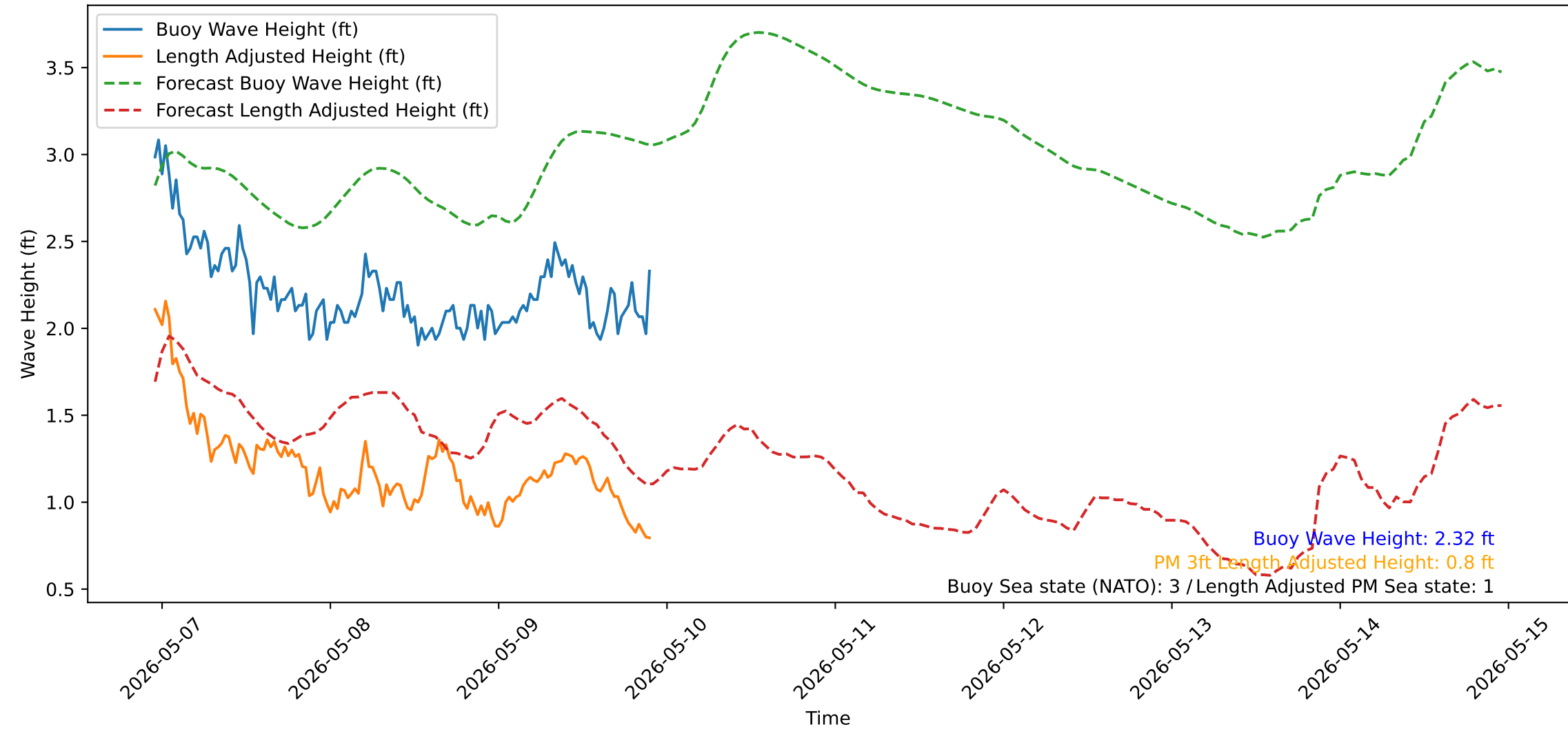
Wave Heights over Time for Red Beach at 2026-05-09 22:40:51
