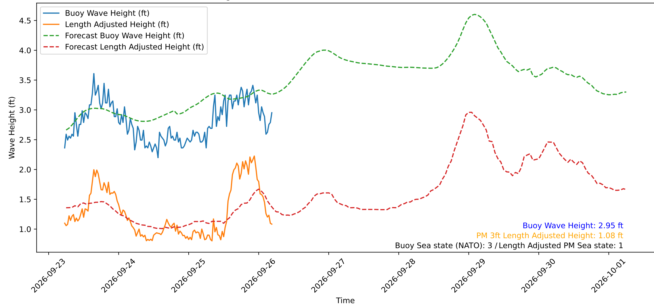
Wave Heights over Time for Oceanside Harbor at 2026-09-26 05:30:30
