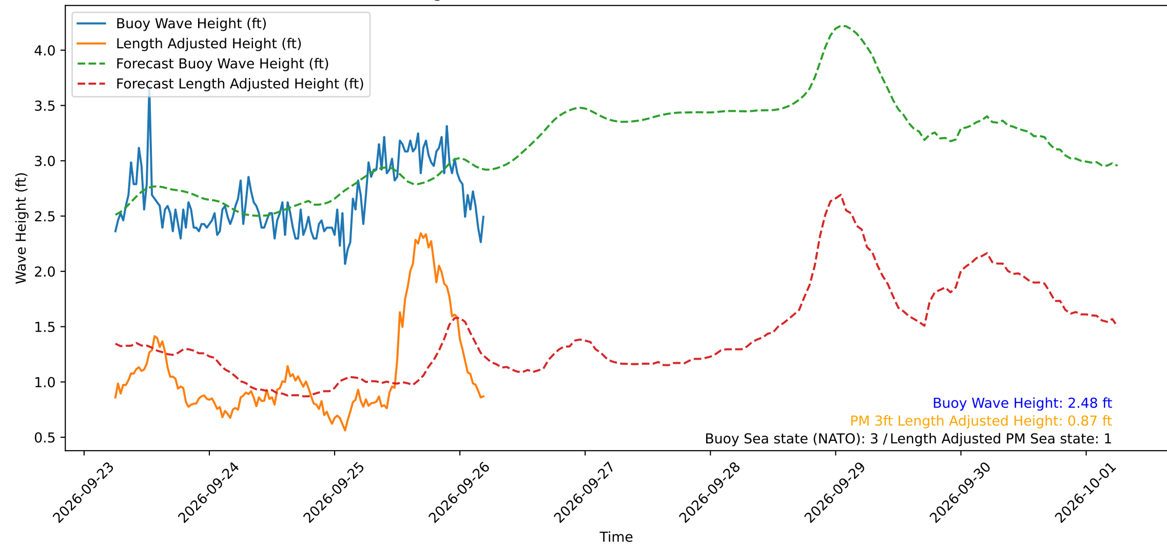
Wave Heights over Time for Red Beach at 2026-09-26 05:30:49
