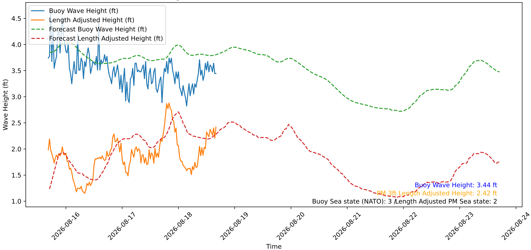
Wave Heights over Time for Oceanside Harbor at 2026-08-18 16:30:26
