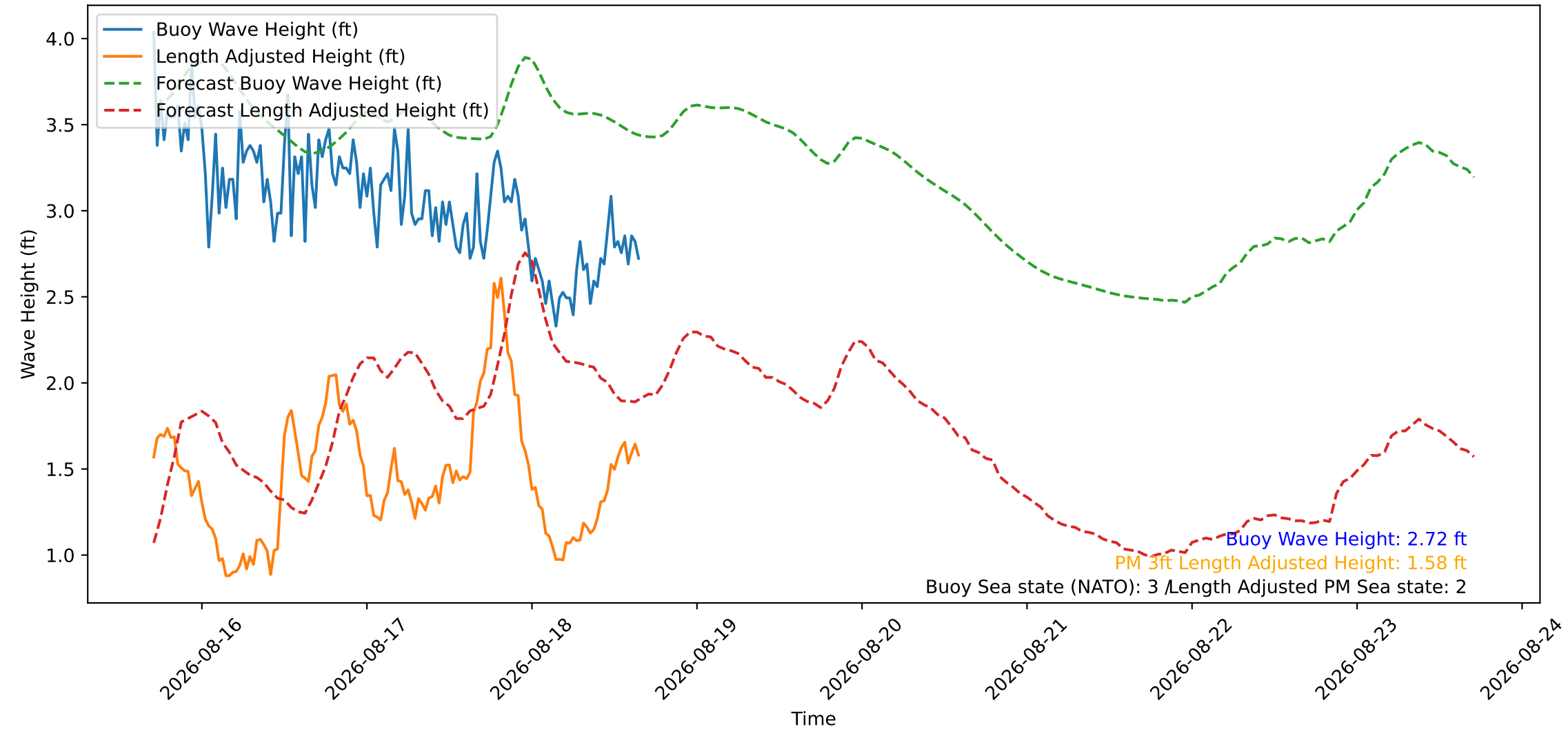
Wave Heights over Time for Red Beach at 2026-08-18 16:30:46
