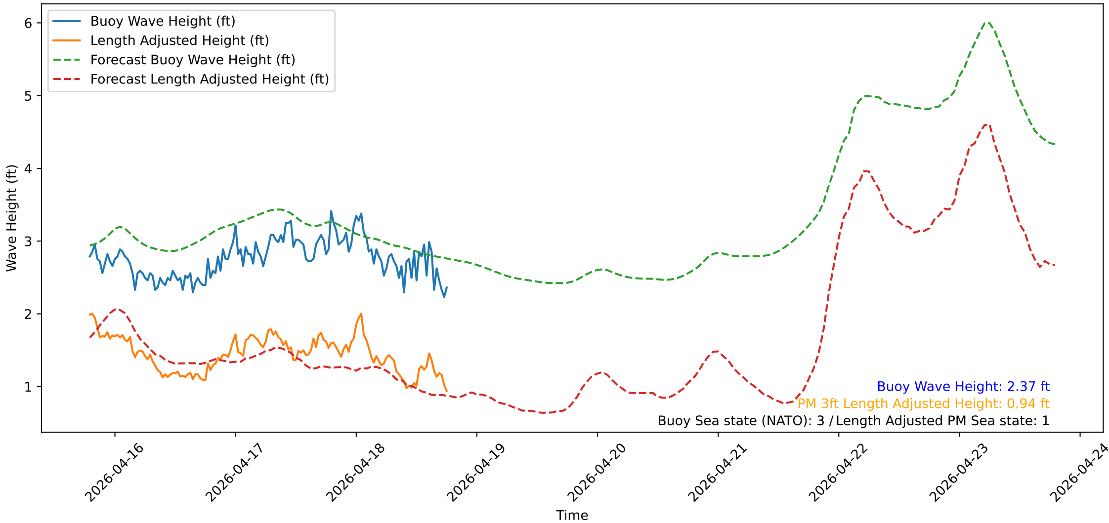
Wave Heights over Time for Oceanside Harbor at 2026-04-18 19:00:31
