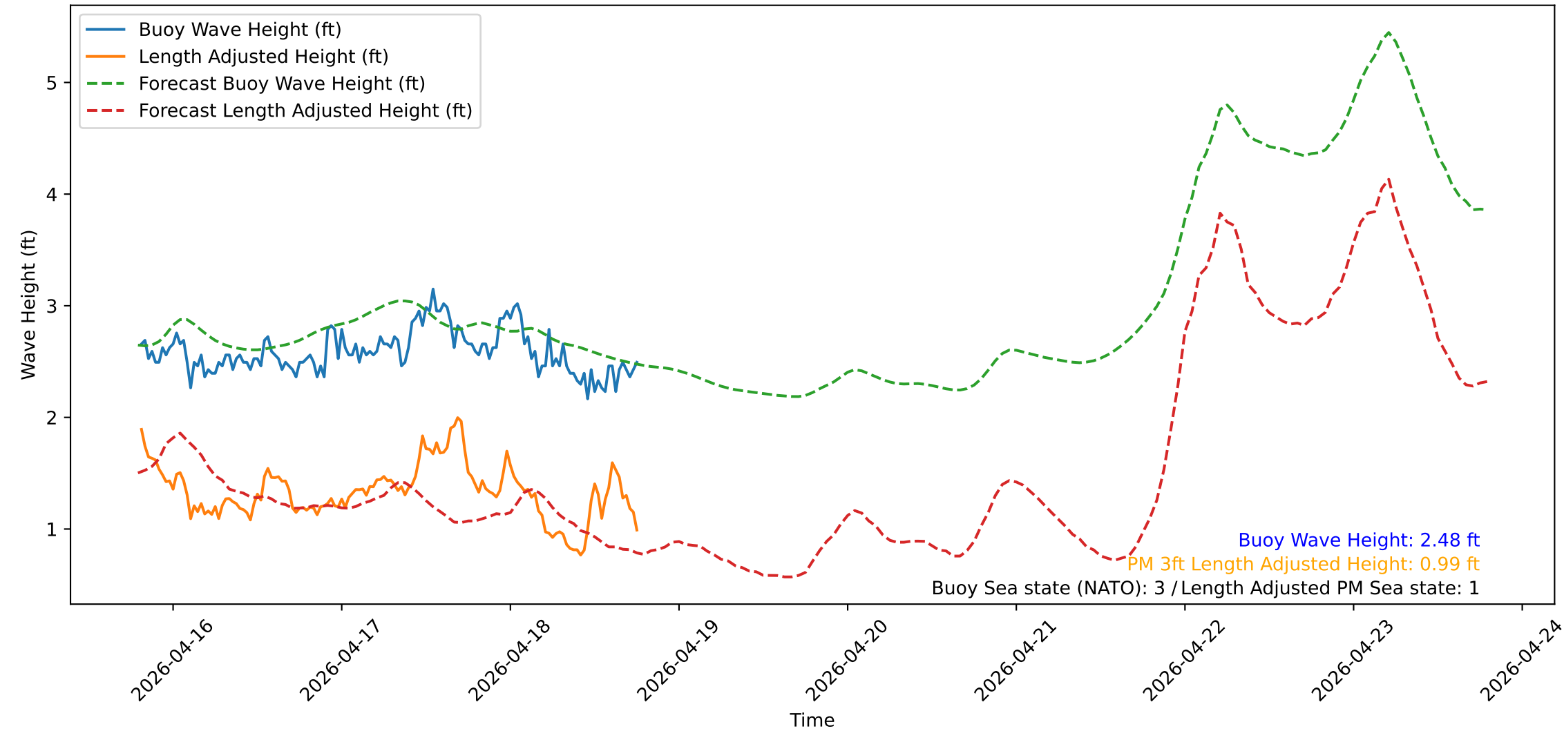
Wave Heights over Time for Red Beach at 2026-04-18 19:00:51
