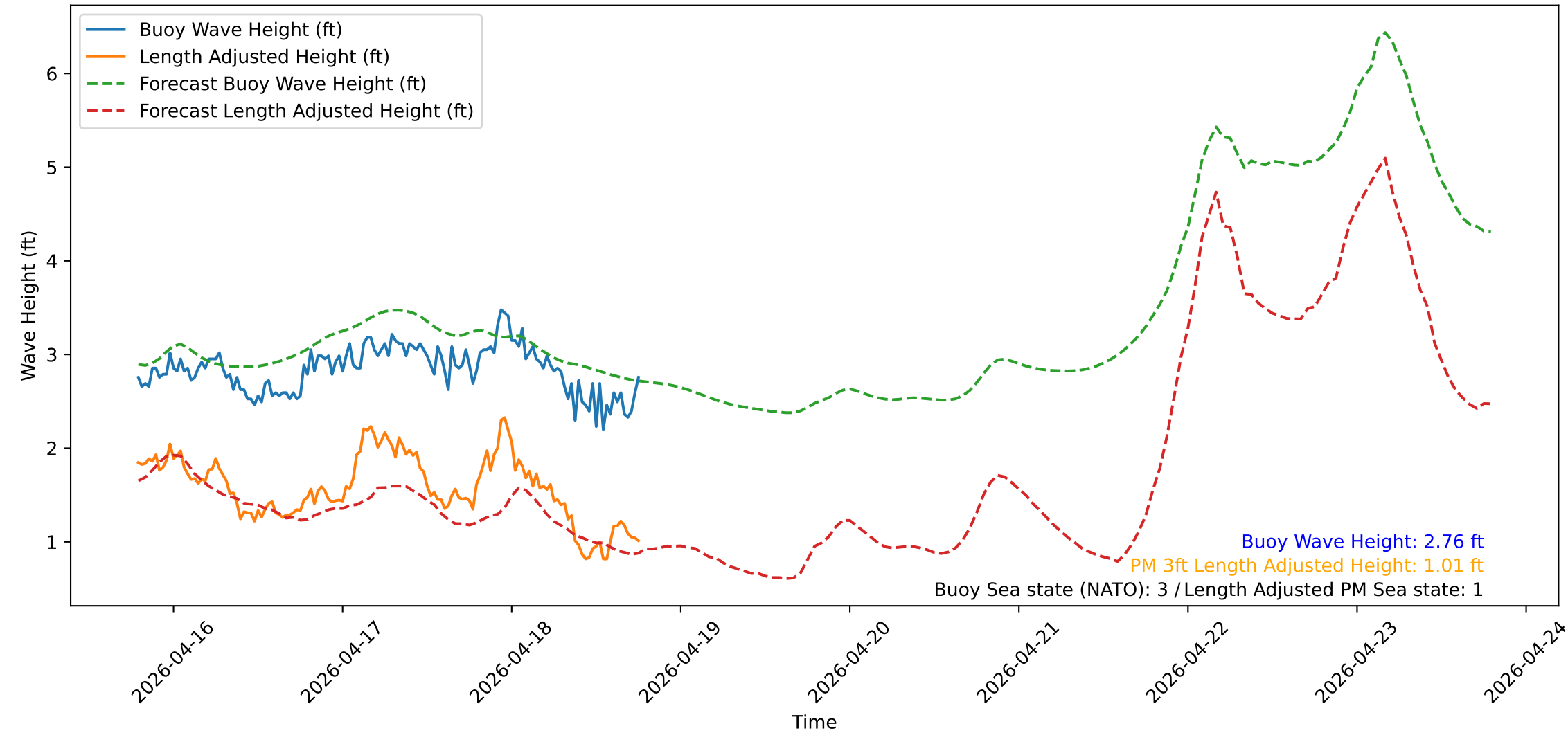
Wave Heights over Time for Green Beach at 2026-04-18 19:01:15
