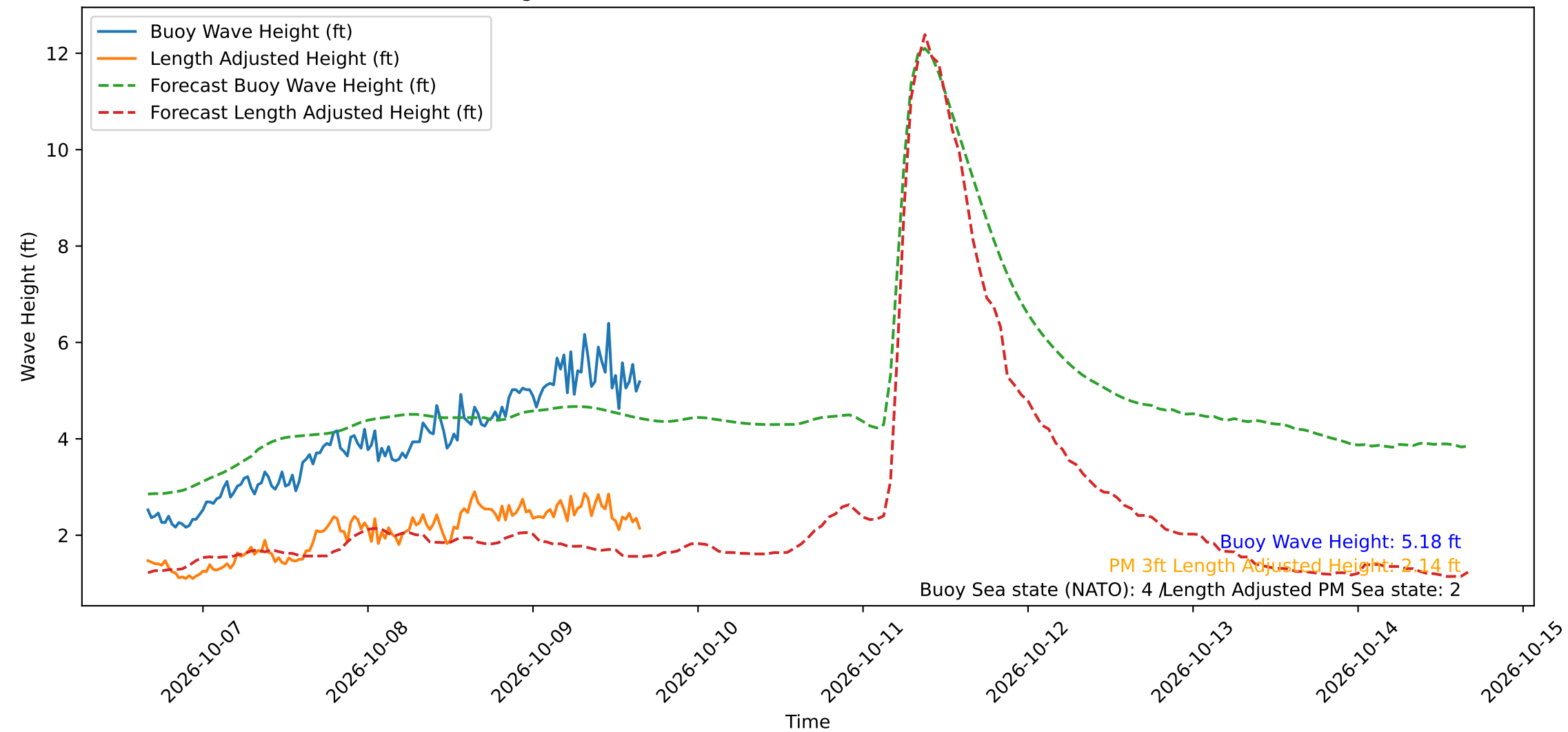
Wave Heights over Time for Oceanside Harbor at 2026-10-09 16:10:30
