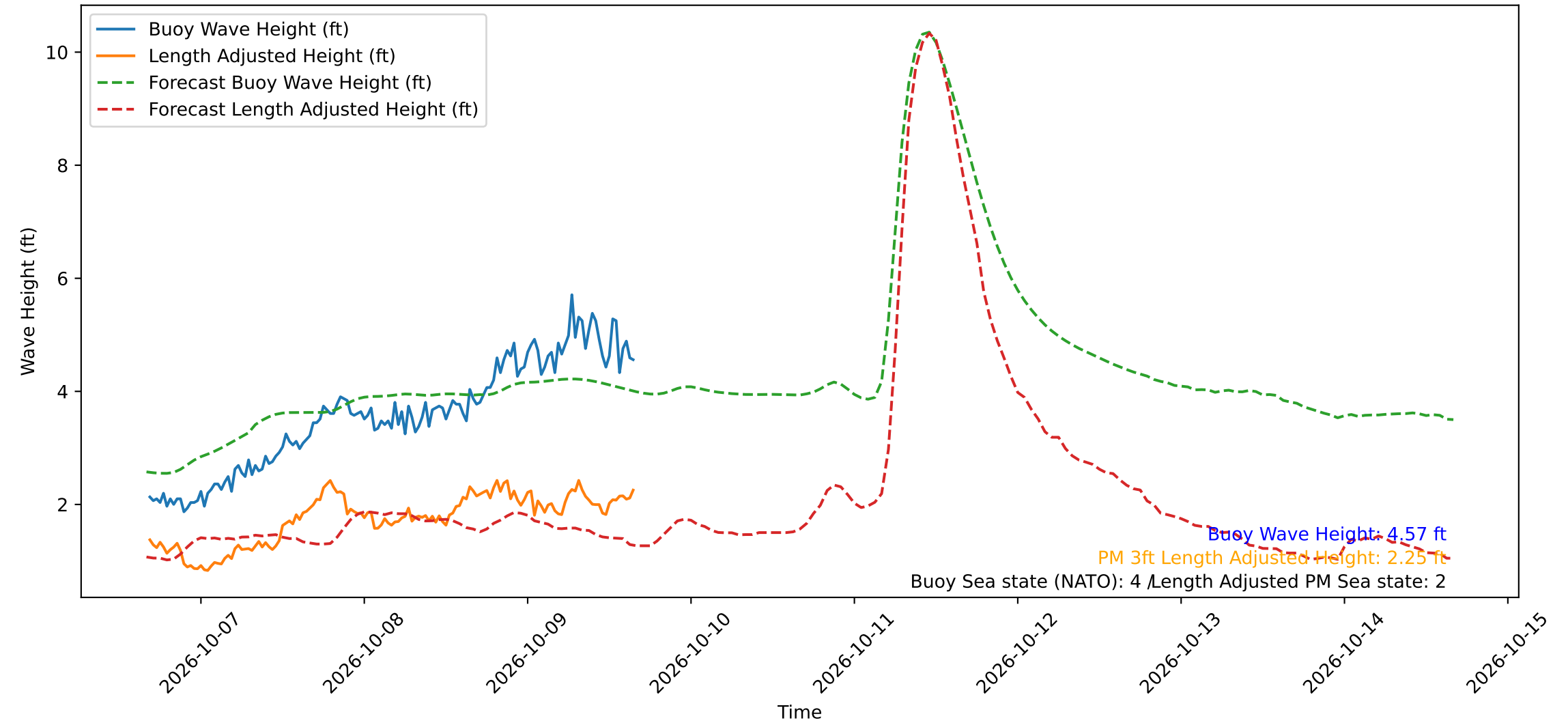
Wave Heights over Time for Red Beach at 2026-10-09 16:10:49
