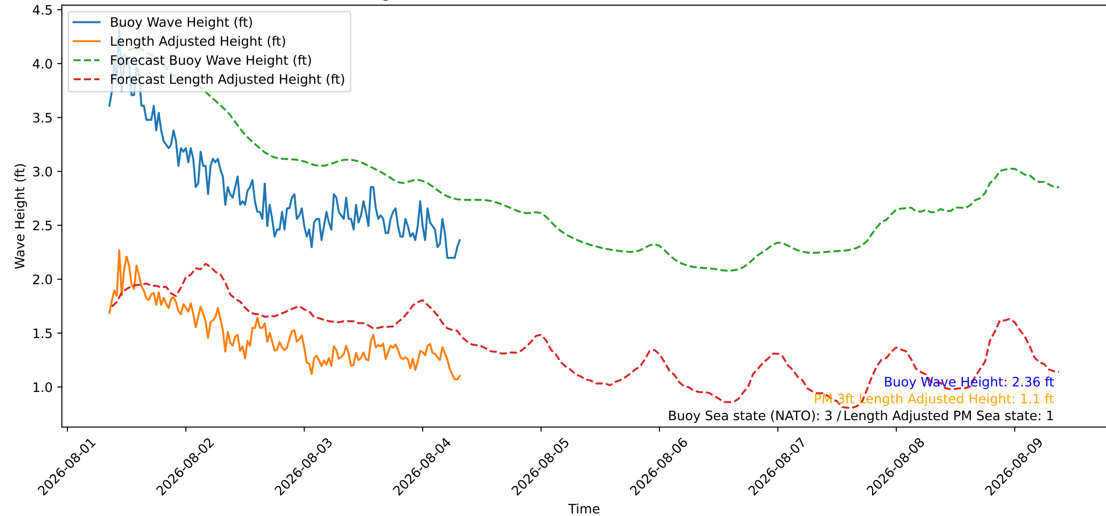
Wave Heights over Time for Oceanside Harbor at 2026-08-04 08:30:26
