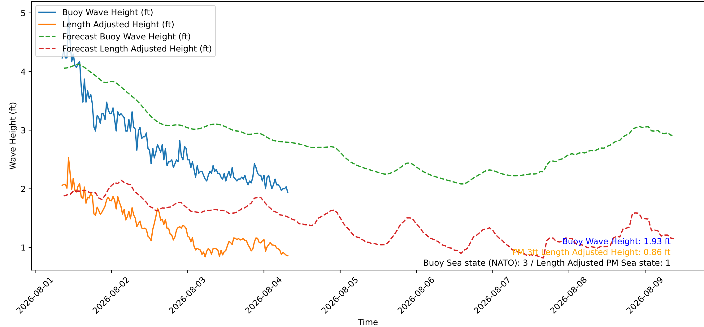
Wave Heights over Time for Green Beach at 2026-08-04 08:31:09
