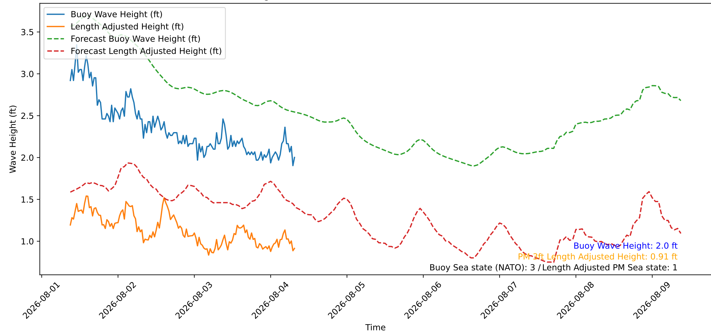
Wave Heights over Time for Red Beach at 2026-08-04 08:30:46
