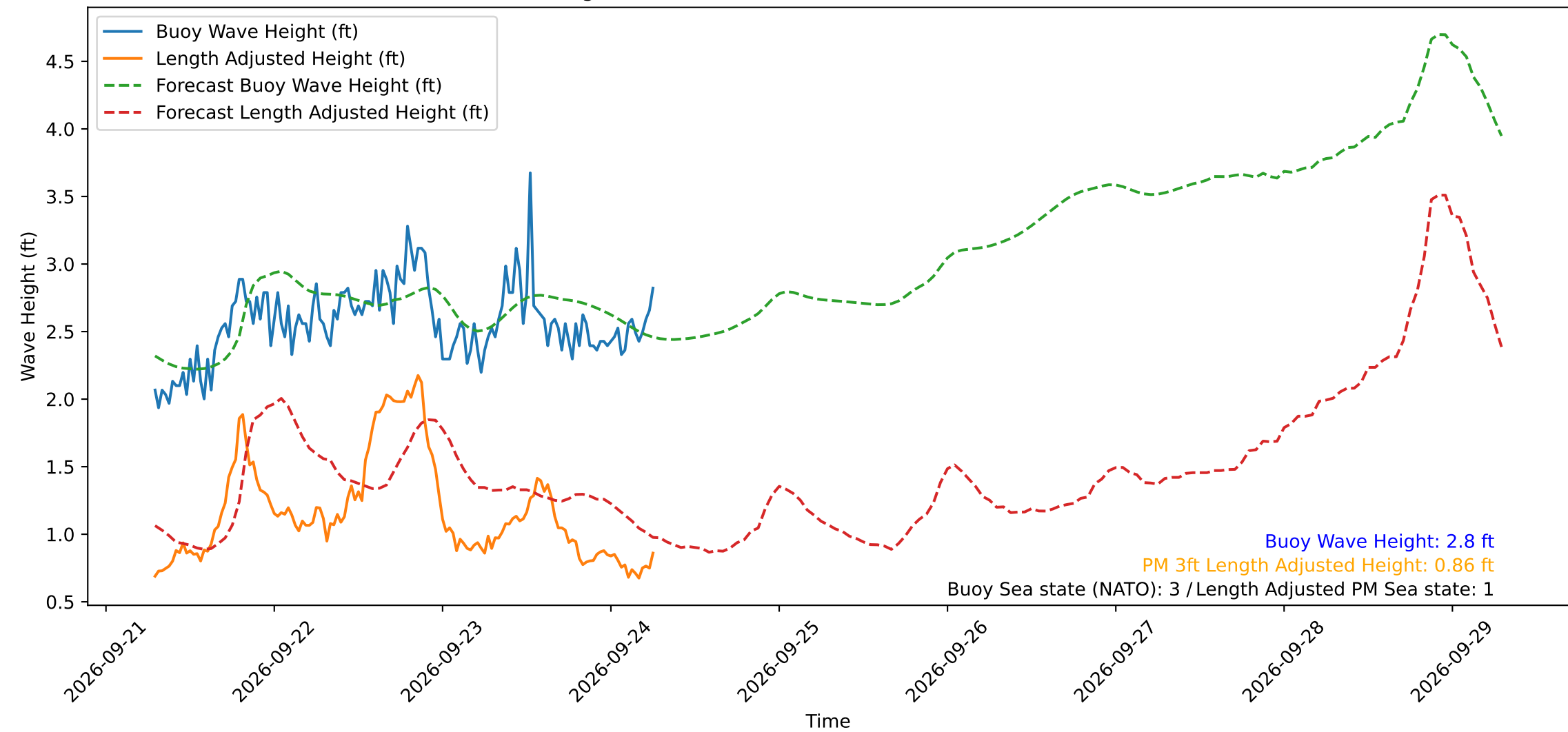
Wave Heights over Time for Red Beach at 2026-09-24 06:40:49
