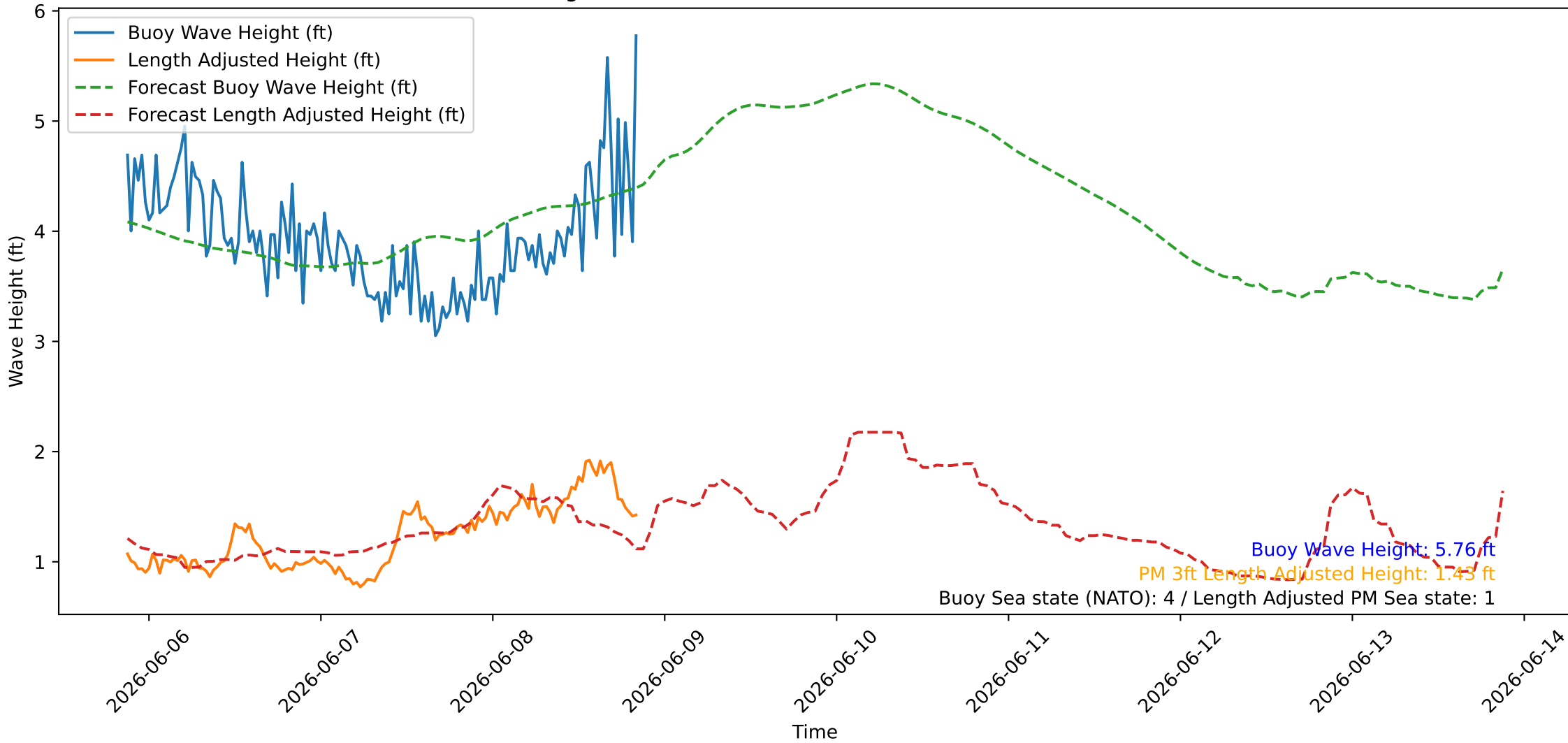
Wave Heights over Time for Red Beach at 2026-06-08 20:40:46
