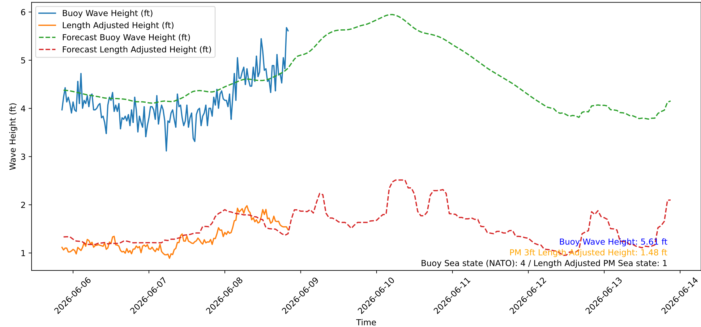
Wave Heights over Time for Green Beach at 2026-06-08 20:41:08
