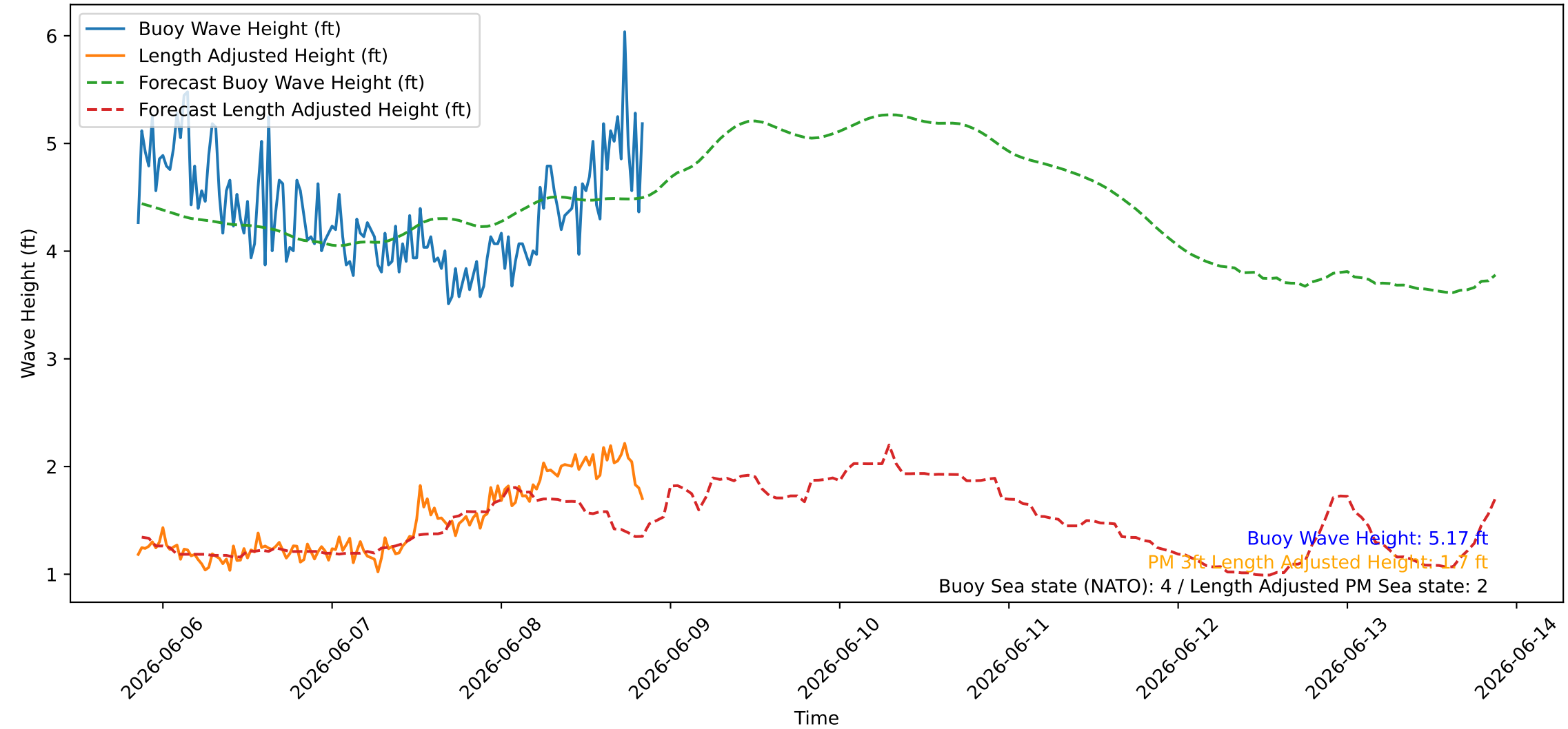
Wave Heights over Time for Oceanside Harbor at 2026-06-08 20:40:26
