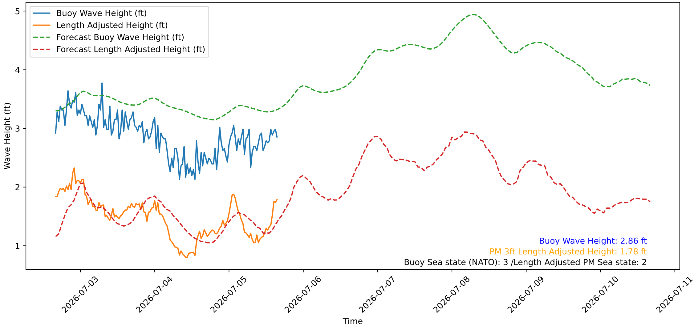
Wave Heights over Time for Oceanside Harbor at 2026-07-05 16:10:27
