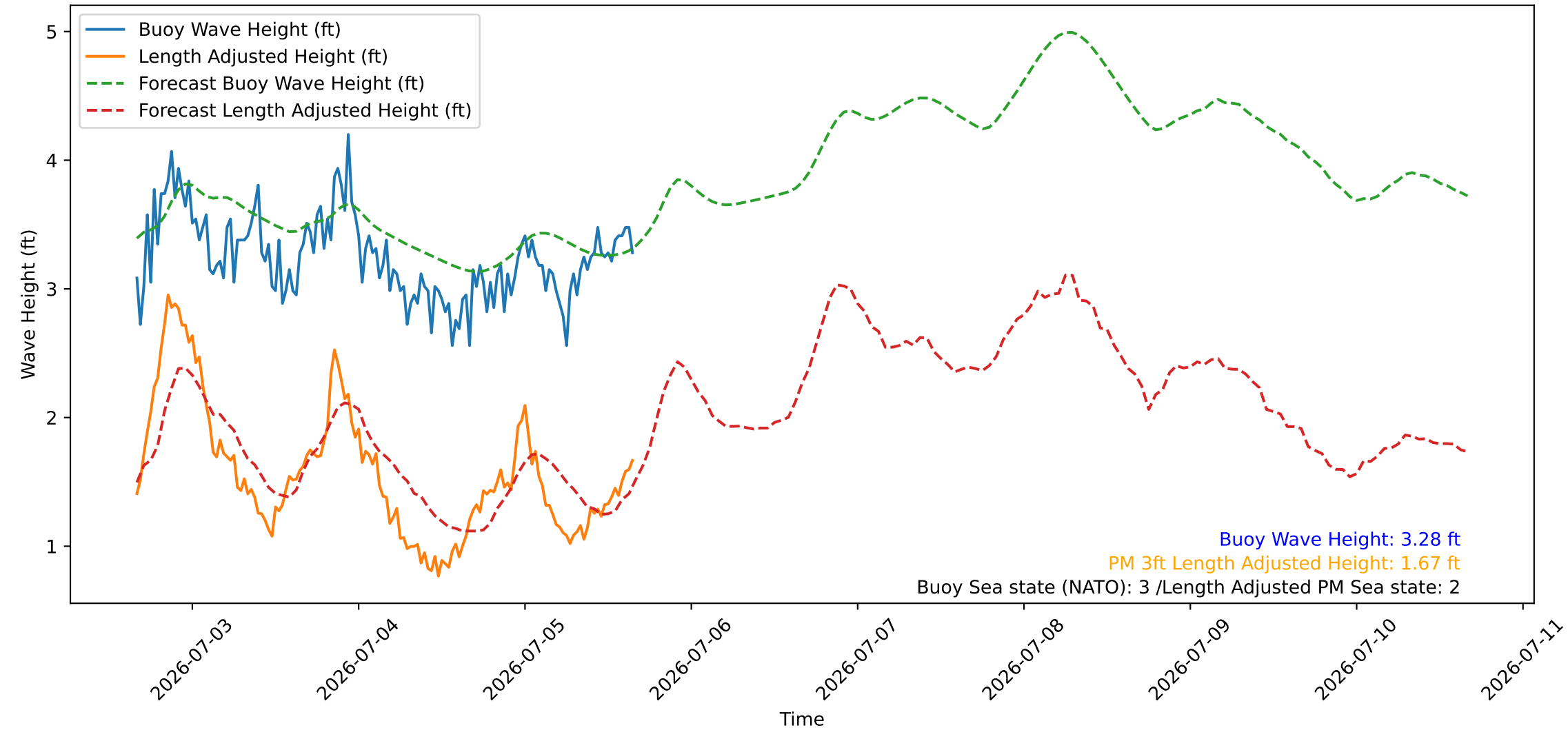
Wave Heights over Time for Green Beach at 2026-07-05 16:11:09
