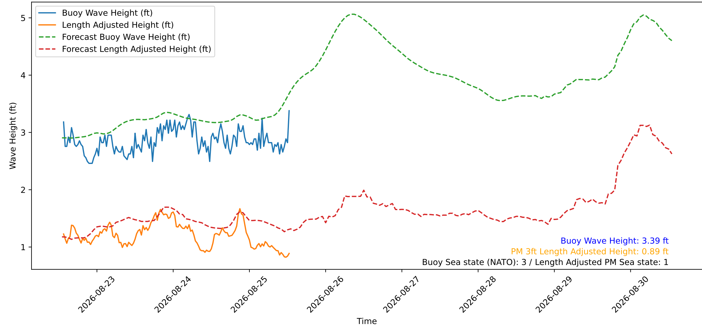
Wave Heights over Time for Green Beach at 2026-08-25 13:11:12
