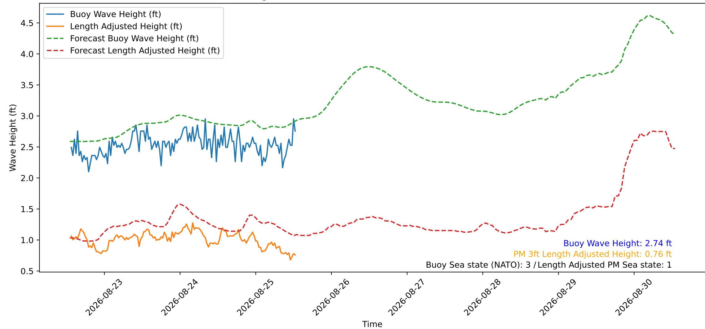
Wave Heights over Time for Red Beach at 2026-08-25 13:10:49
