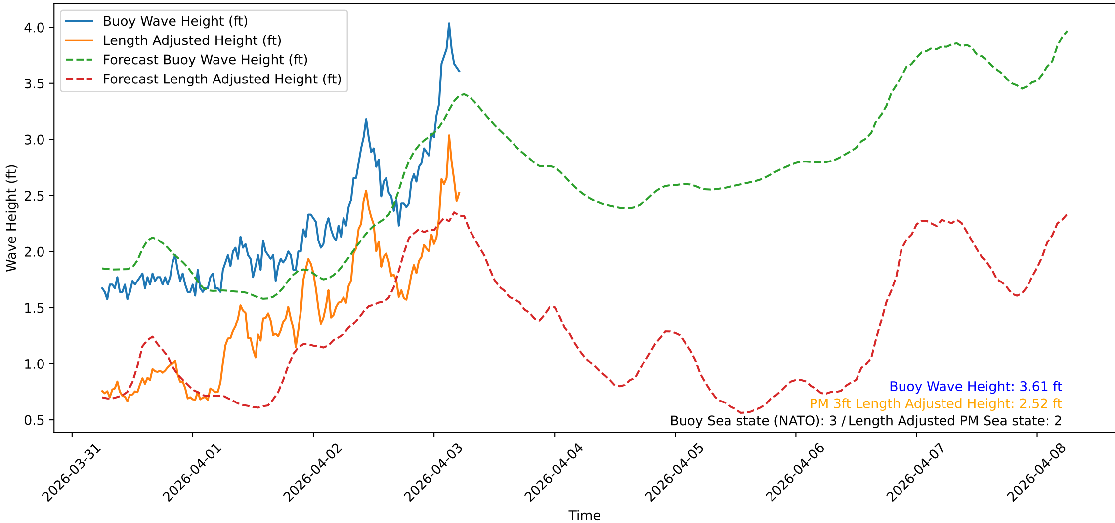
Wave Heights over Time for Oceanside Harbor at 2026-04-03 06:10:31
