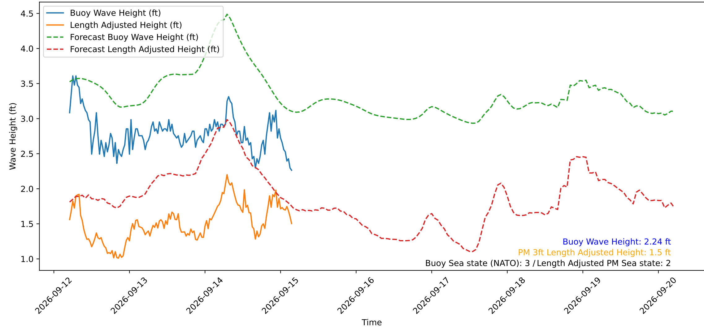
Wave Heights over Time for Green Beach at 2026-09-15 04:31:12
