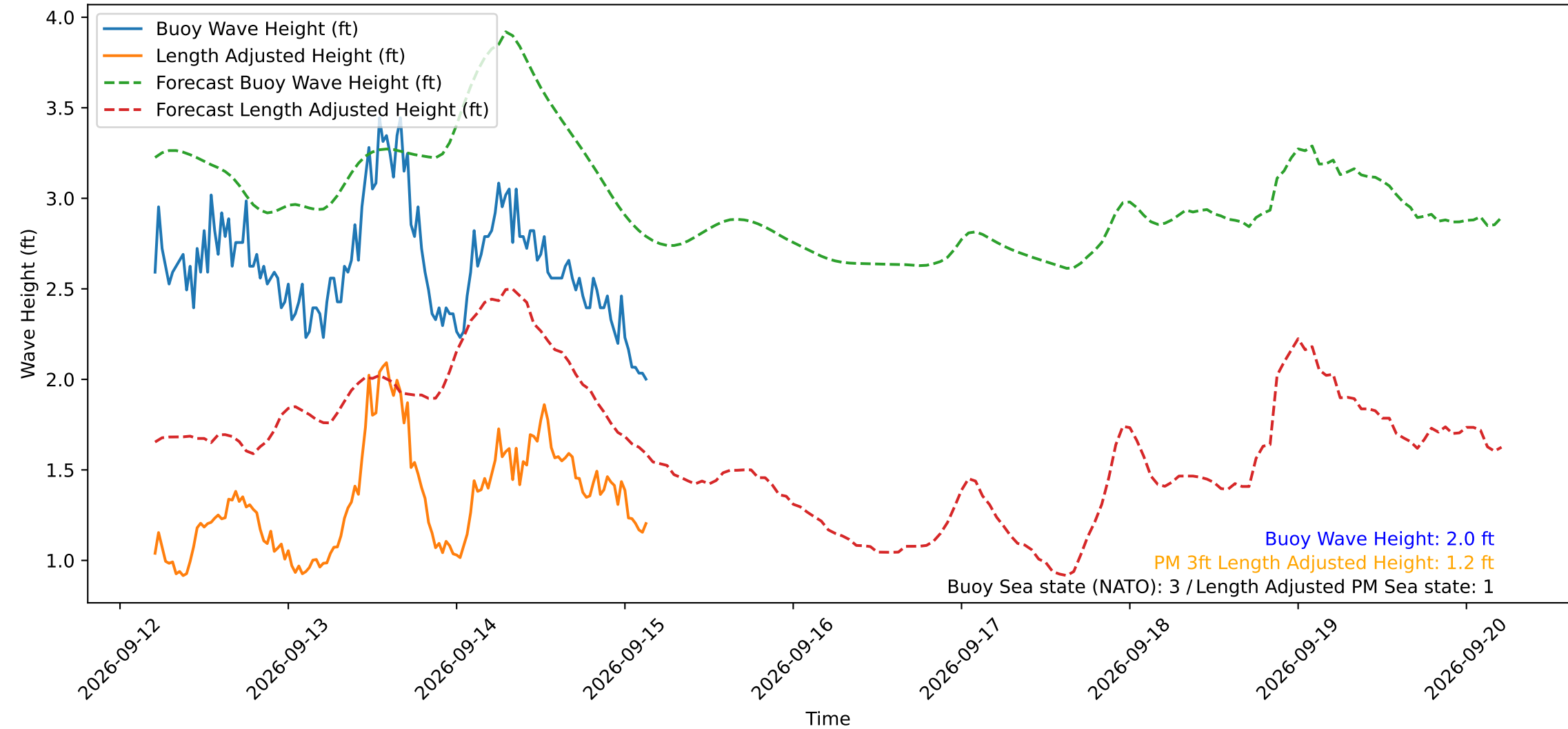
Wave Heights over Time for Red Beach at 2026-09-15 04:30:49
