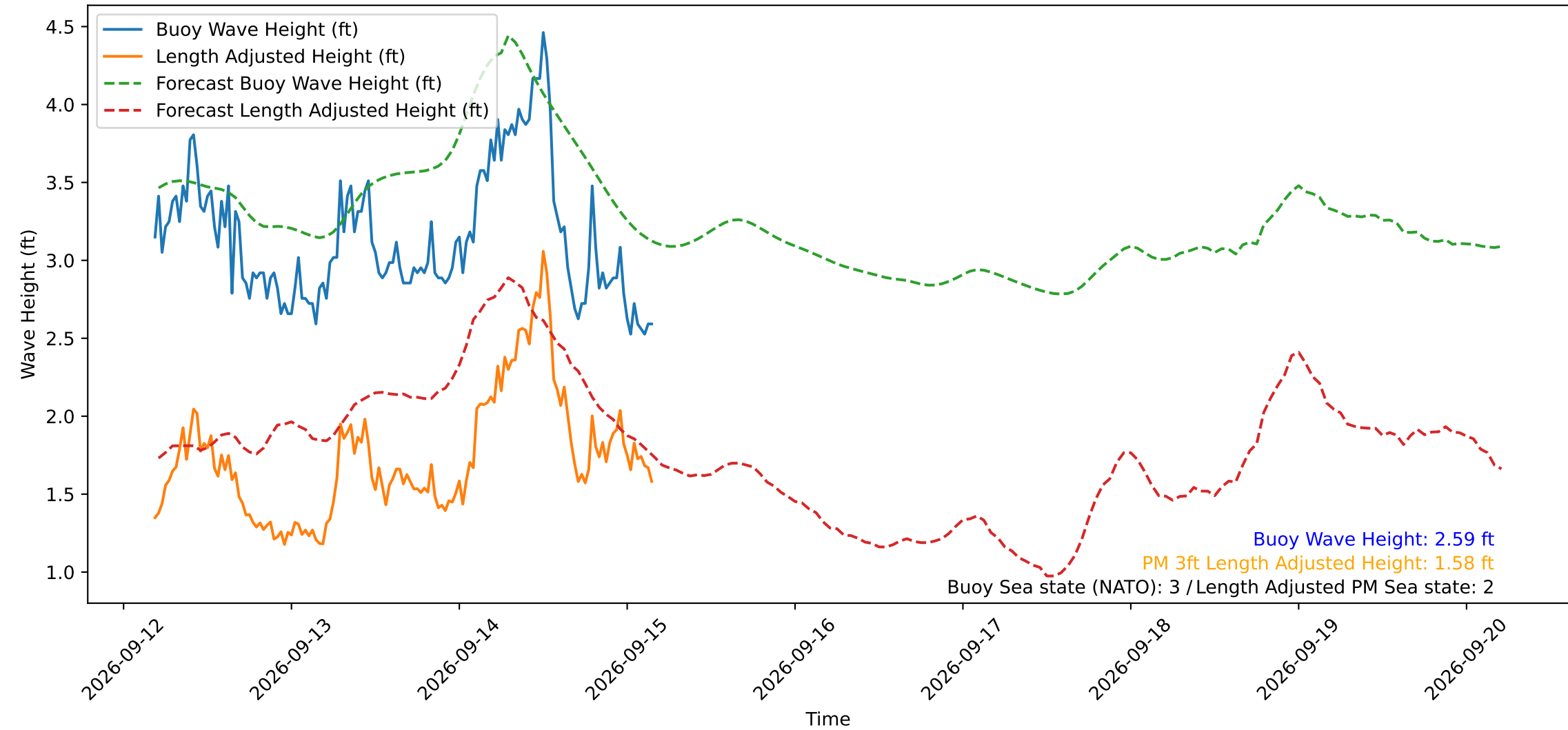
Wave Heights over Time for Oceanside Harbor at 2026-09-15 04:30:30
