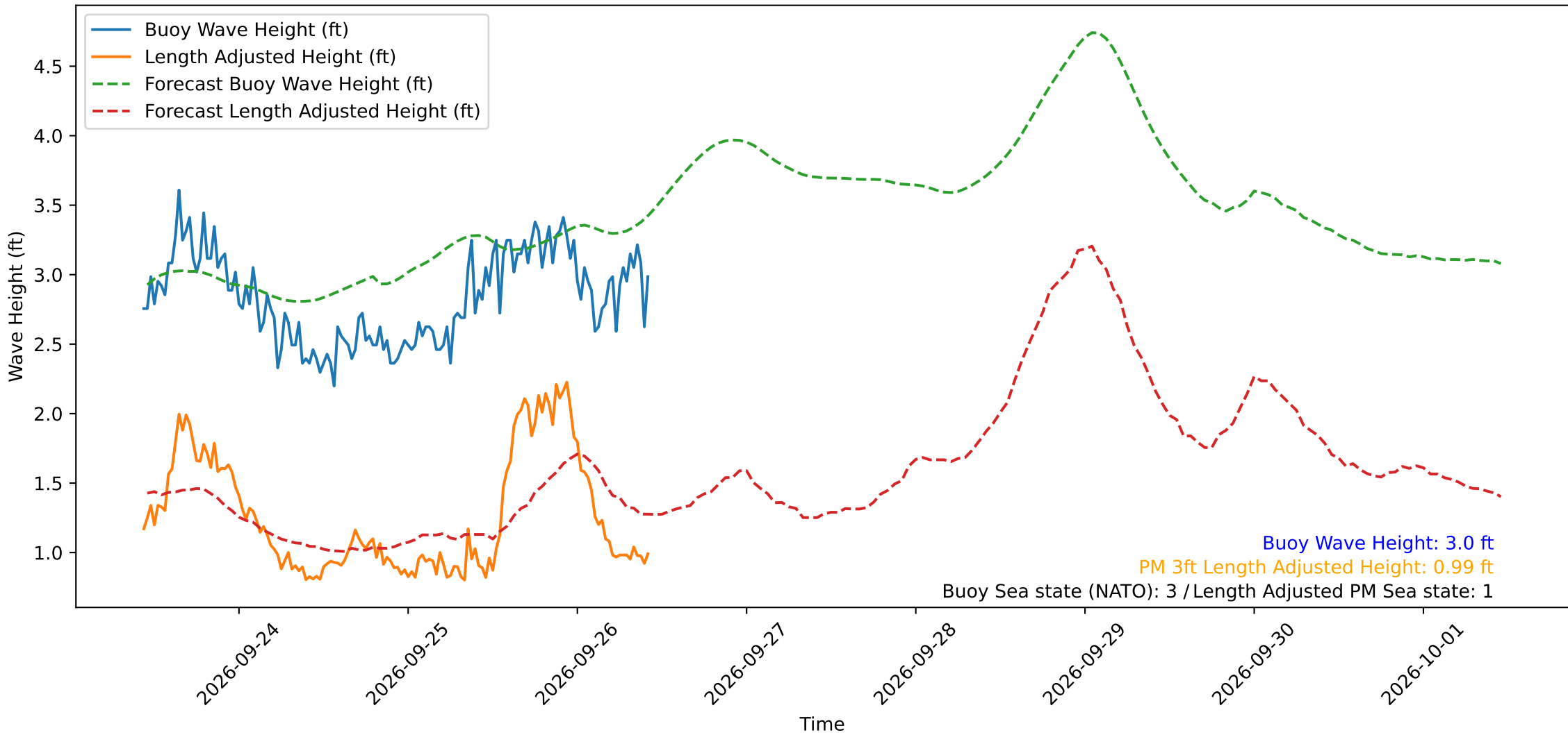
Wave Heights over Time for Oceanside Harbor at 2026-09-26 10:40:30
