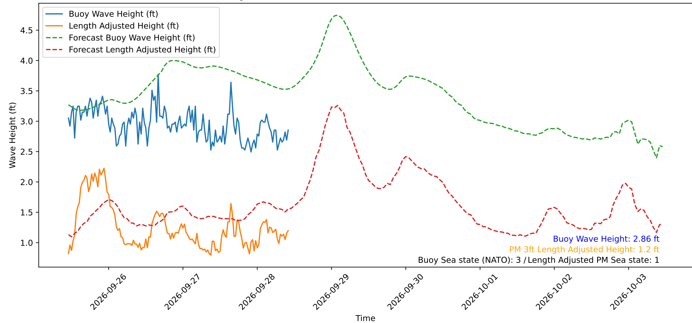
Wave Heights over Time for Oceanside Harbor at 2026-09-28 10:50:30
