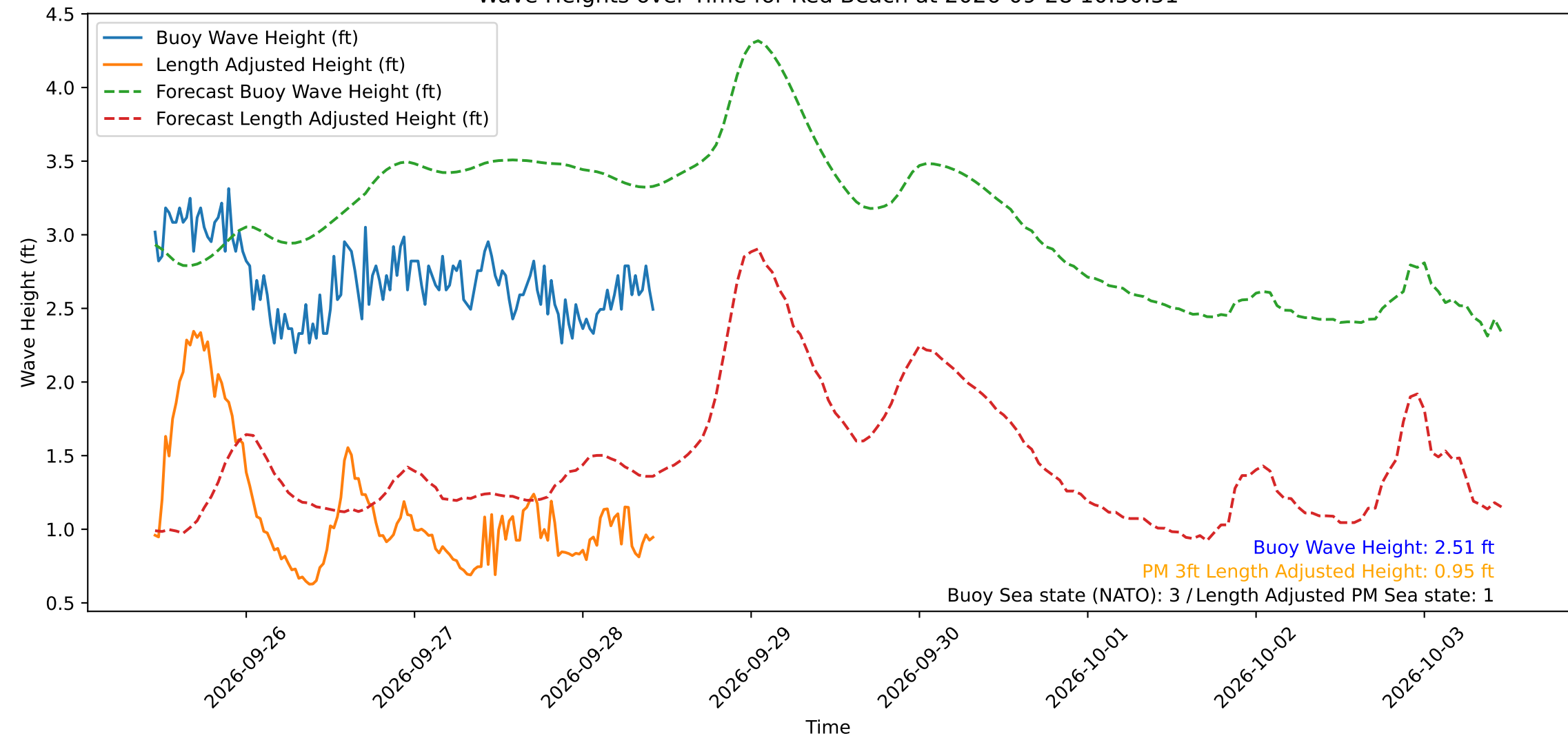
Wave Heights over Time for Red Beach at 2026-09-28 10:50:51
