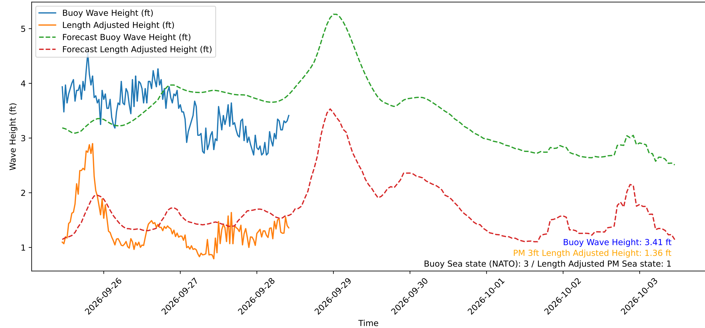
Wave Heights over Time for Green Beach at 2026-09-28 10:51:14
