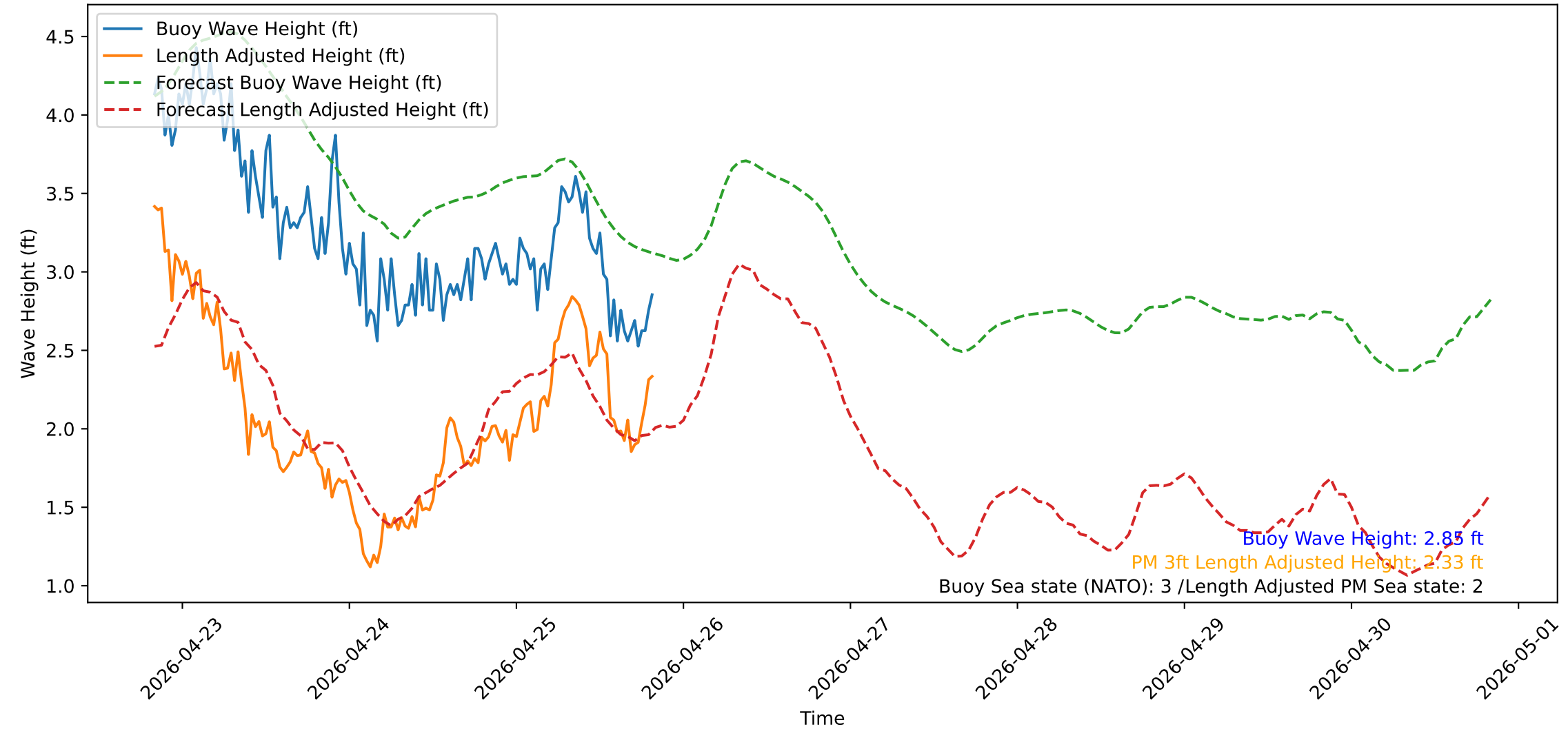
Wave Heights over Time for Oceanside Harbor at 2026-04-25 20:00:31
