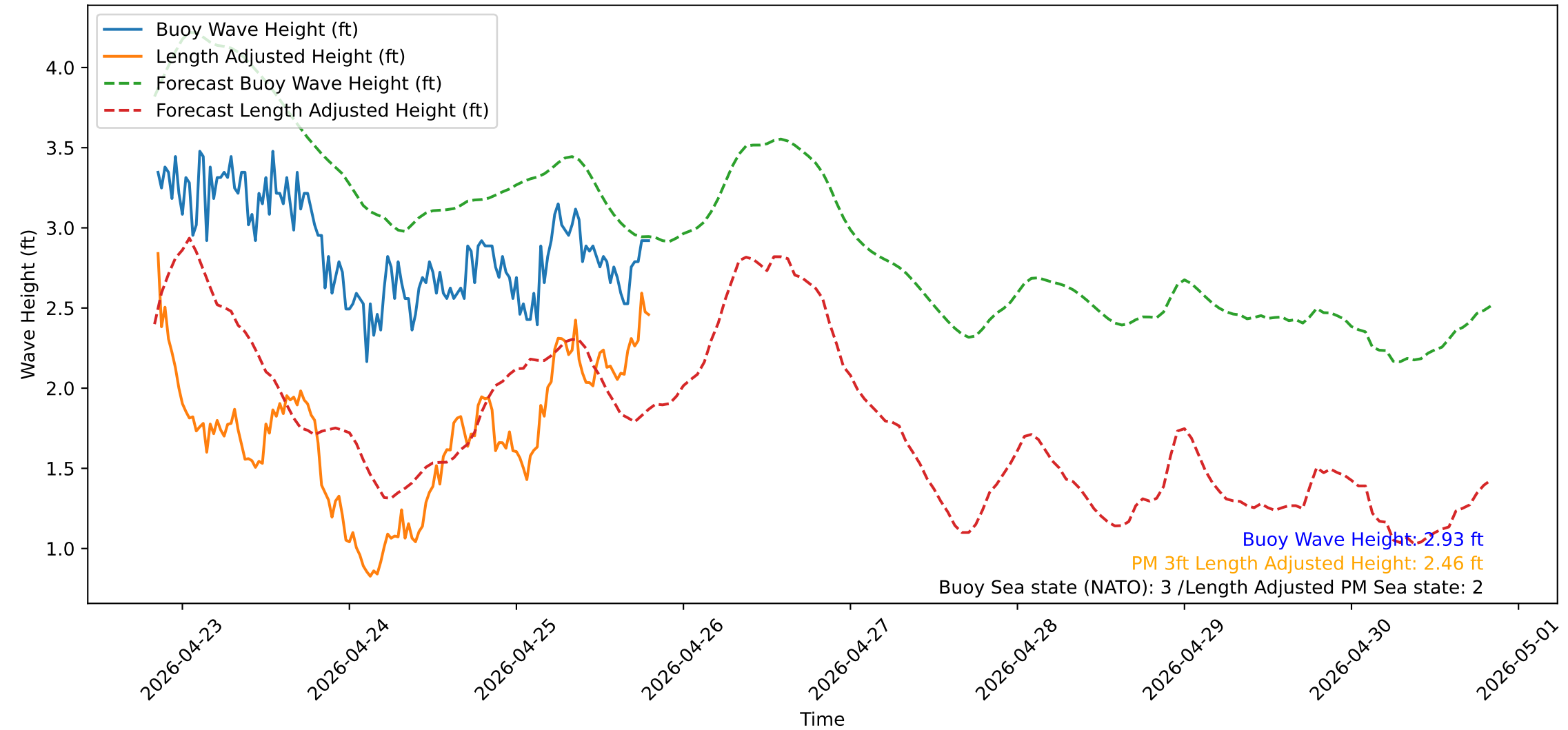
Wave Heights over Time for Red Beach at 2026-04-25 20:00:50
