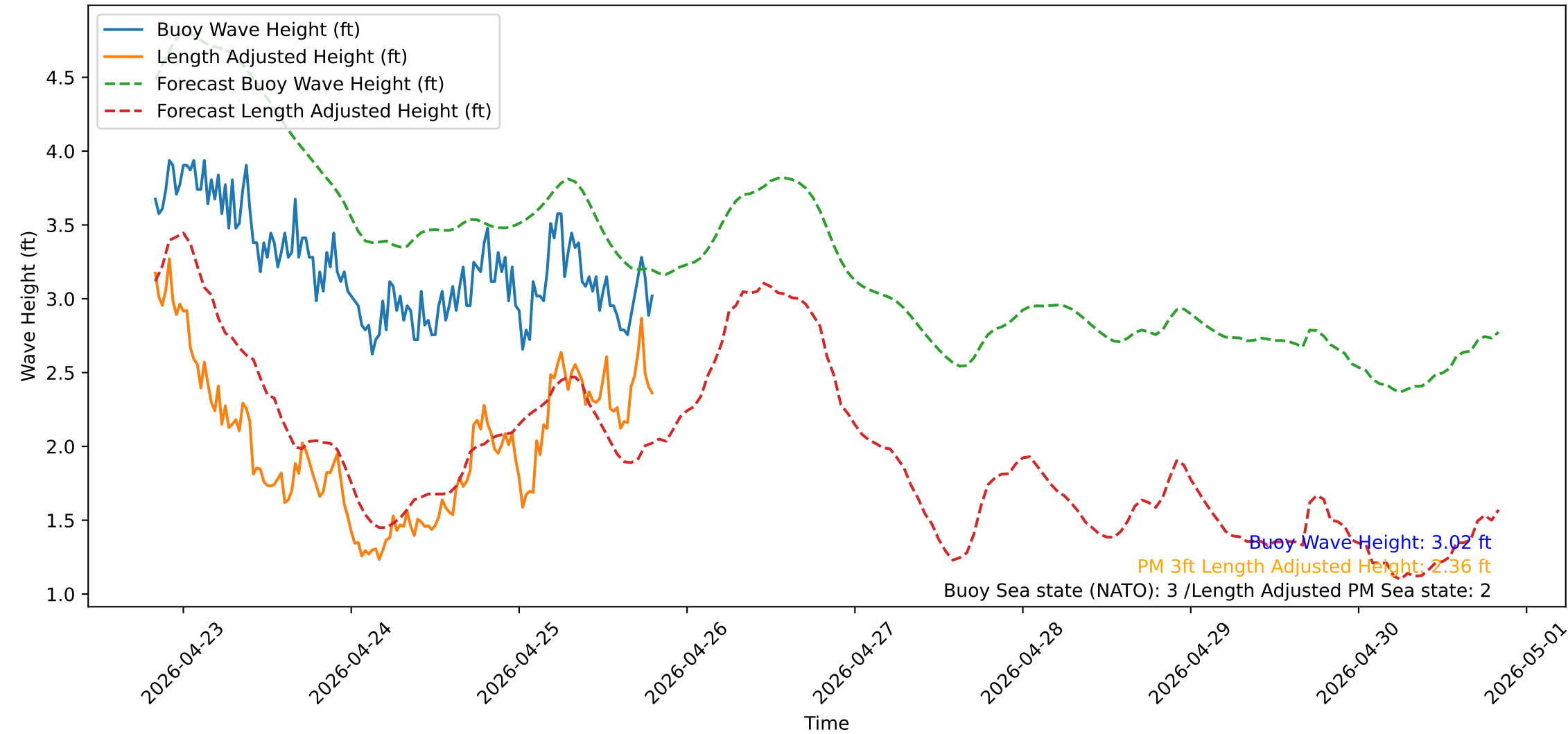
Wave Heights over Time for Green Beach at 2026-04-25 20:01:12
