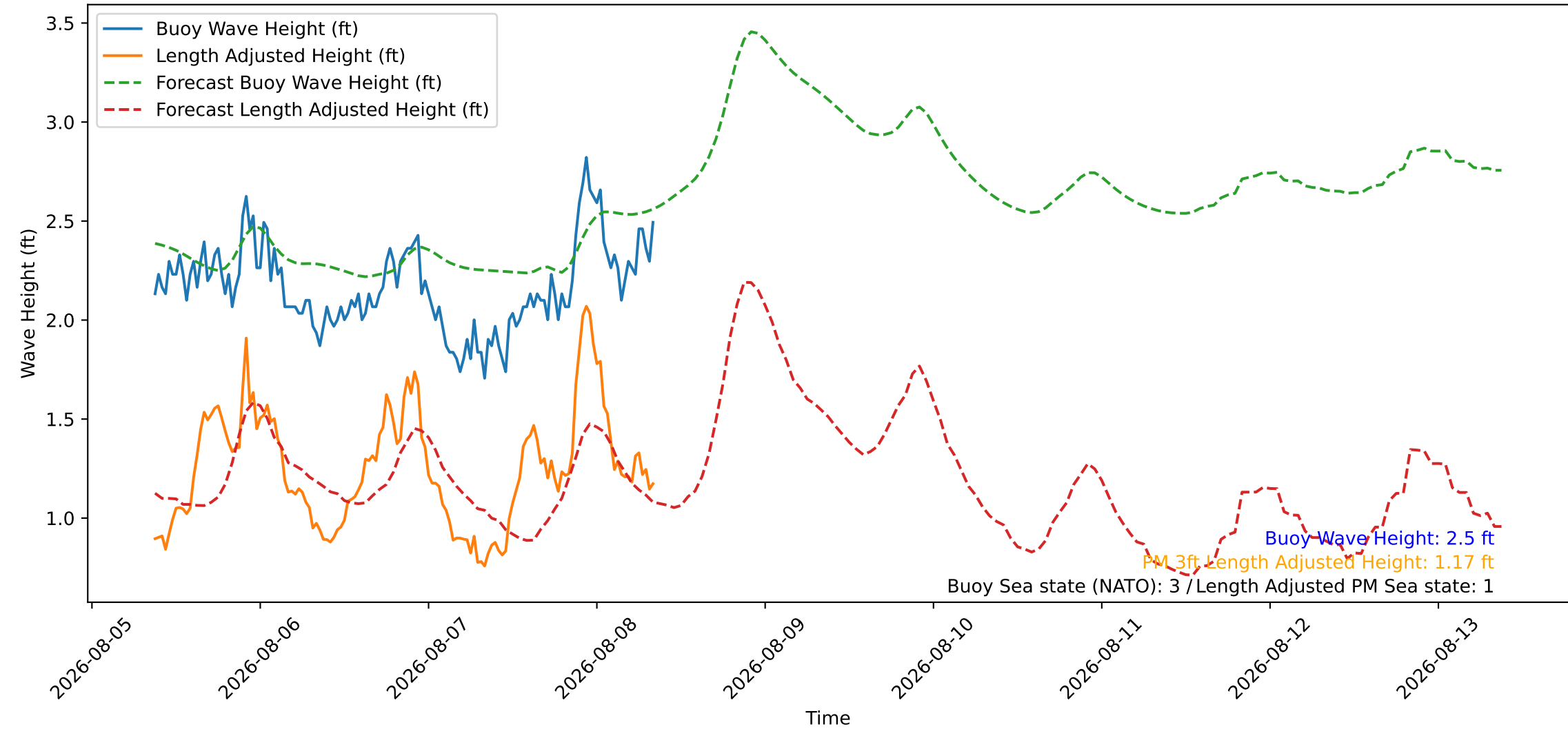
Wave Heights over Time for Green Beach at 2026-08-08 08:51:09
