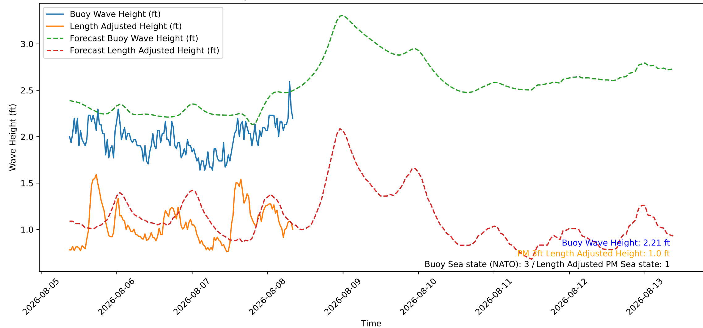
Wave Heights over Time for Oceanside Harbor at 2026-08-08 08:50:26
