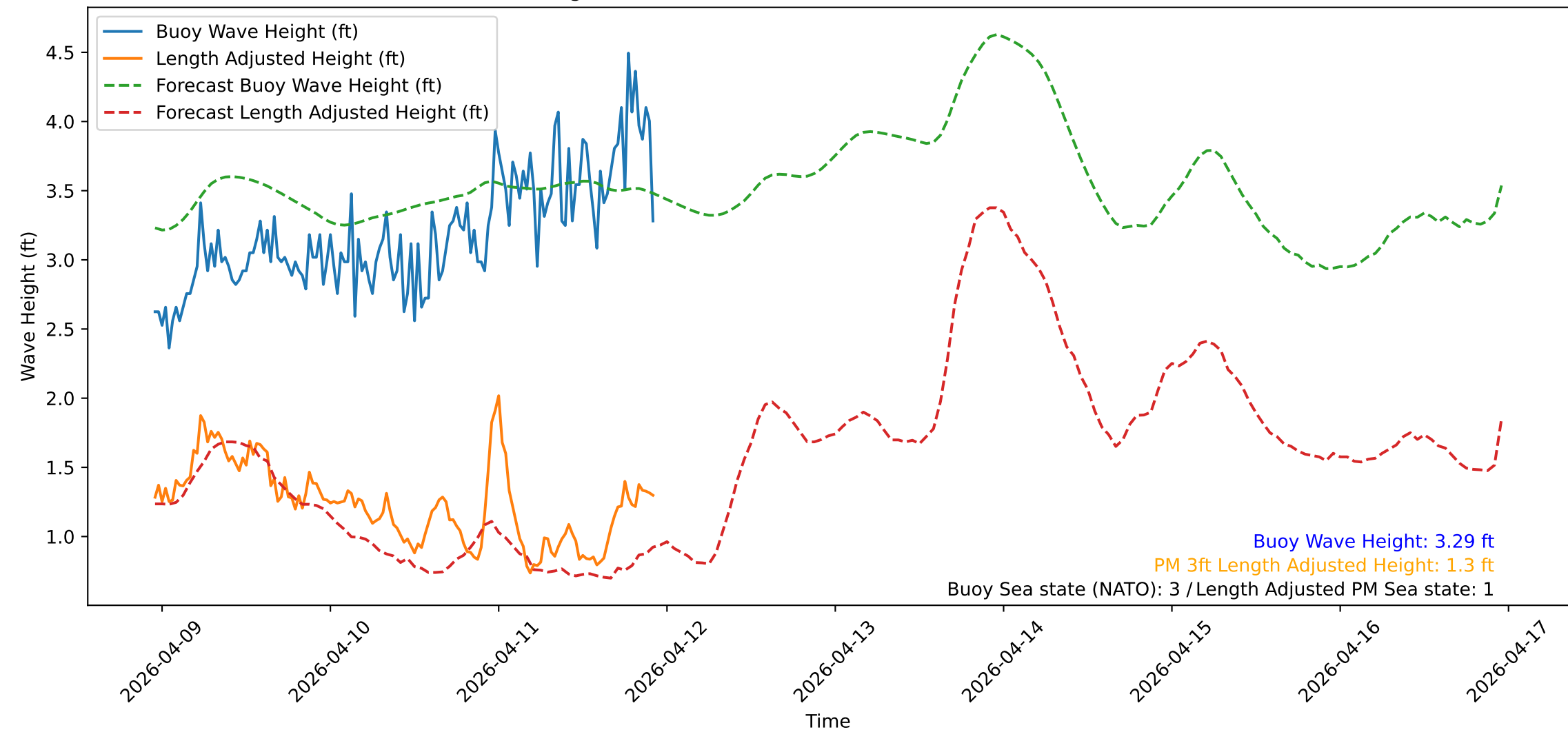
Wave Heights over Time for Green Beach at 2026-04-11 22:51:14
