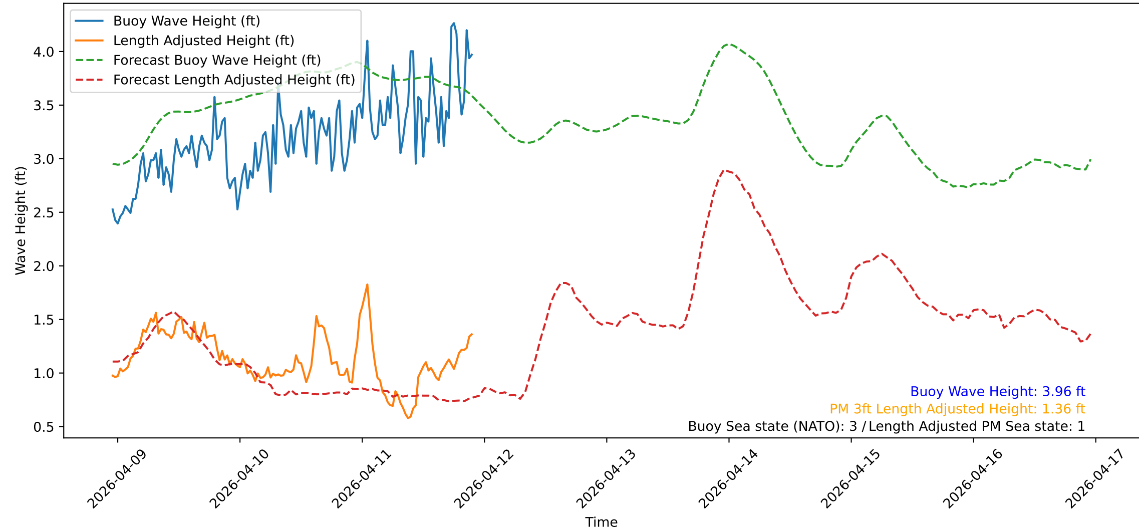
Wave Heights over Time for Red Beach at 2026-04-11 22:50:52
