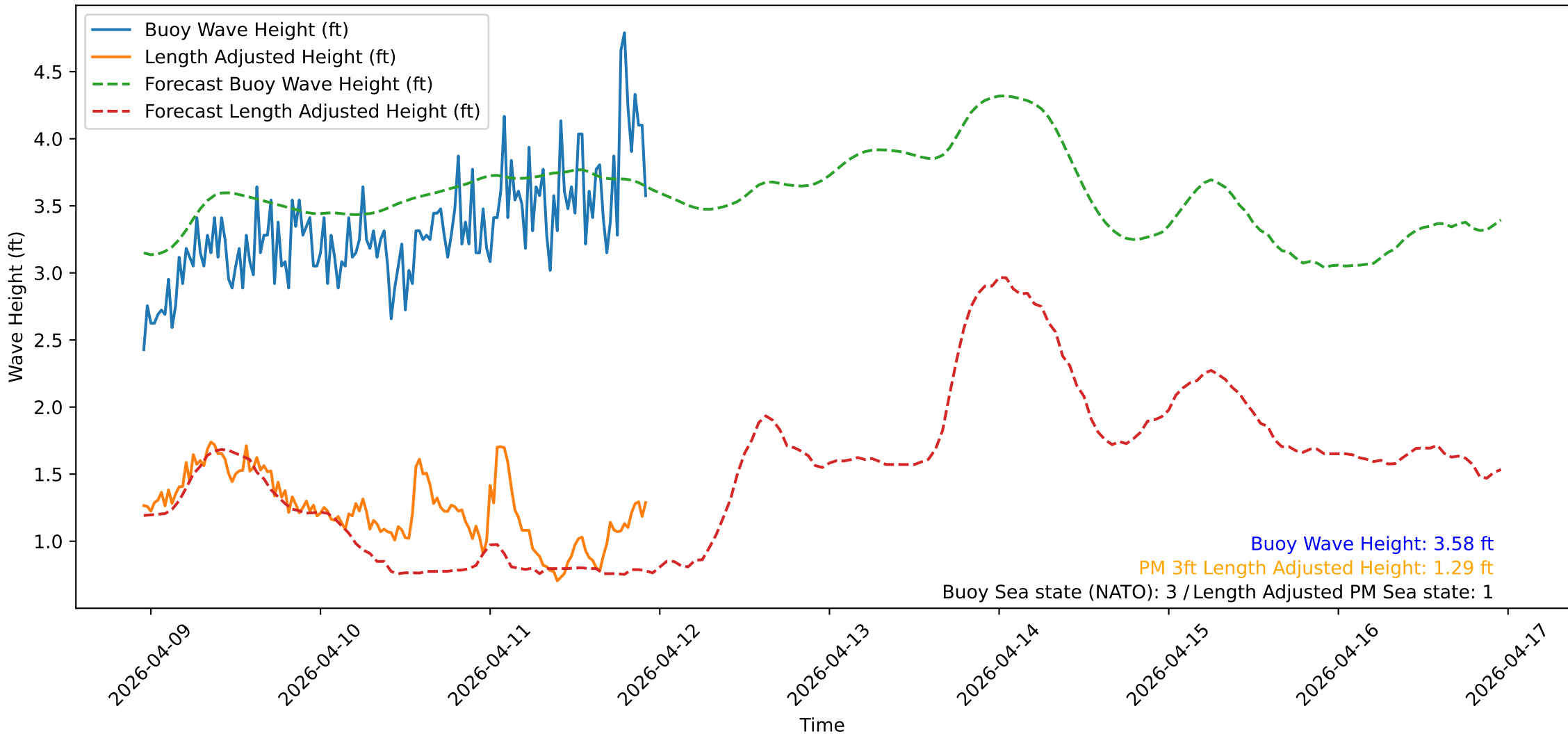
Wave Heights over Time for Oceanside Harbor at 2026-04-11 22:50:31
