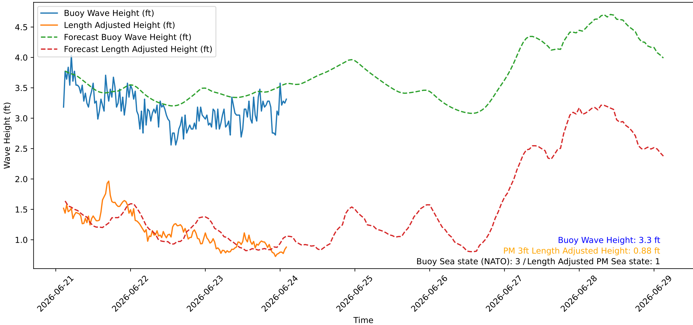
Wave Heights over Time for Oceanside Harbor at 2026-06-24 02:40:26
