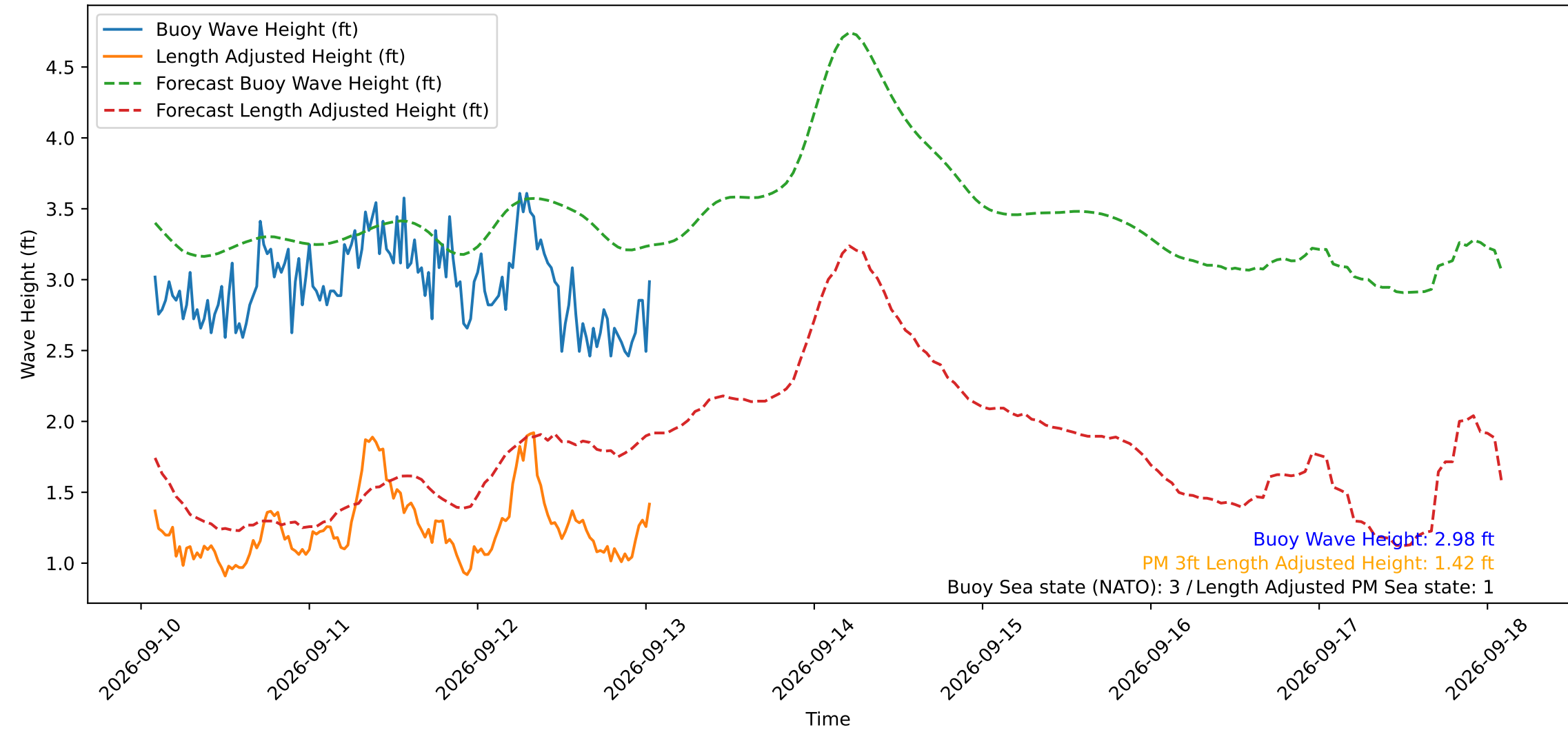
Wave Heights over Time for Green Beach at 2026-09-13 01:31:11
