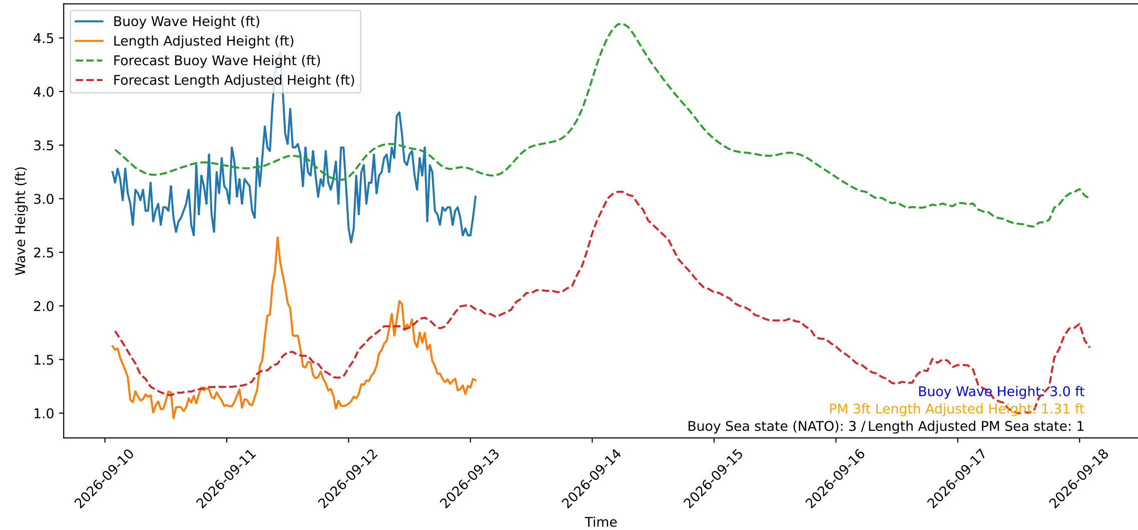
Wave Heights over Time for Oceanside Harbor at 2026-09-13 01:30:30
