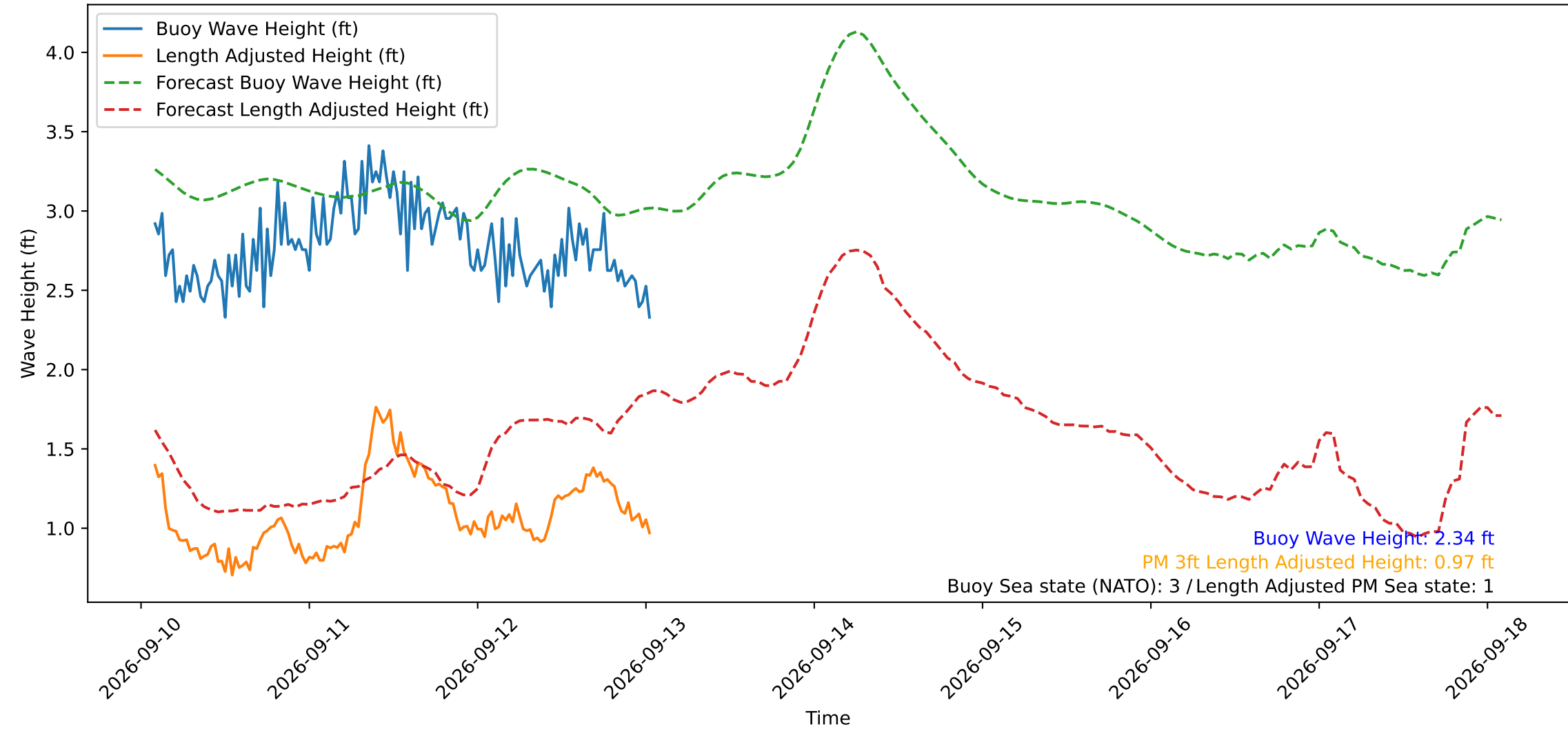
Wave Heights over Time for Red Beach at 2026-09-13 01:30:49
