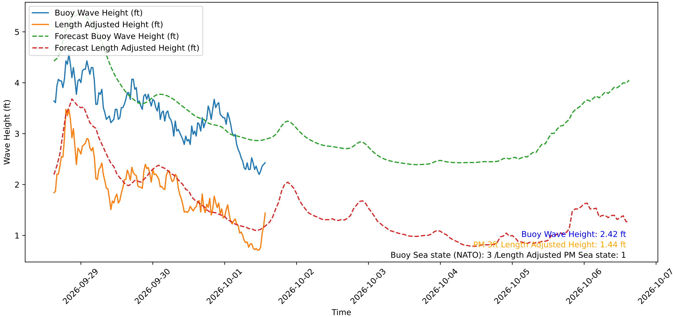
Wave Heights over Time for Green Beach at 2026-10-01 14:31:12
