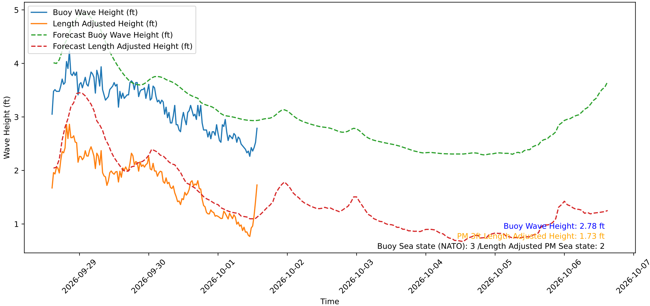
Wave Heights over Time for Oceanside Harbor at 2026-10-01 14:30:30
