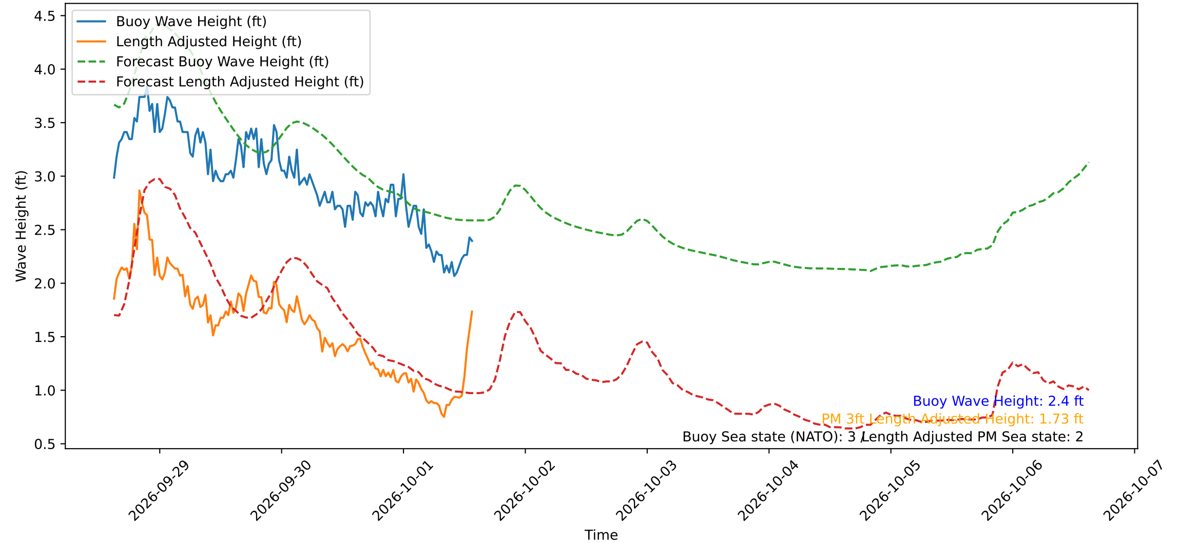
Wave Heights over Time for Red Beach at 2026-10-01 14:30:50
