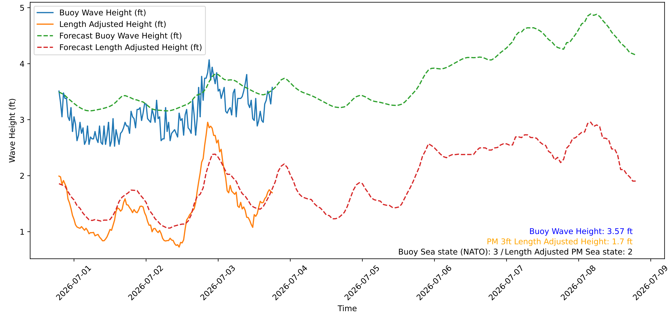
Wave Heights over Time for Green Beach at 2026-07-03 19:01:08
