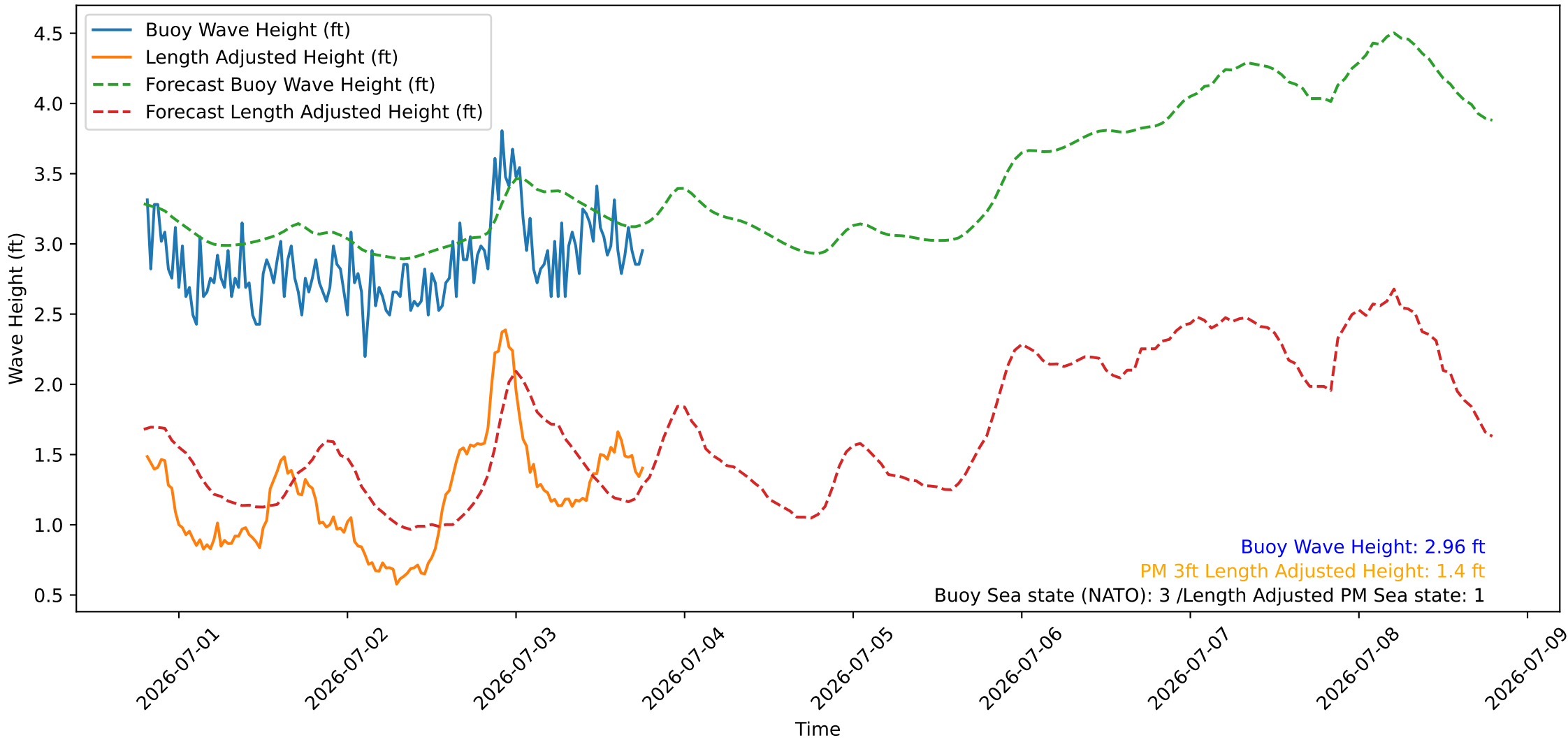
Wave Heights over Time for Red Beach at 2026-07-03 19:00:46
