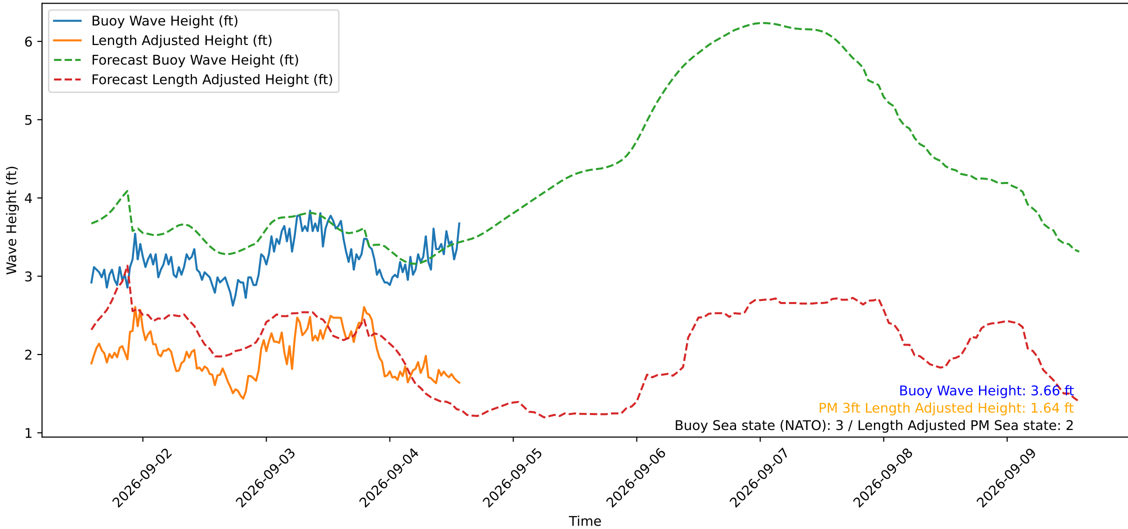
Wave Heights over Time for Oceanside Harbor at 2026-09-04 14:10:30
