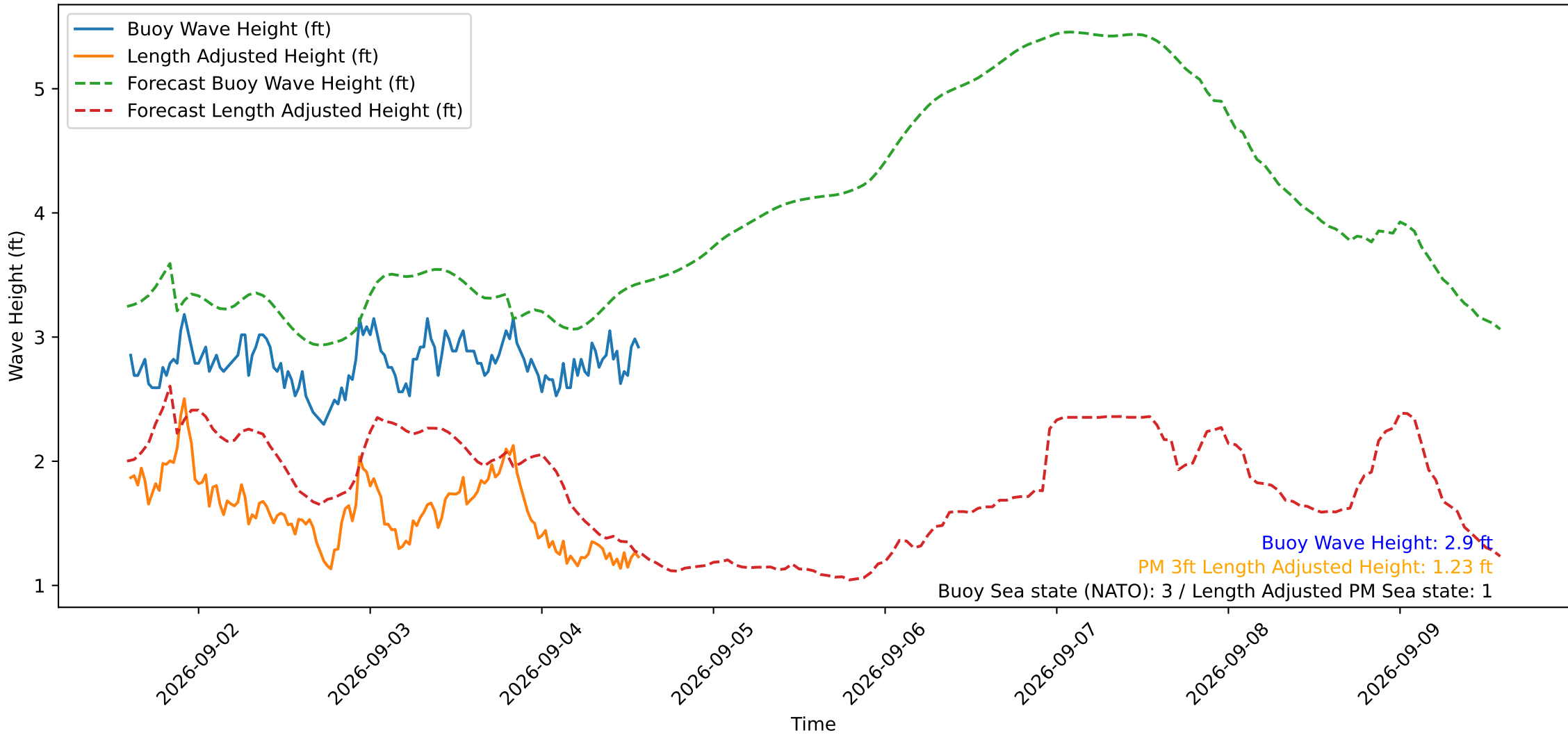
Wave Heights over Time for Red Beach at 2026-09-04 14:10:50
