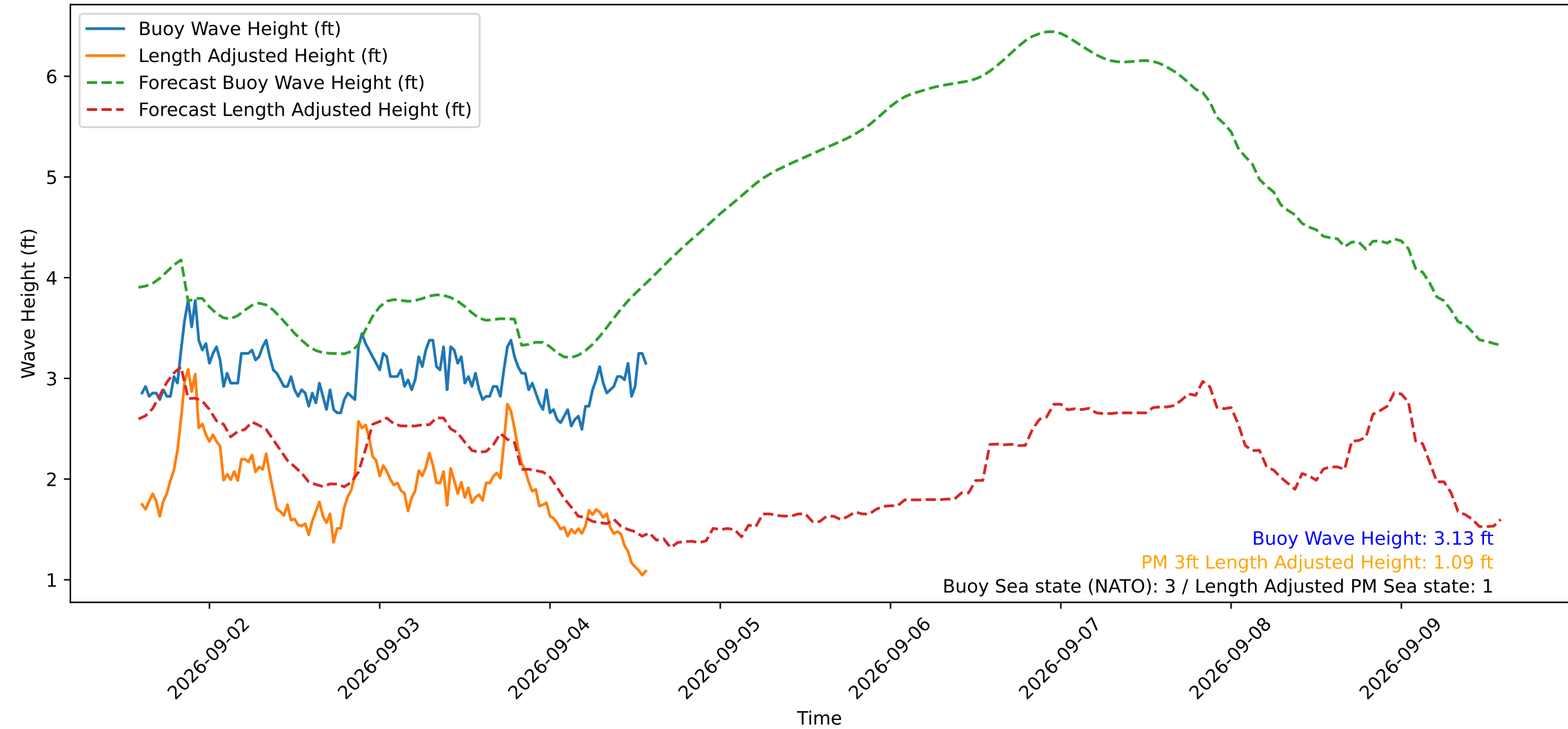
Wave Heights over Time for Green Beach at 2026-09-04 14:11:13
