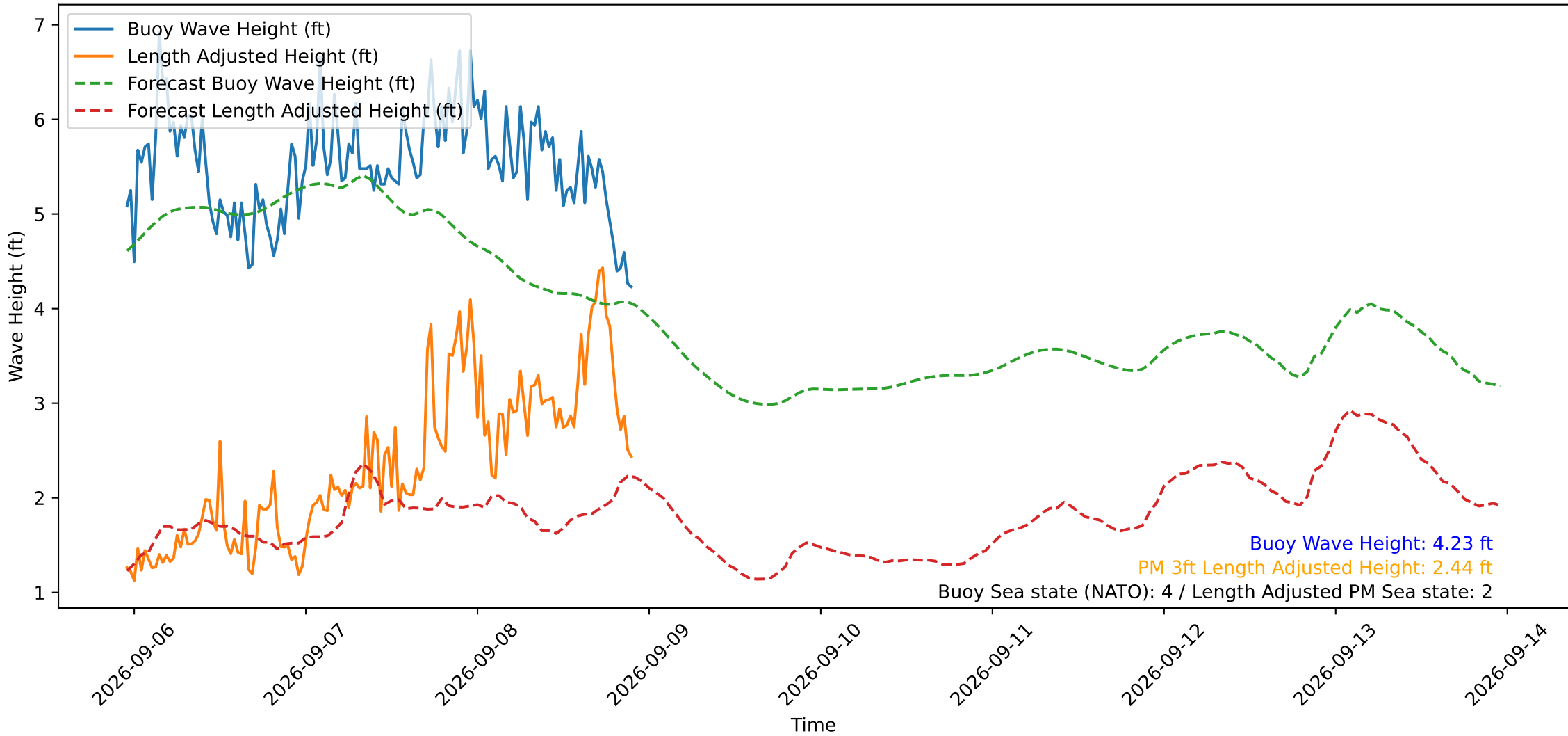
Wave Heights over Time for Red Beach at 2026-09-08 22:40:49
