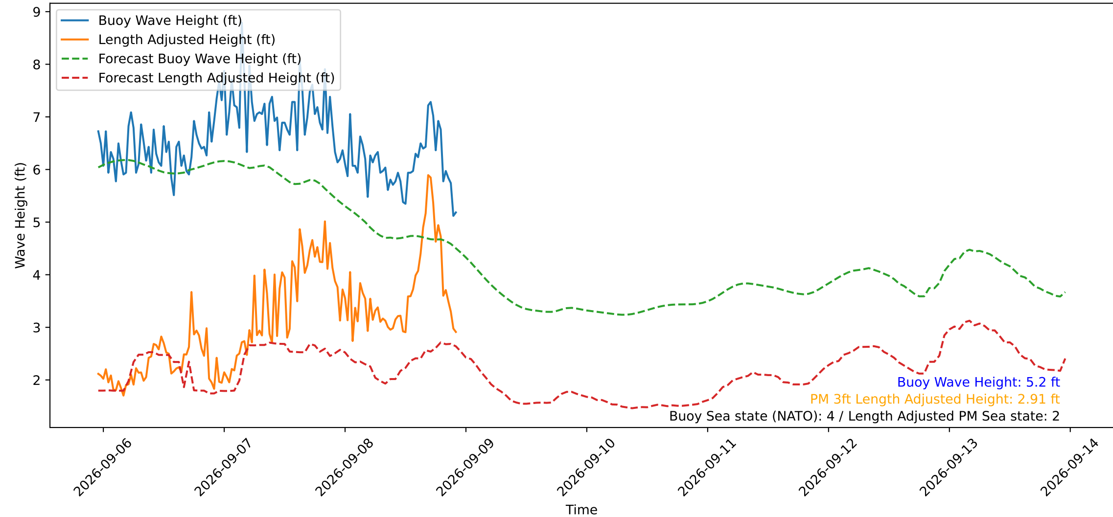
Wave Heights over Time for Green Beach at 2026-09-08 22:41:12
