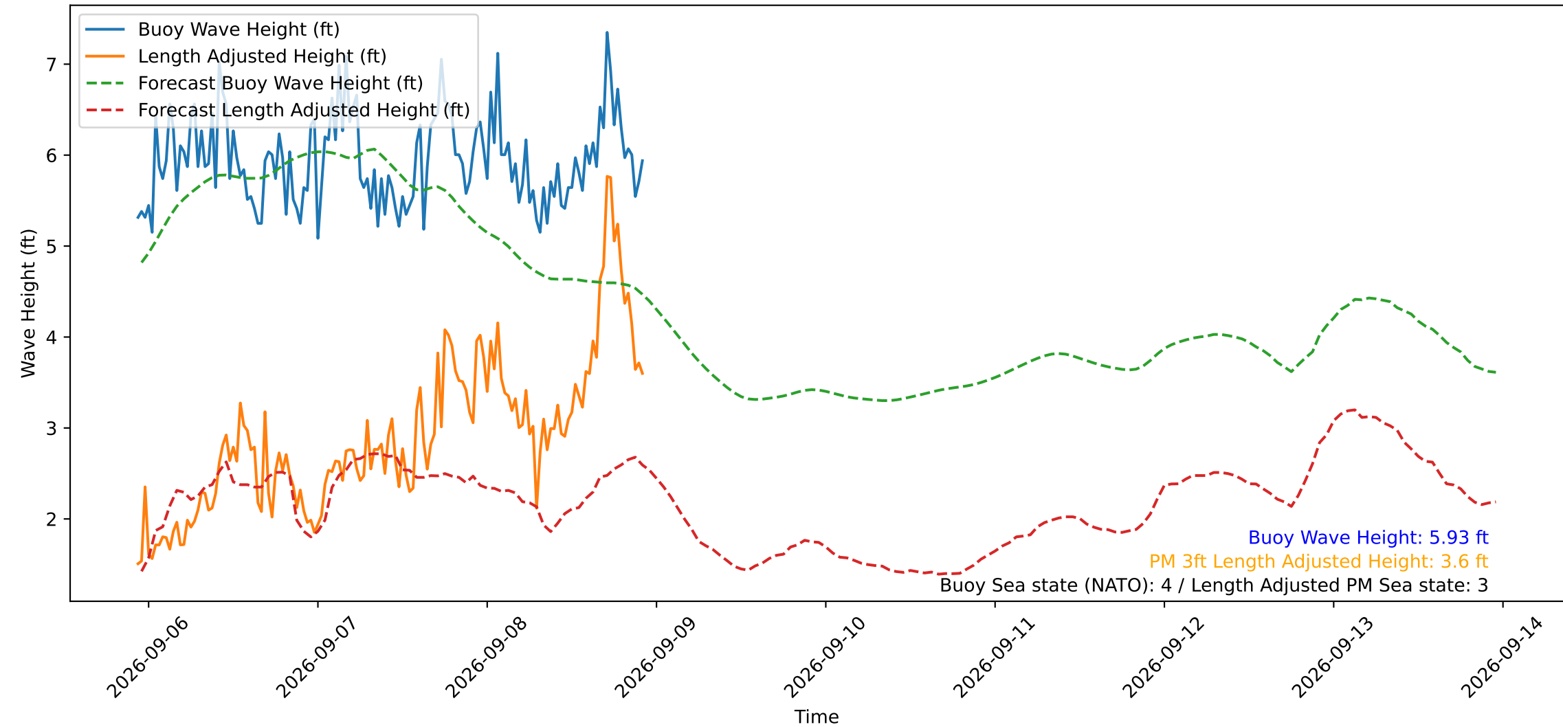
Wave Heights over Time for Oceanside Harbor at 2026-09-08 22:40:29
