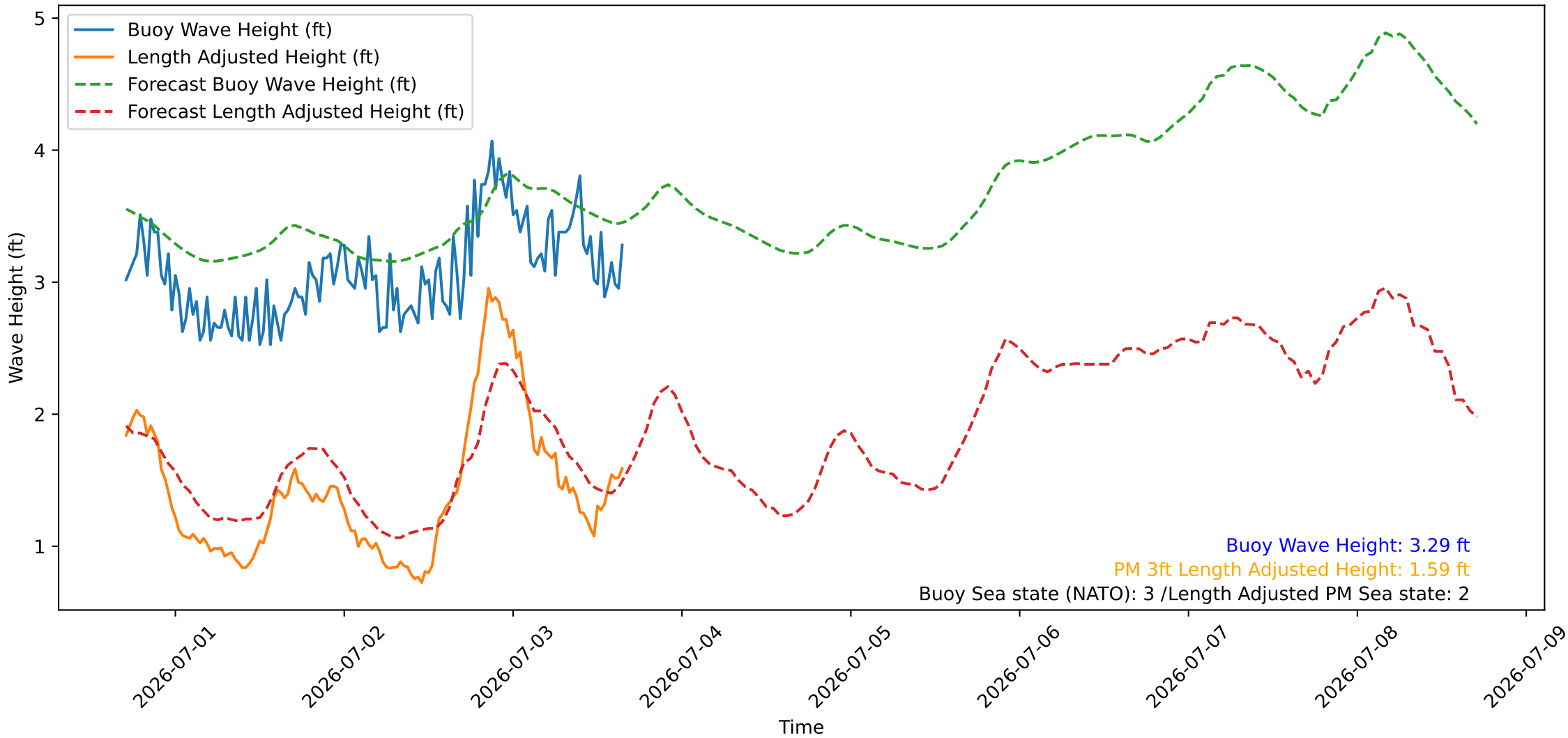
Wave Heights over Time for Green Beach at 2026-07-03 17:01:09
