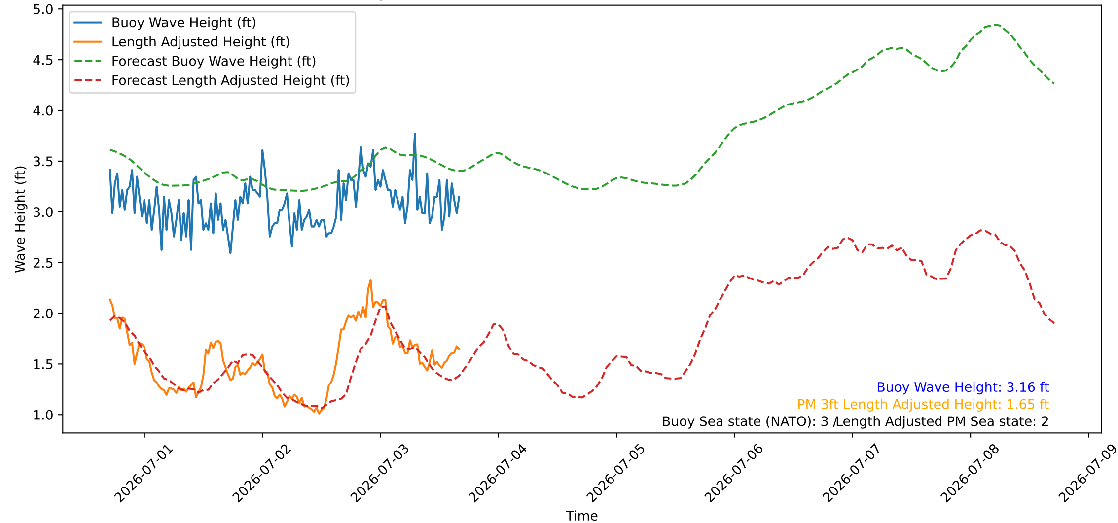
Wave Heights over Time for Oceanside Harbor at 2026-07-03 17:00:26
