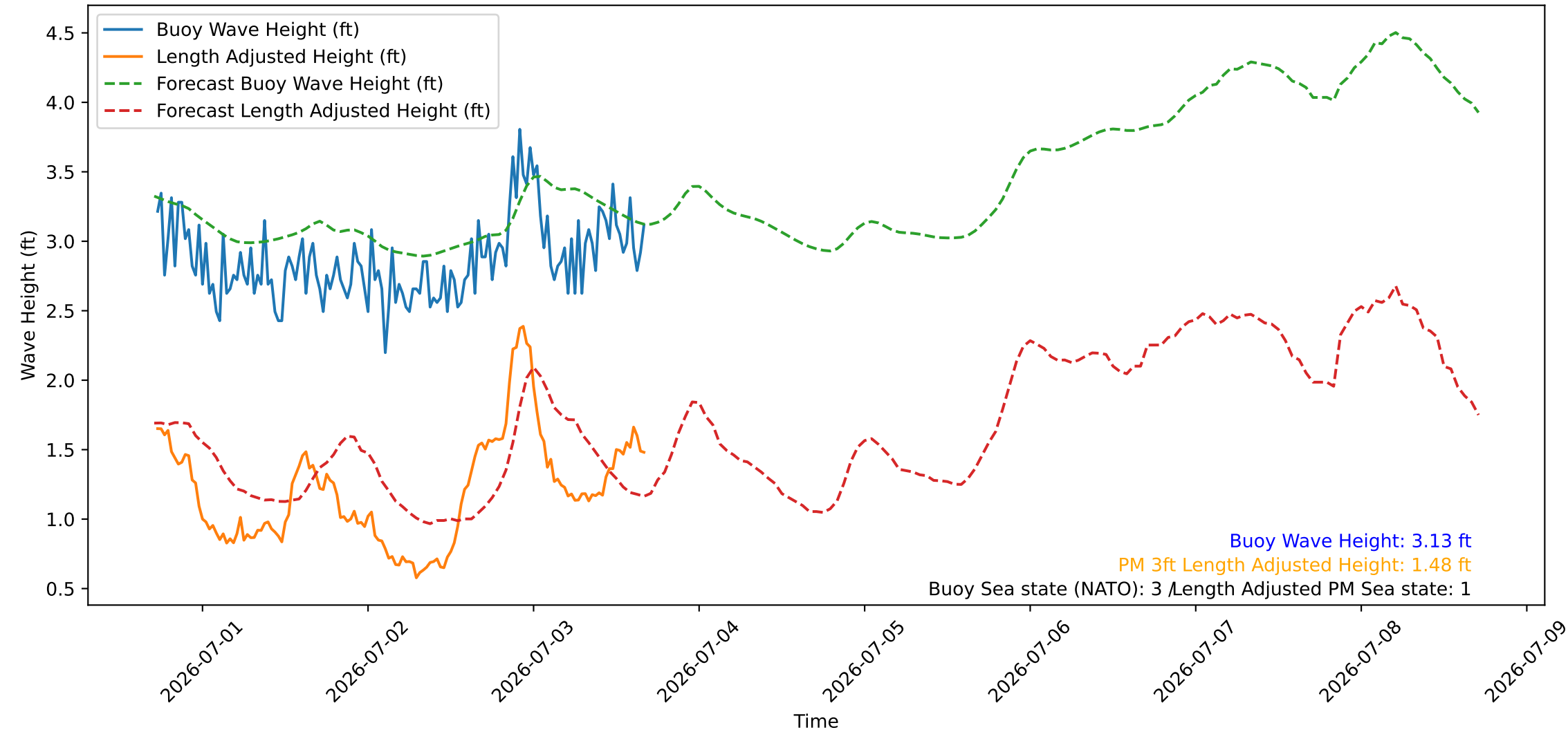
Wave Heights over Time for Red Beach at 2026-07-03 17:00:46
