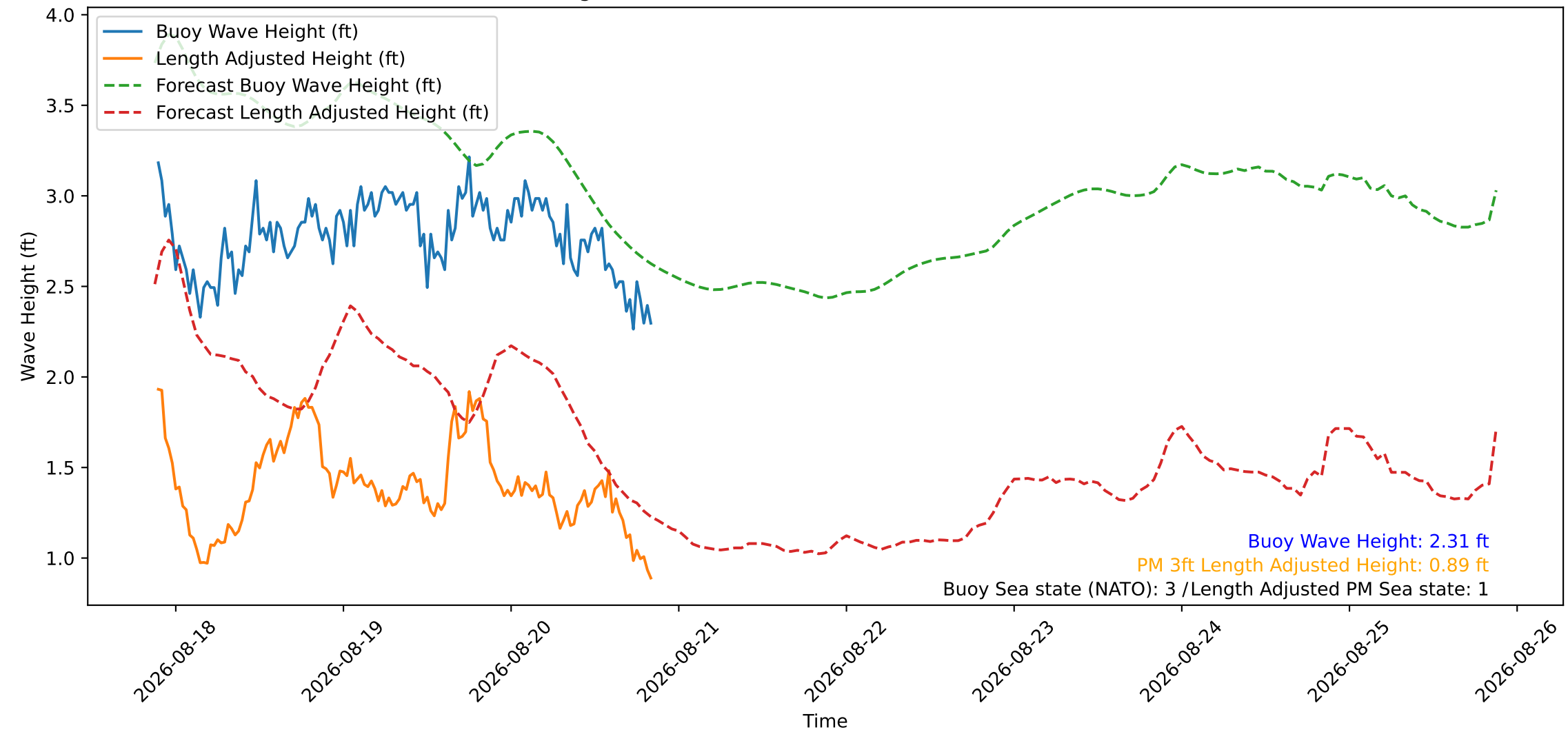
Wave Heights over Time for Red Beach at 2026-08-20 21:00:46
