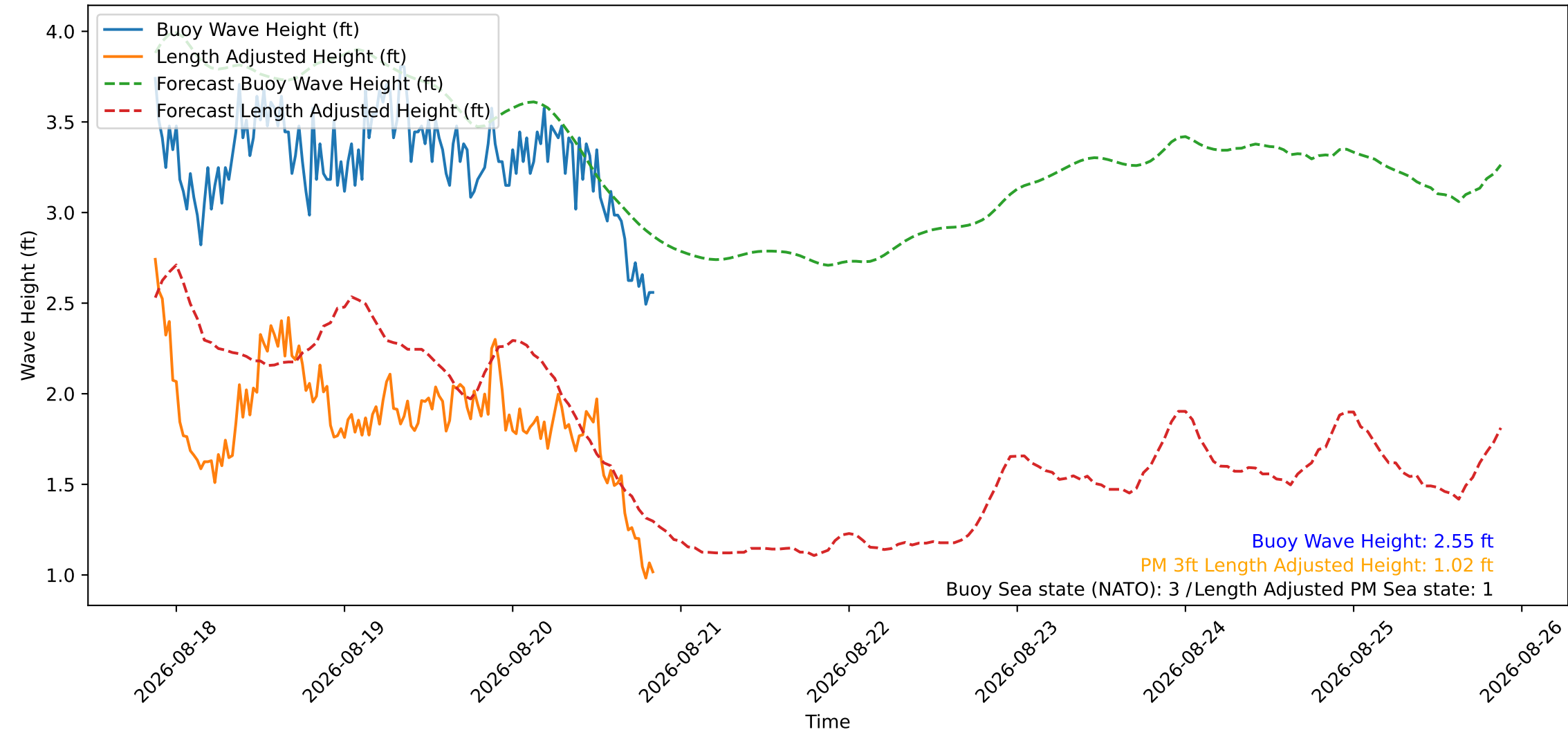
Wave Heights over Time for Oceanside Harbor at 2026-08-20 21:00:27
