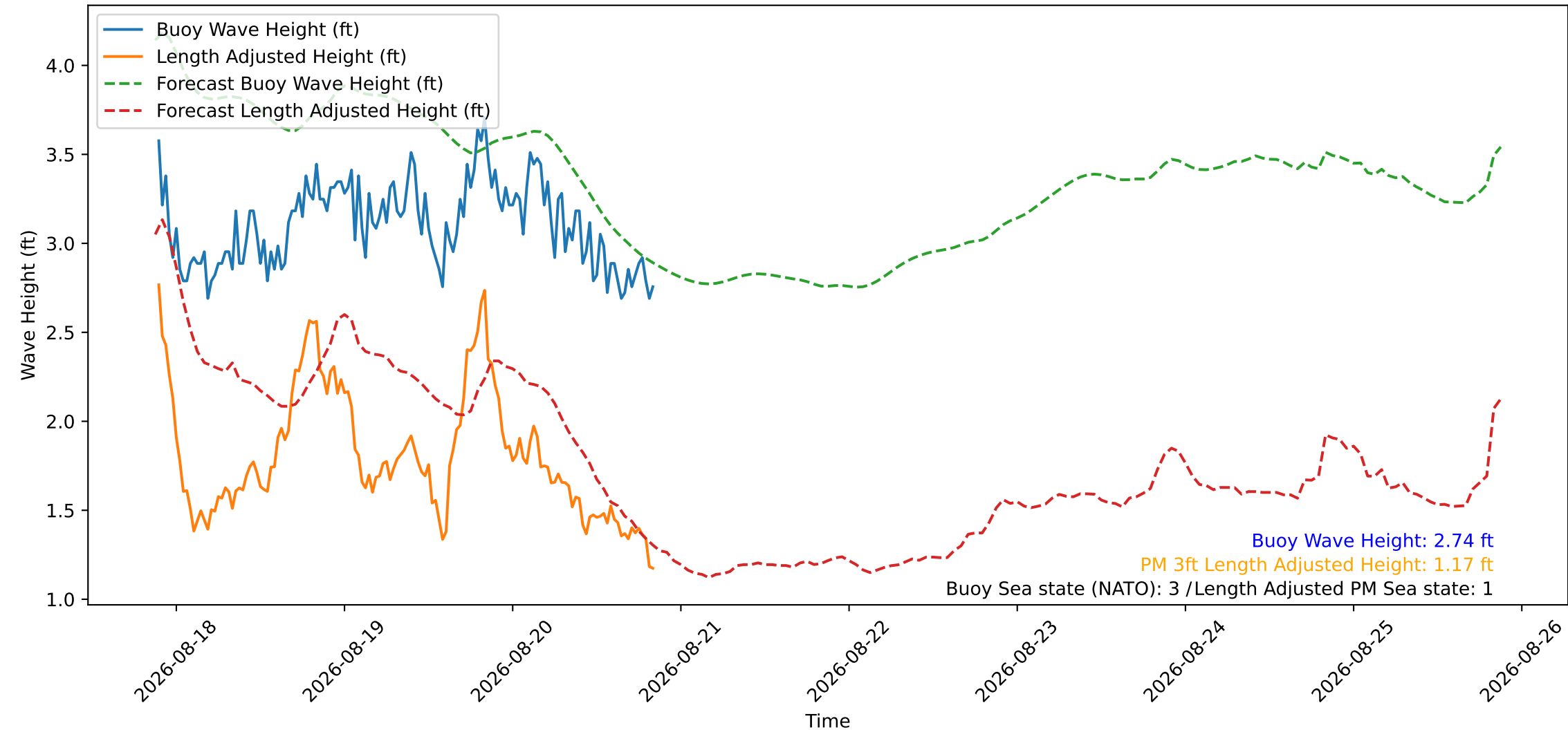
Wave Heights over Time for Green Beach at 2026-08-20 21:01:09
