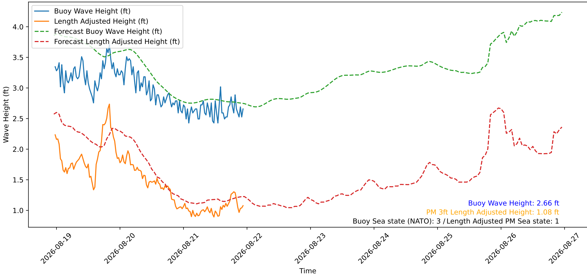
Wave Heights over Time for Green Beach at 2026-08-21 23:21:15
