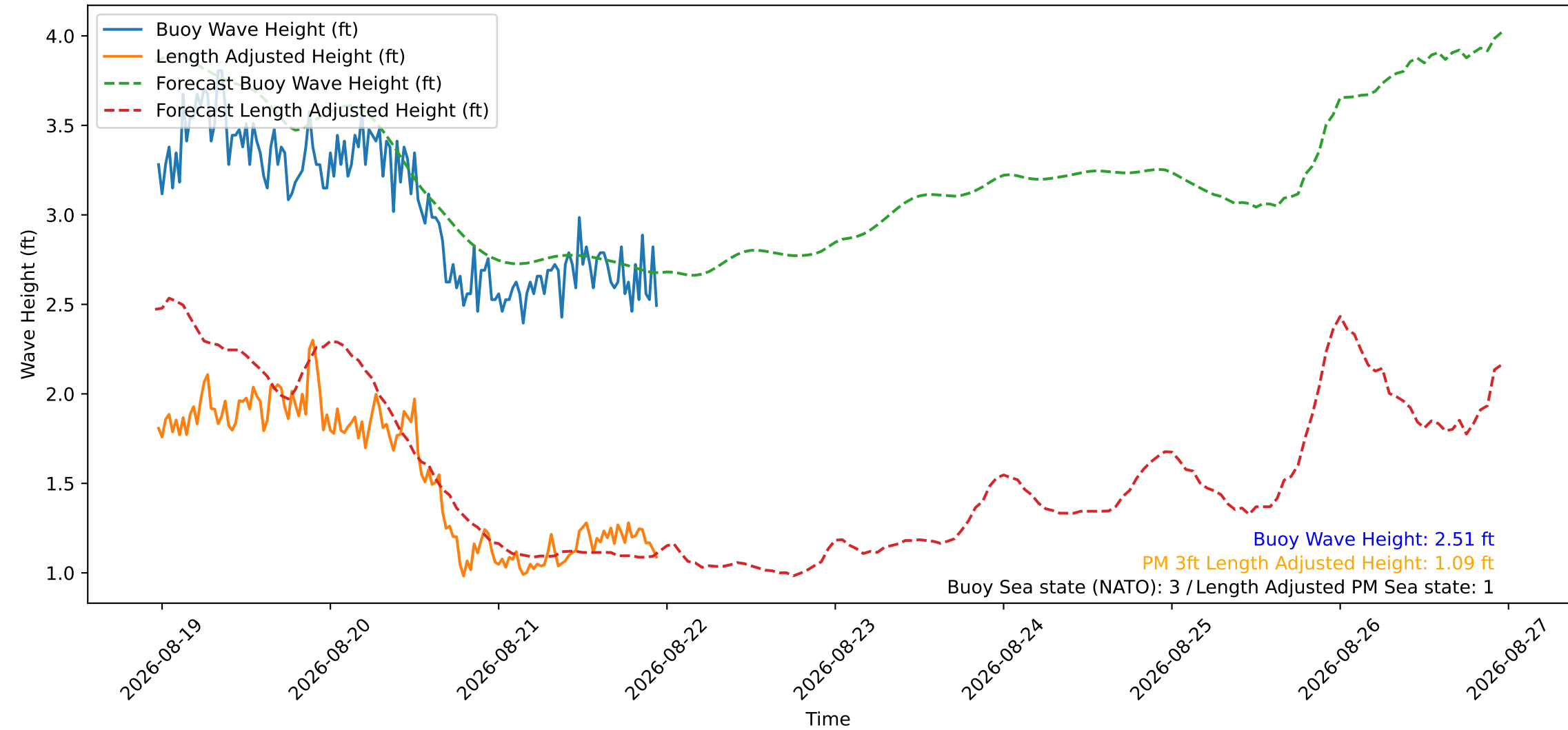
Wave Heights over Time for Oceanside Harbor at 2026-08-21 23:20:30
