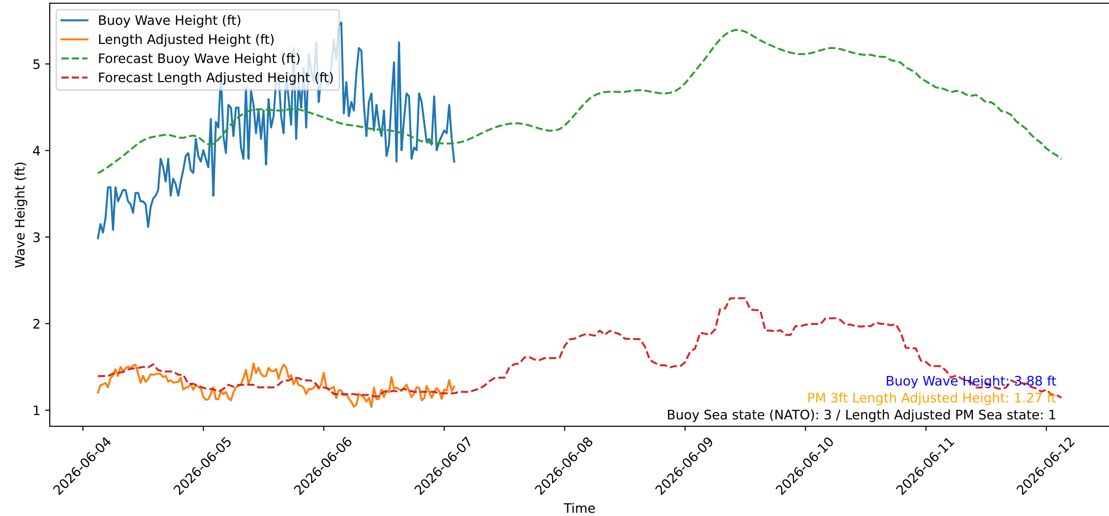
Wave Heights over Time for Oceanside Harbor at 2026-06-07 03:00:26
