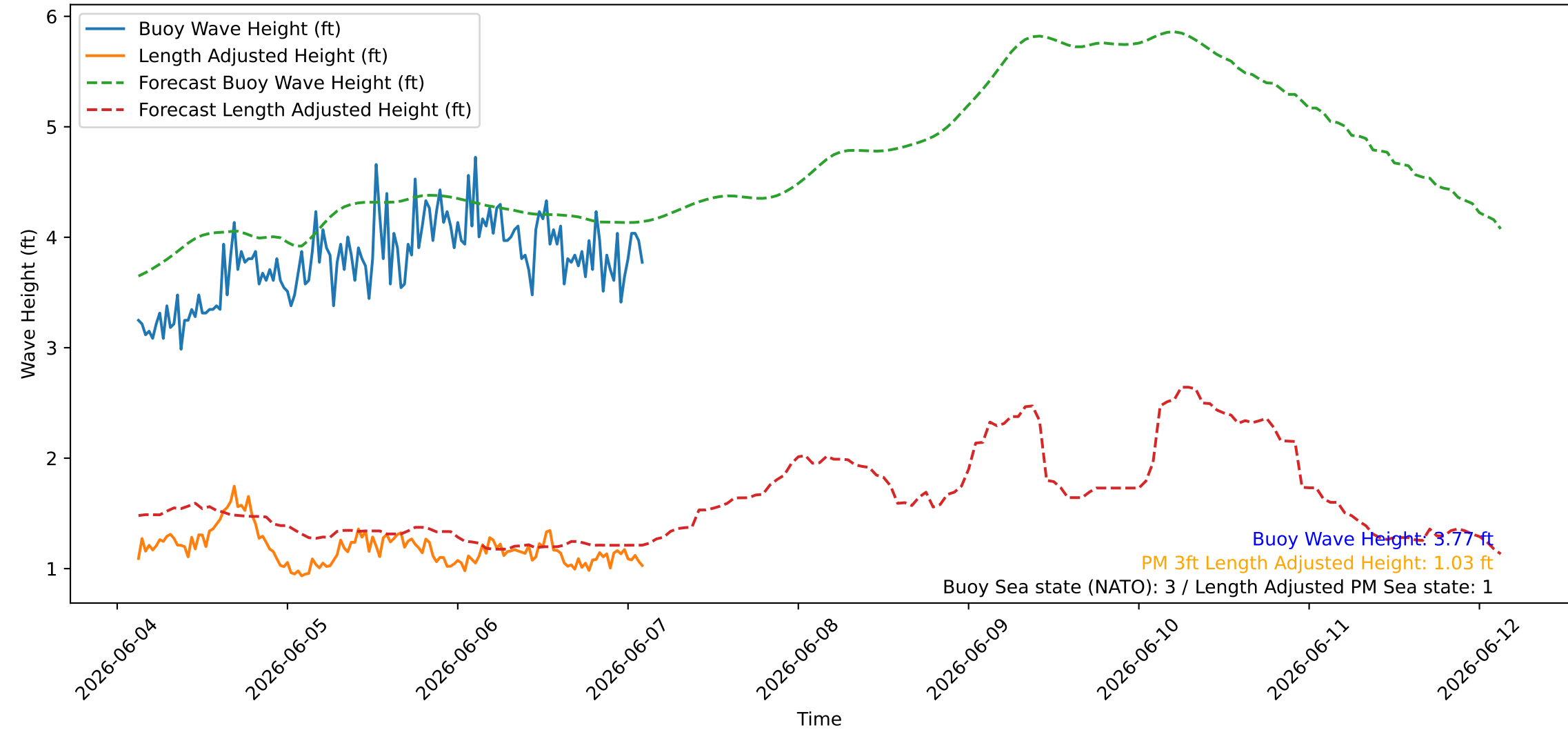
Wave Heights over Time for Green Beach at 2026-06-07 03:01:07
