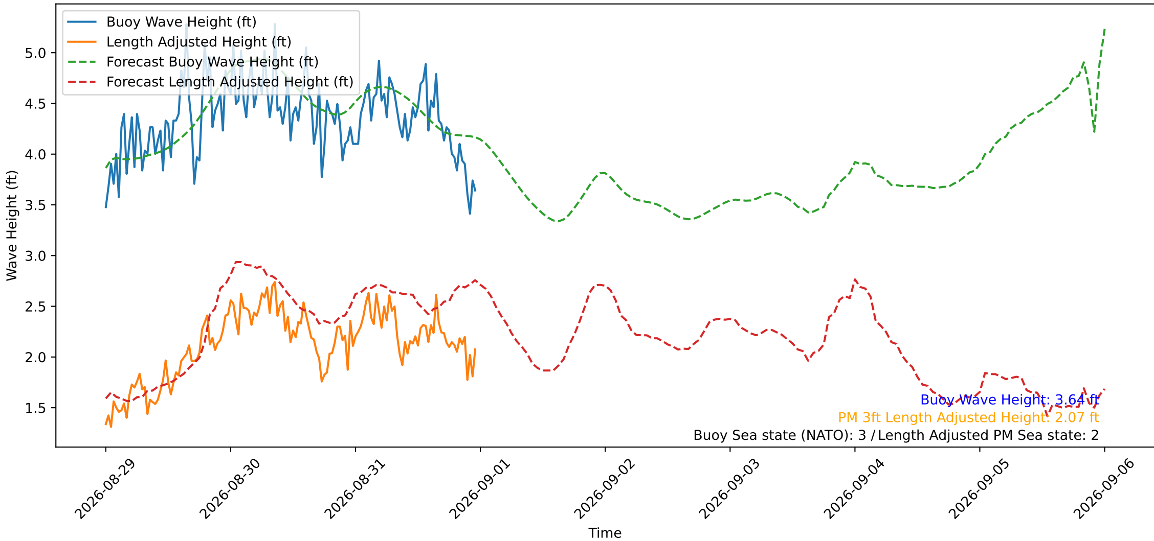
Wave Heights over Time for Oceanside Harbor at 2026-09-01 00:00:29
