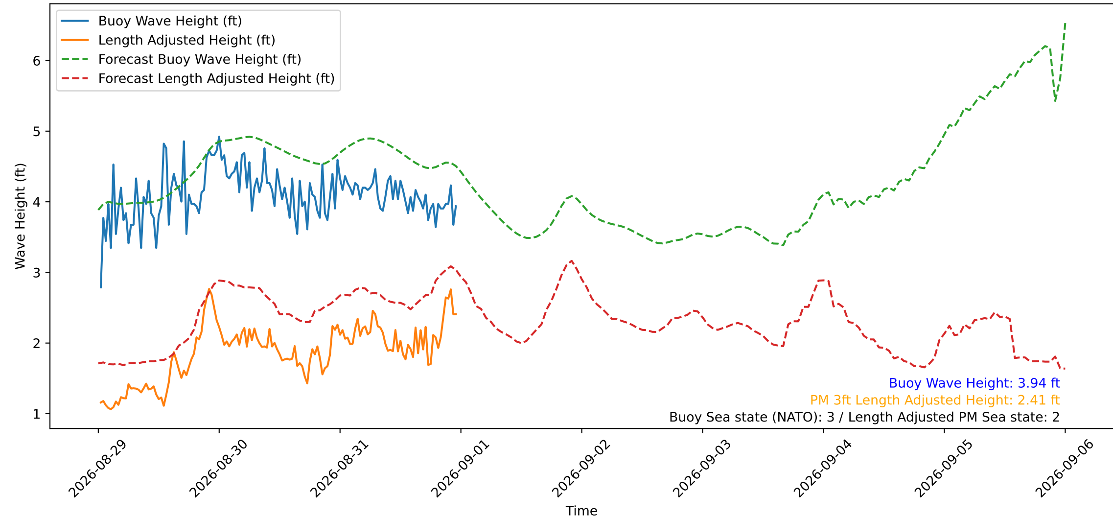
Wave Heights over Time for Green Beach at 2026-09-01 00:01:12
