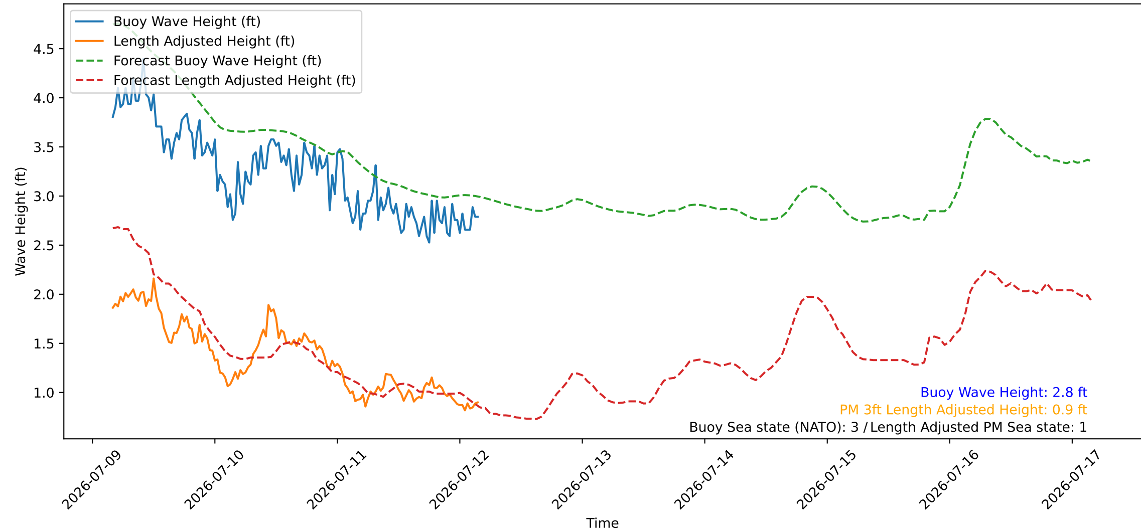
Wave Heights over Time for Green Beach at 2026-07-12 04:11:08
