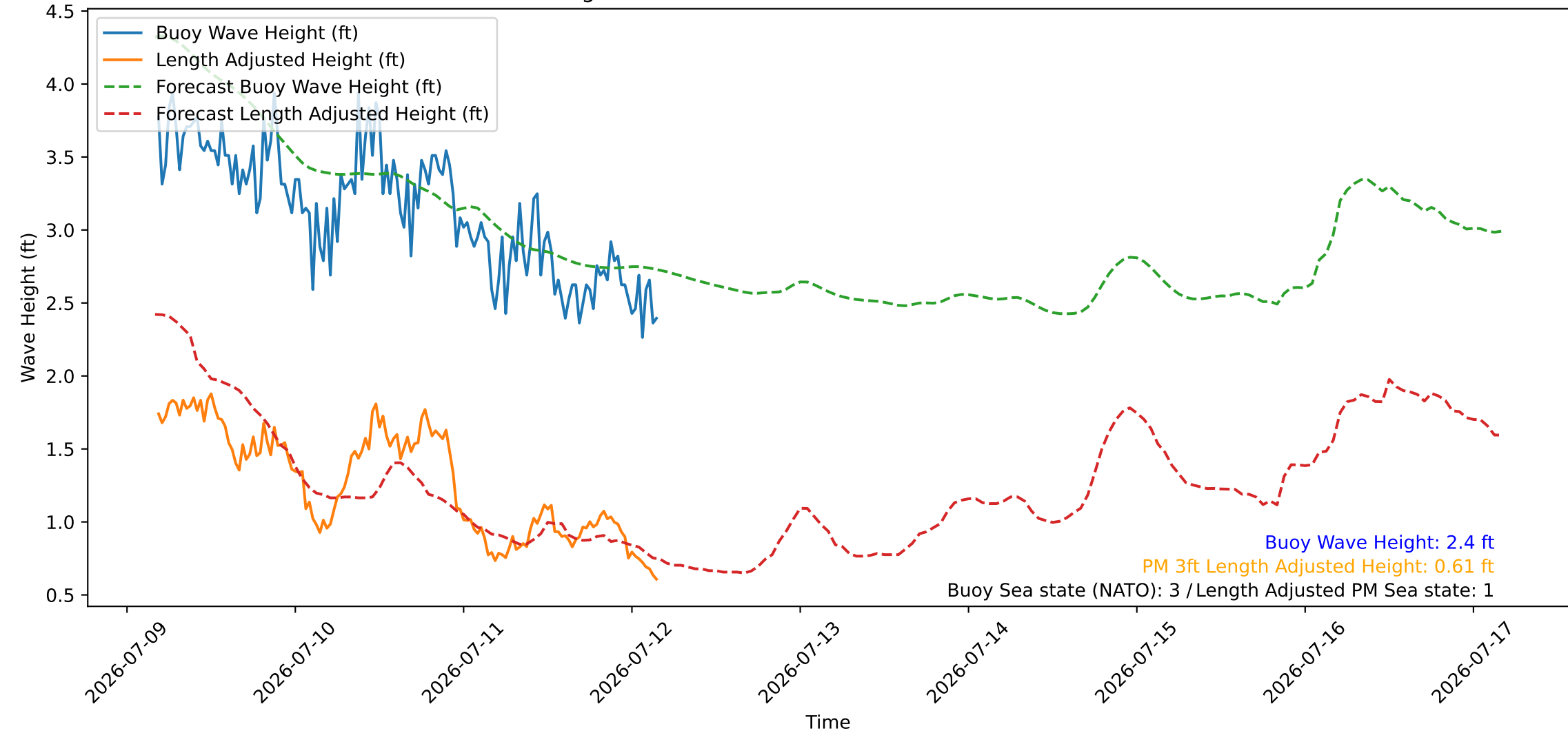
Wave Heights over Time for Red Beach at 2026-07-12 04:10:45
