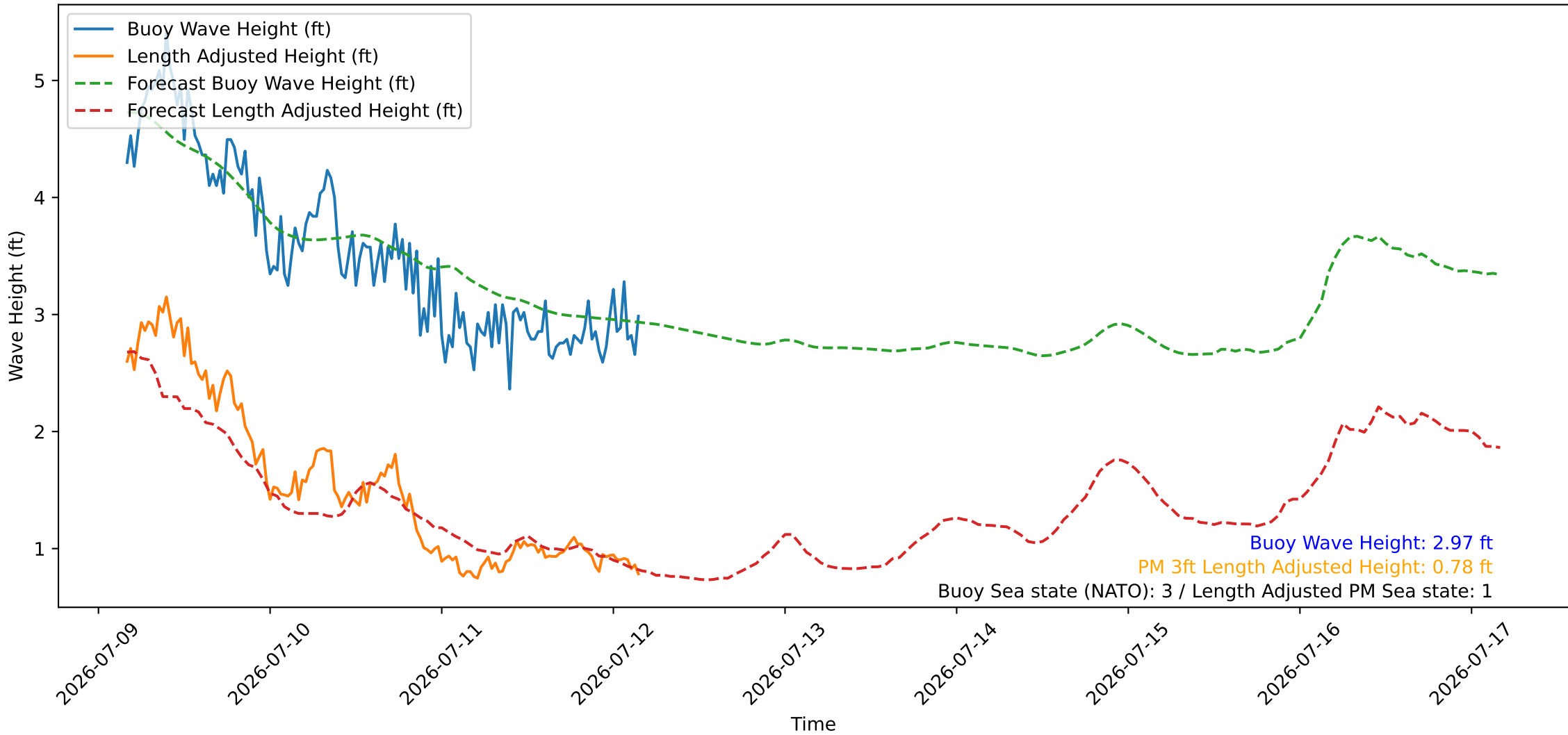
Wave Heights over Time for Oceanside Harbor at 2026-07-12 04:10:26
